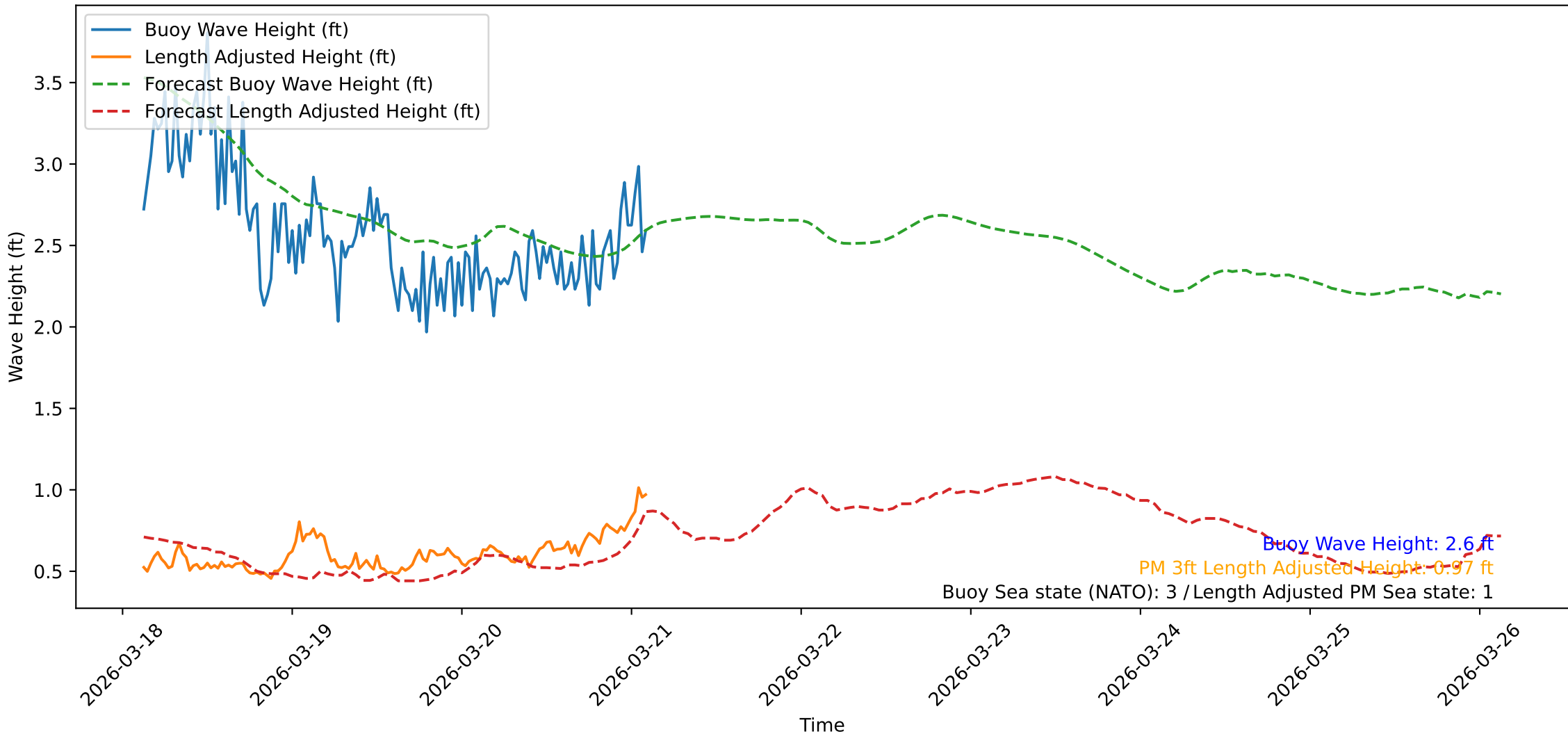
Wave Heights over Time for Oceanside Harbor at 2026-03-21 03:00:31
