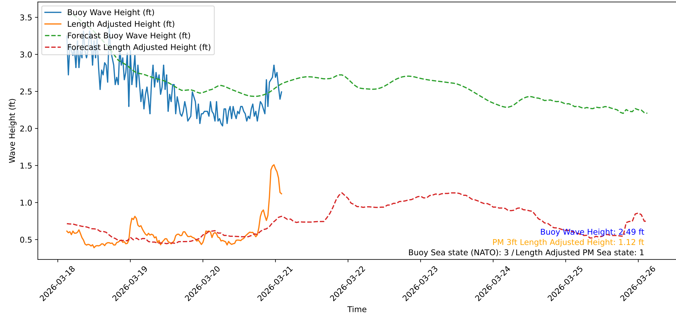
Wave Heights over Time for Green Beach at 2026-03-21 03:01:10
