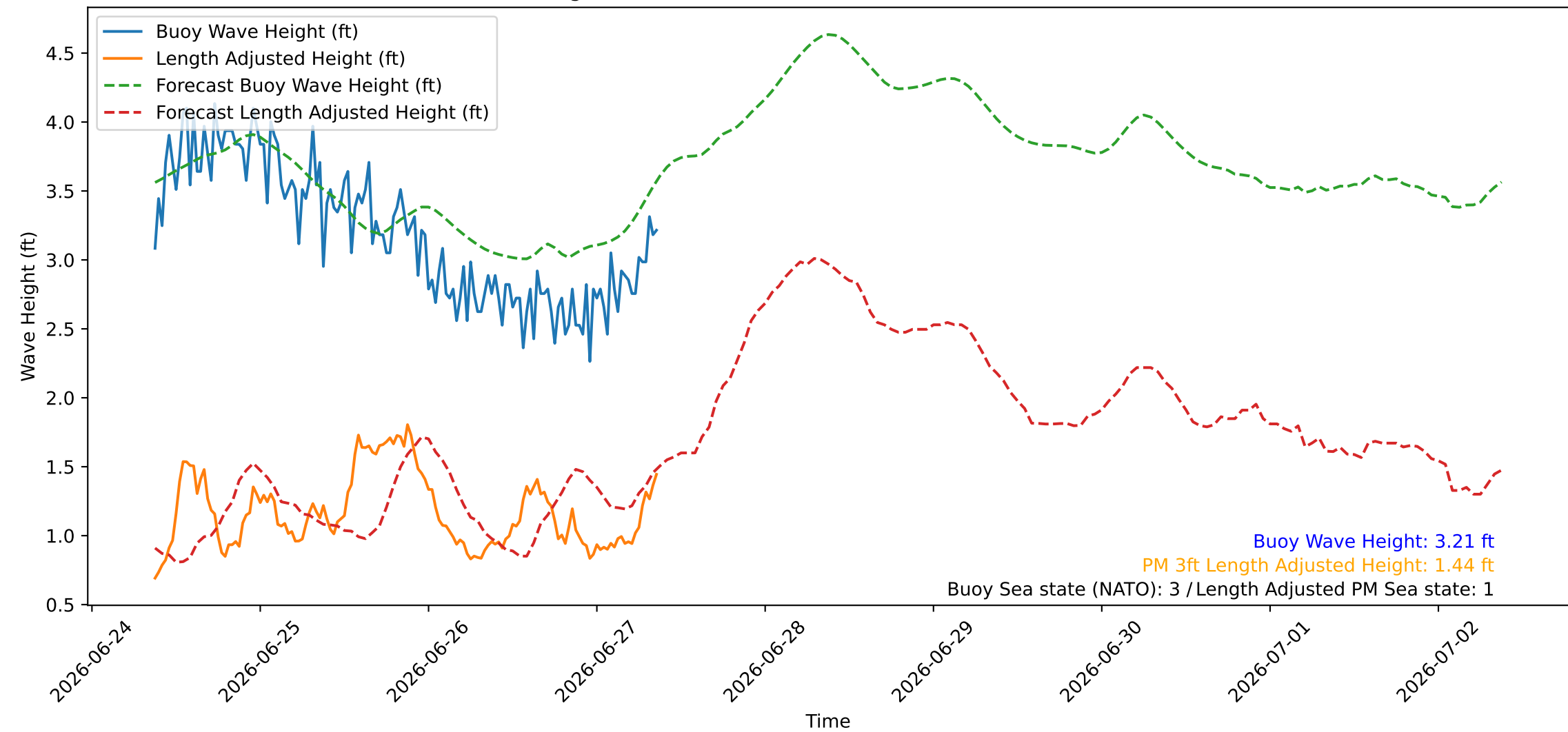
Wave Heights over Time for Green Beach at 2026-06-27 09:11:08
