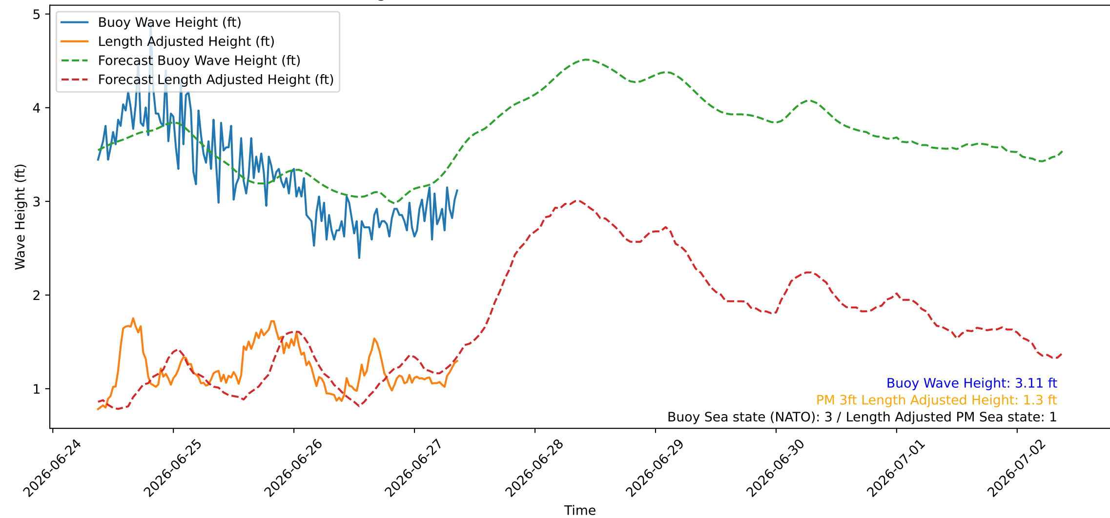
Wave Heights over Time for Oceanside Harbor at 2026-06-27 09:10:26
