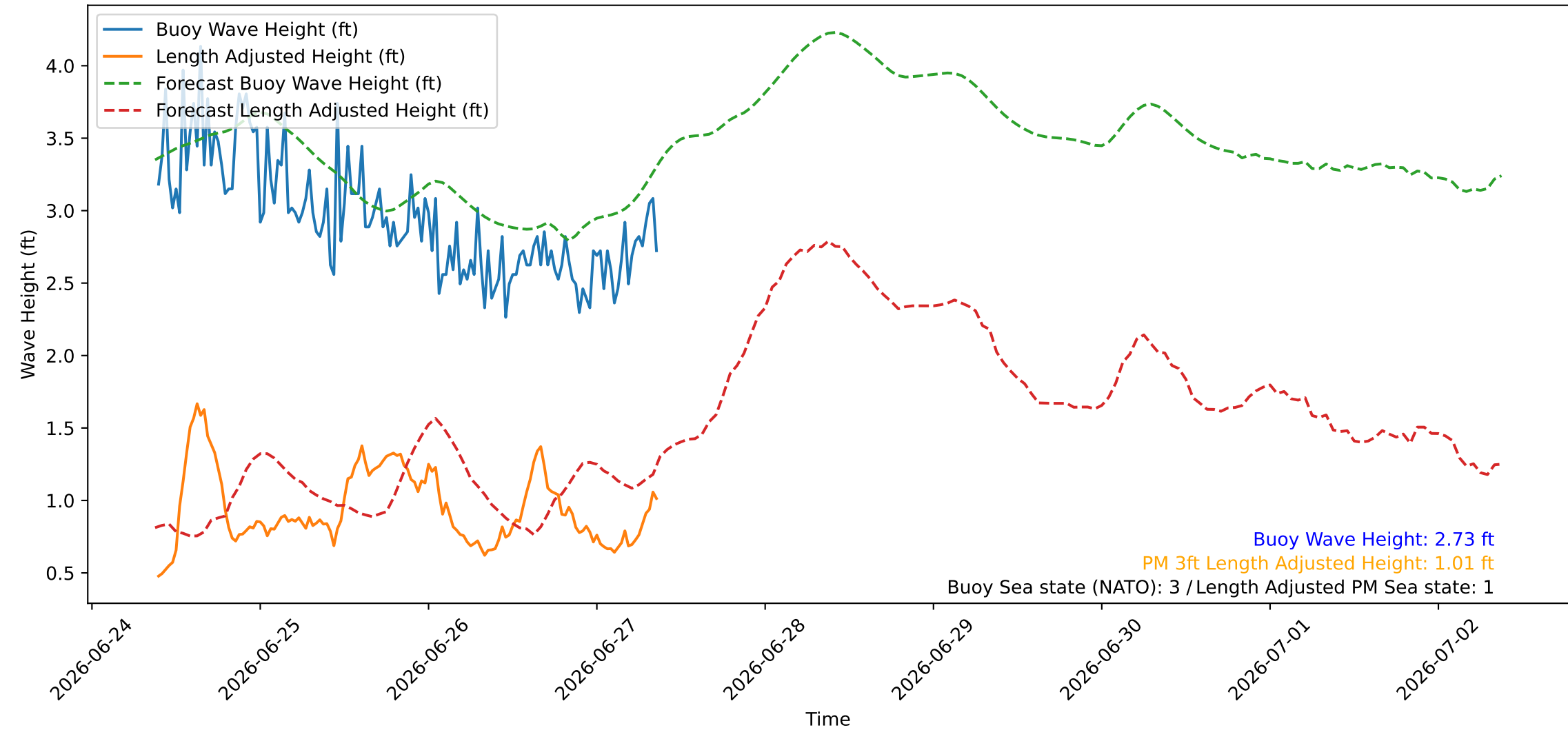
Wave Heights over Time for Red Beach at 2026-06-27 09:10:45
