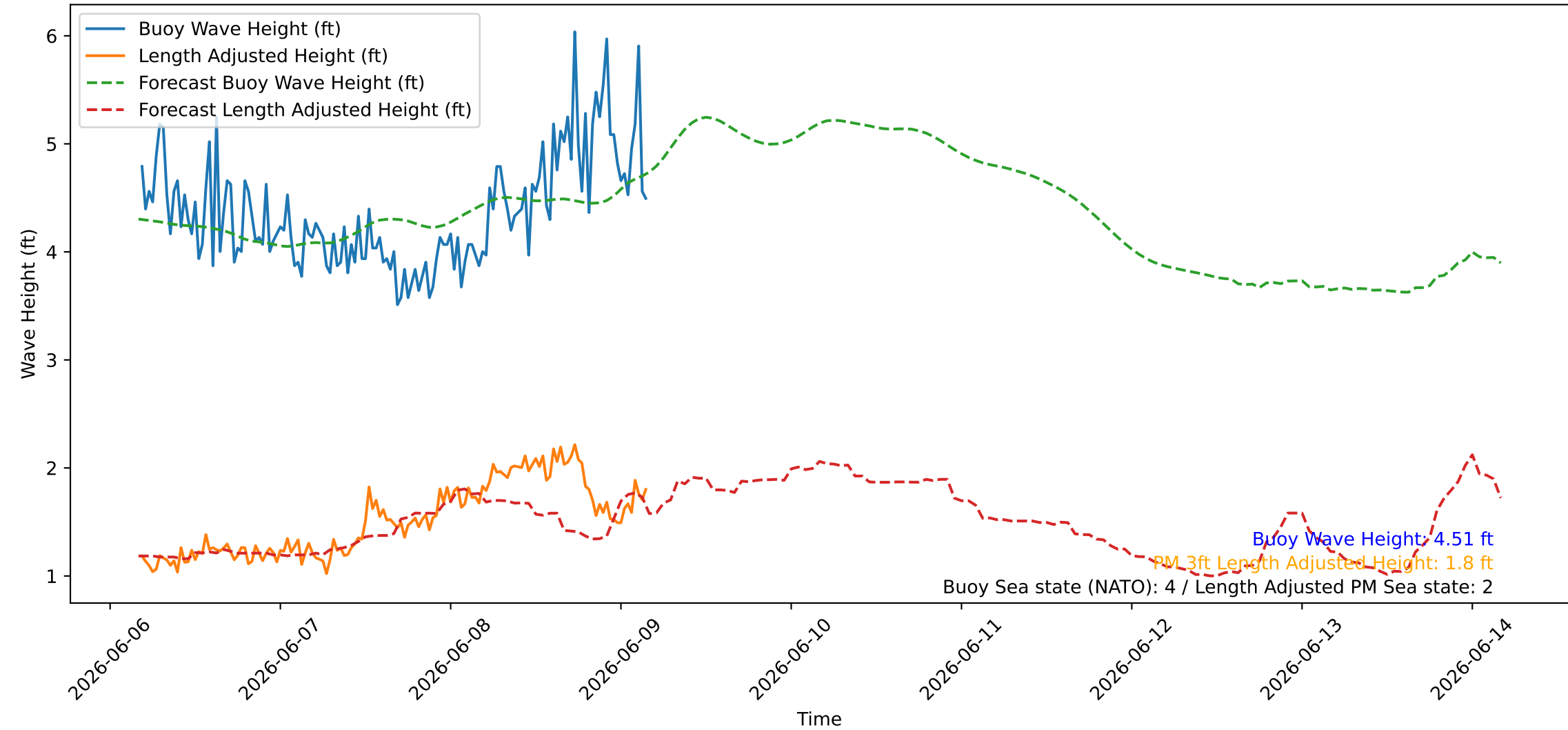
Wave Heights over Time for Oceanside Harbor at 2026-06-09 04:20:26
