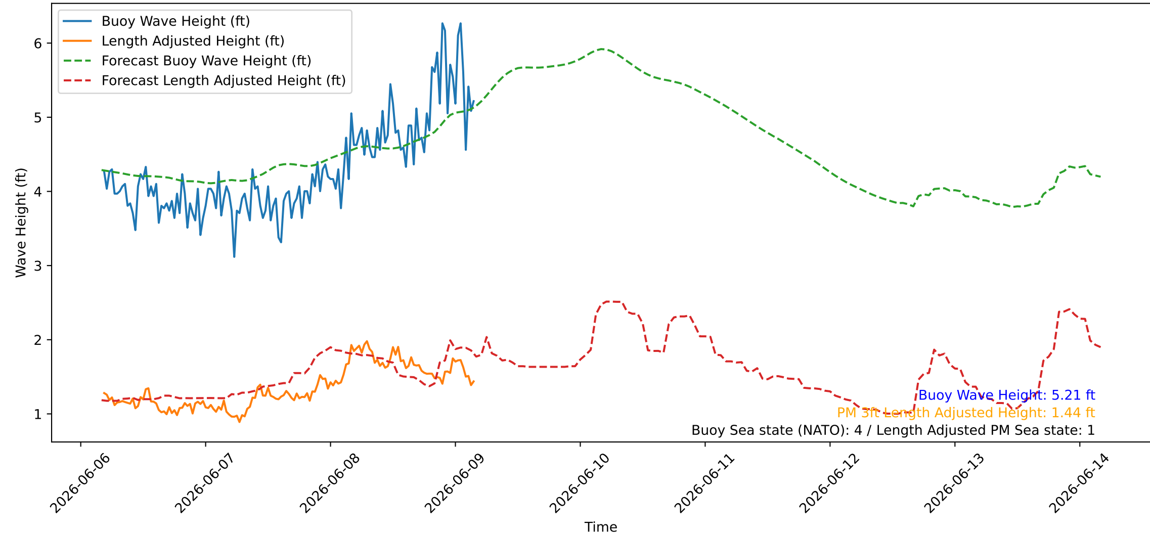
Wave Heights over Time for Green Beach at 2026-06-09 04:21:09
