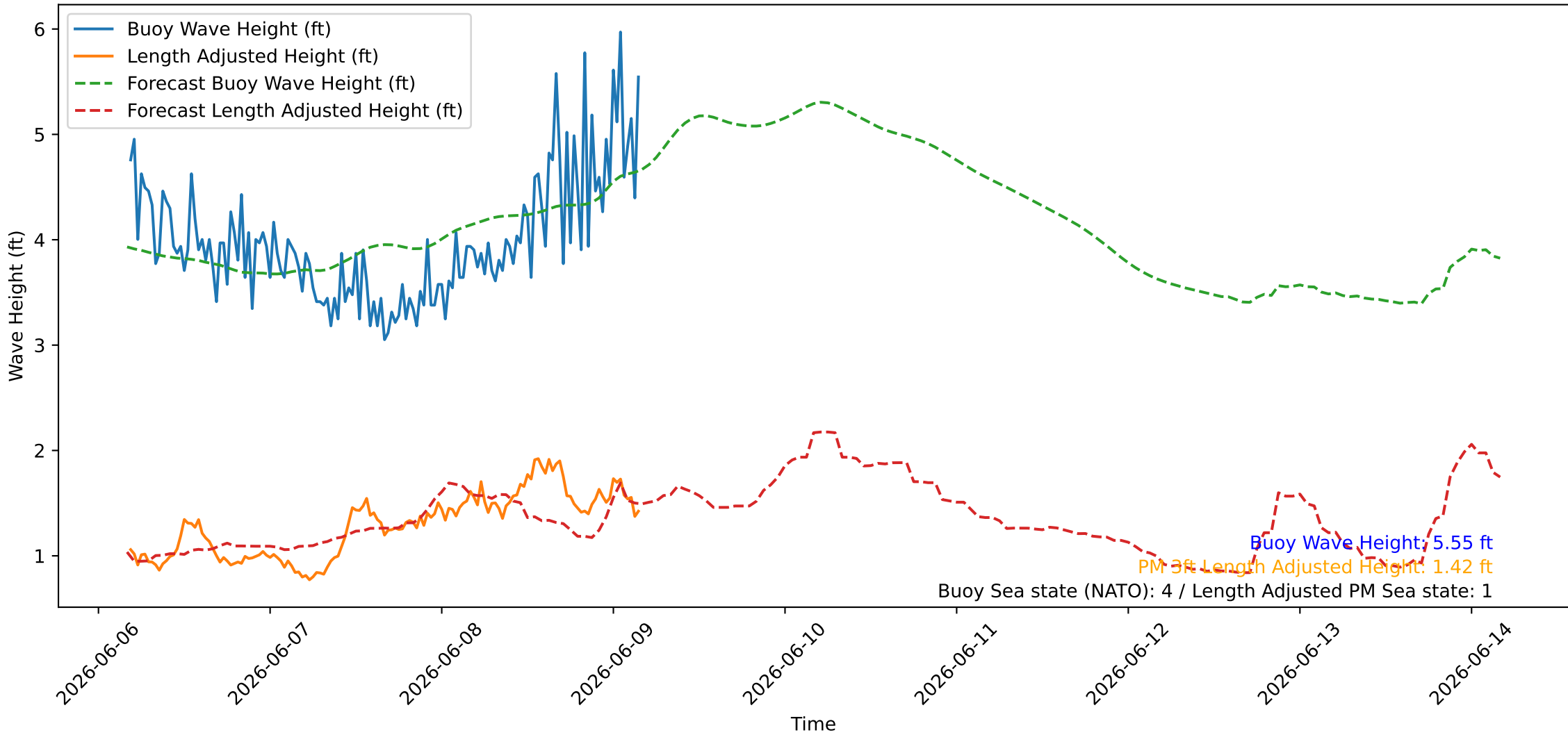
Wave Heights over Time for Red Beach at 2026-06-09 04:20:47
