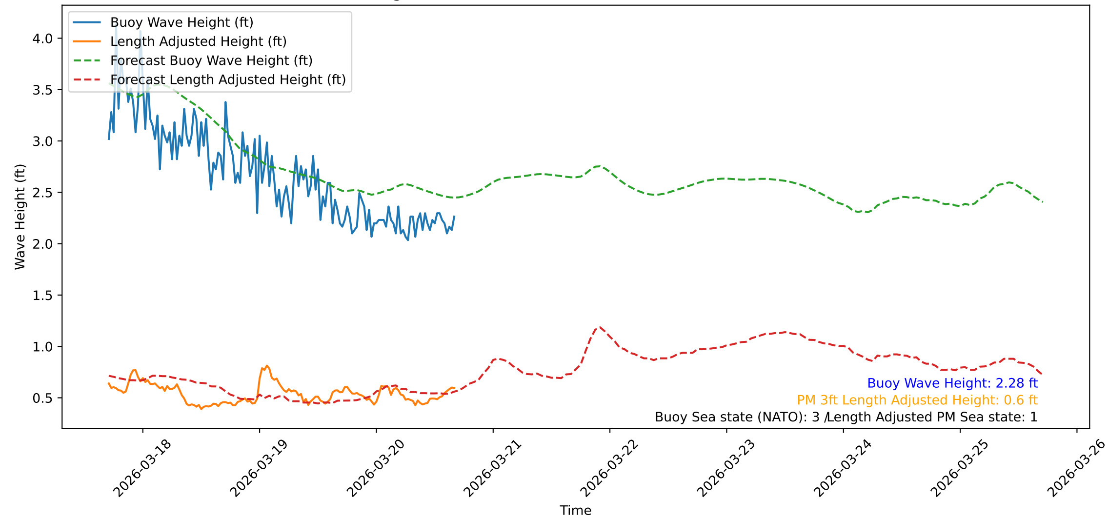
Wave Heights over Time for Green Beach at 2026-03-20 16:51:09
