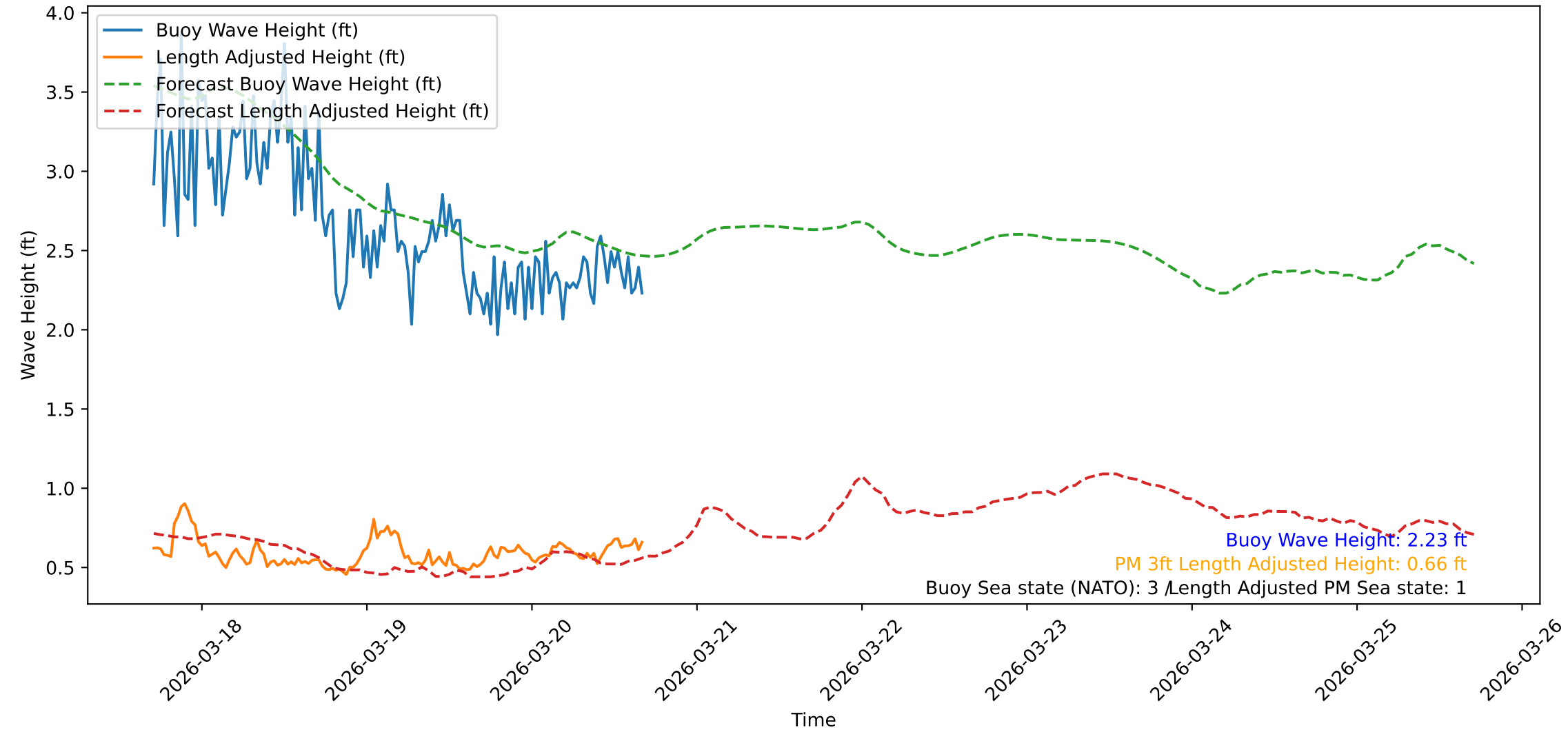
Wave Heights over Time for Oceanside Harbor at 2026-03-20 16:50:31
