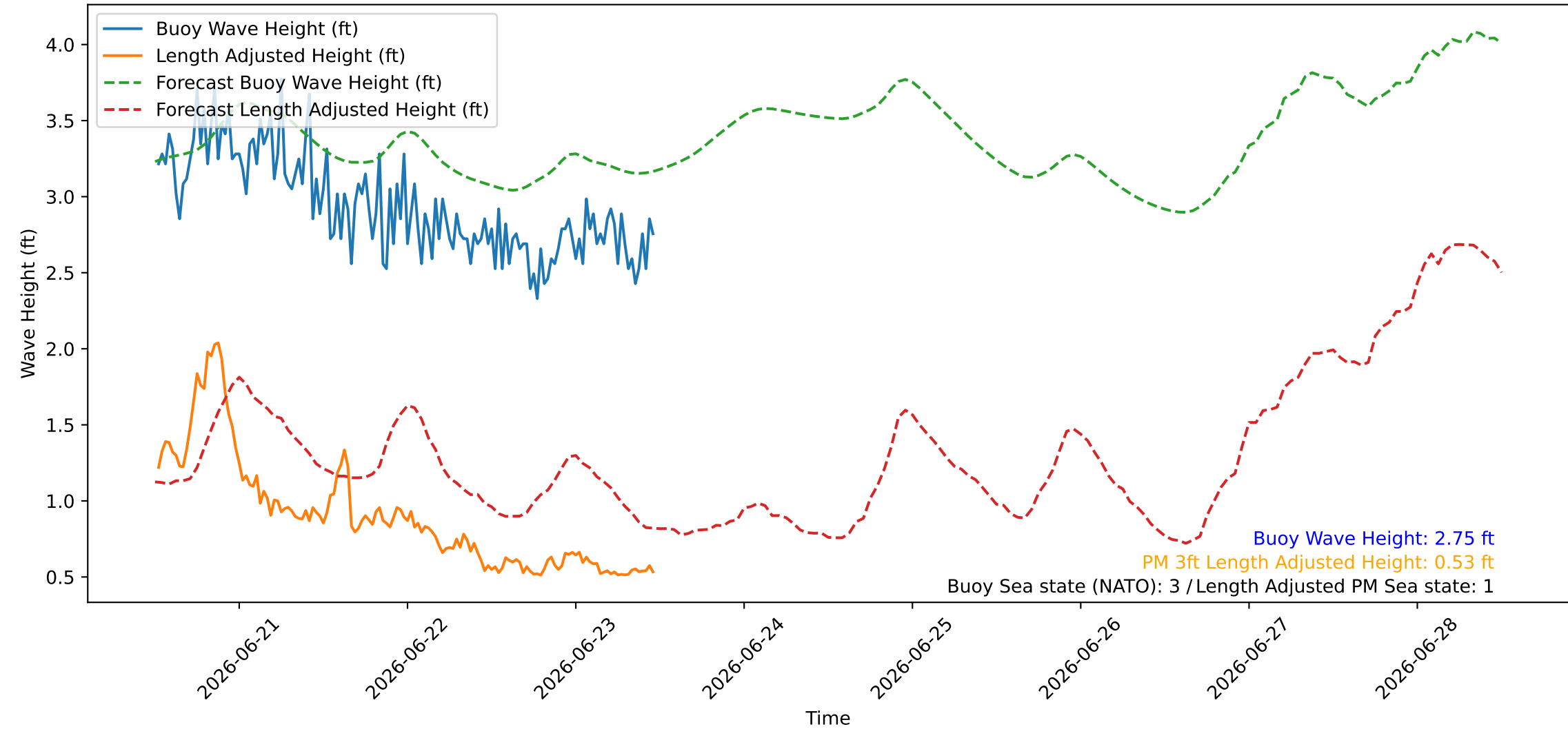
Wave Heights over Time for Red Beach at 2026-06-23 12:10:47
