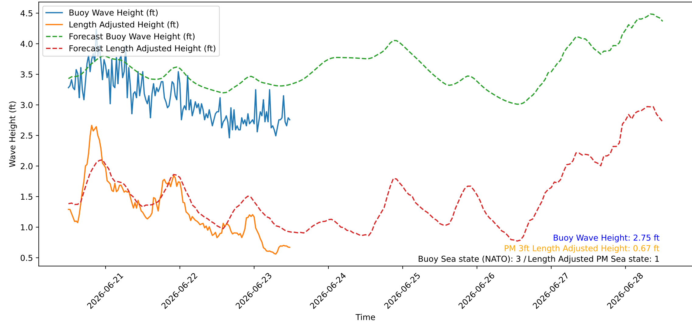
Wave Heights over Time for Green Beach at 2026-06-23 12:11:10
