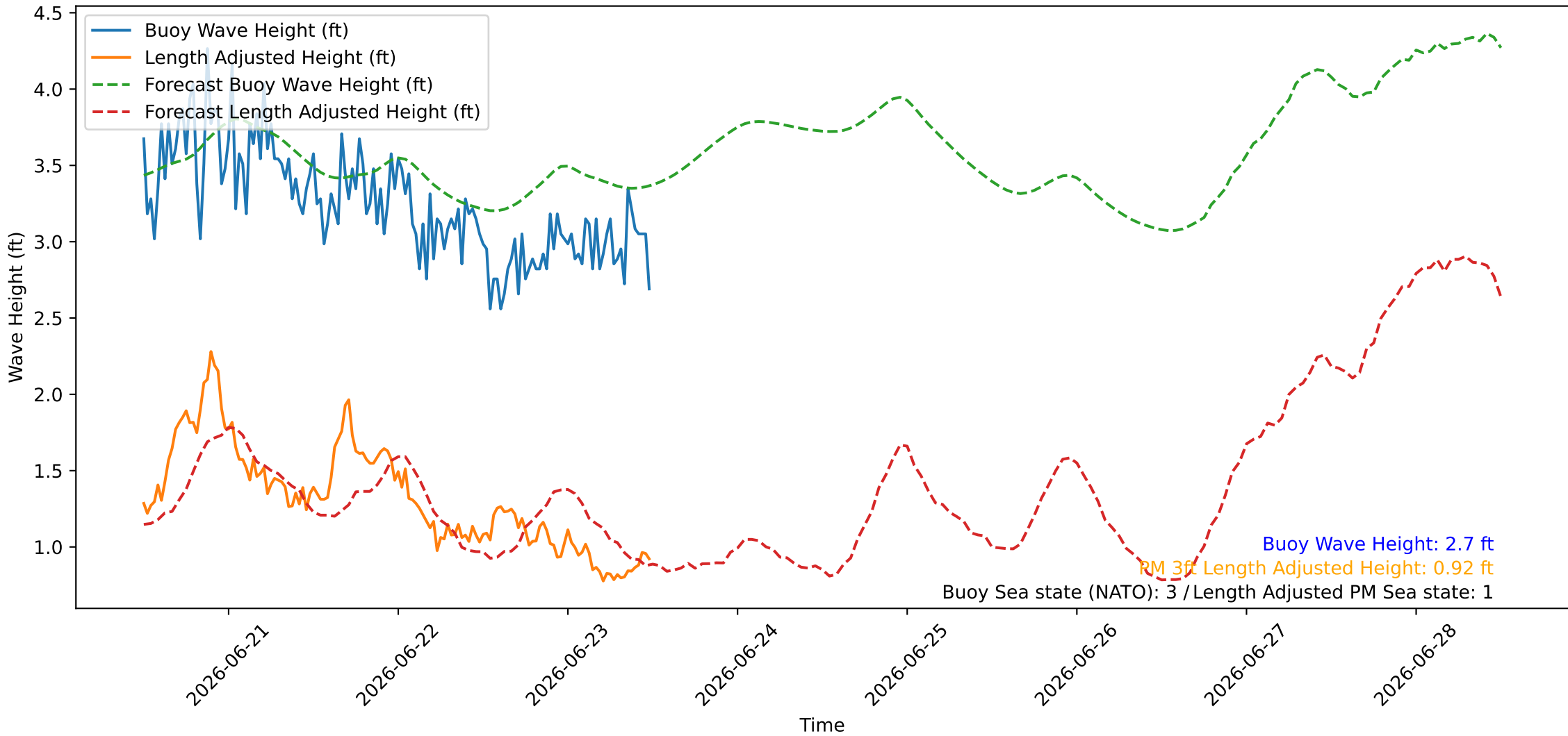
Wave Heights over Time for Oceanside Harbor at 2026-06-23 12:10:26
