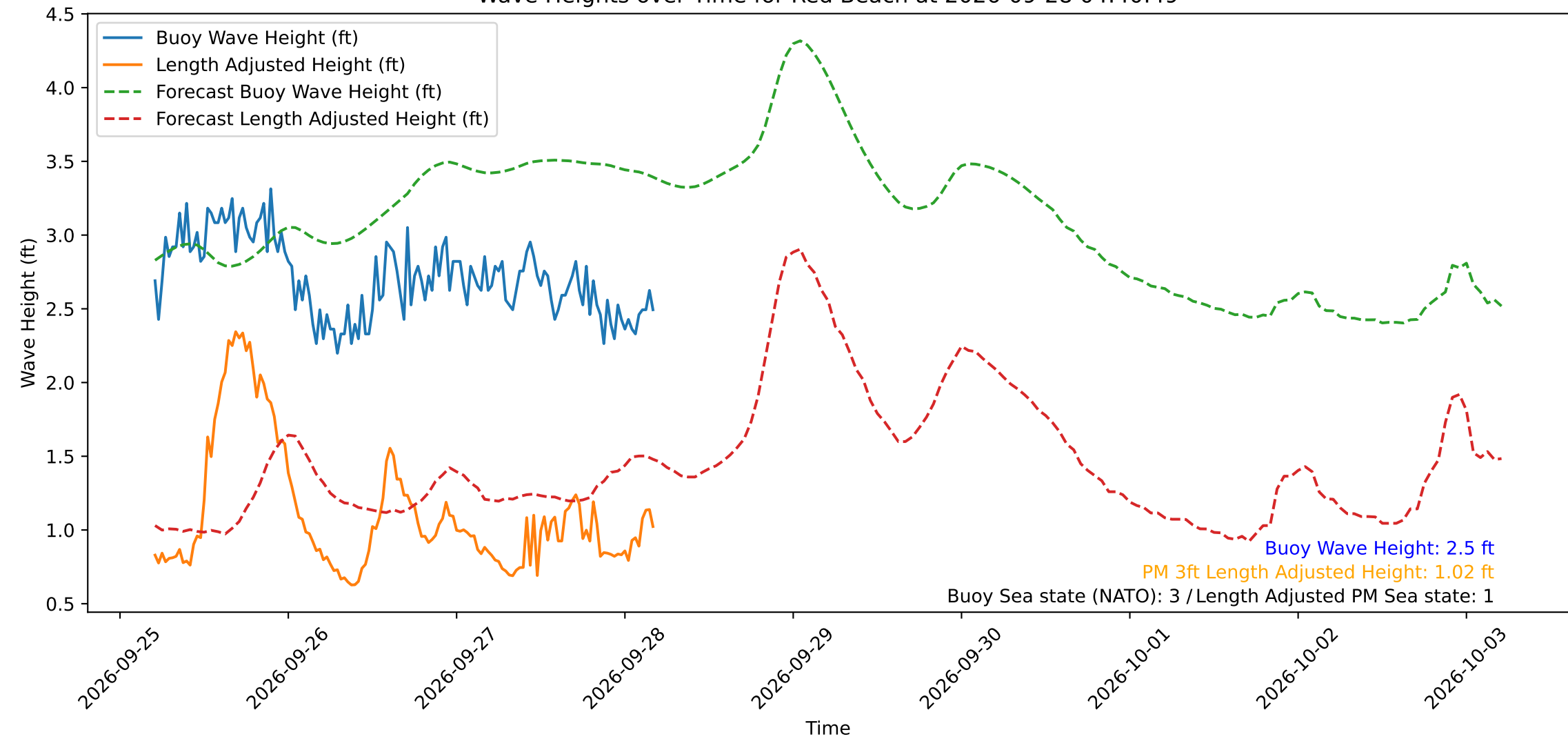
Wave Heights over Time for Red Beach at 2026-09-28 04:40:49
