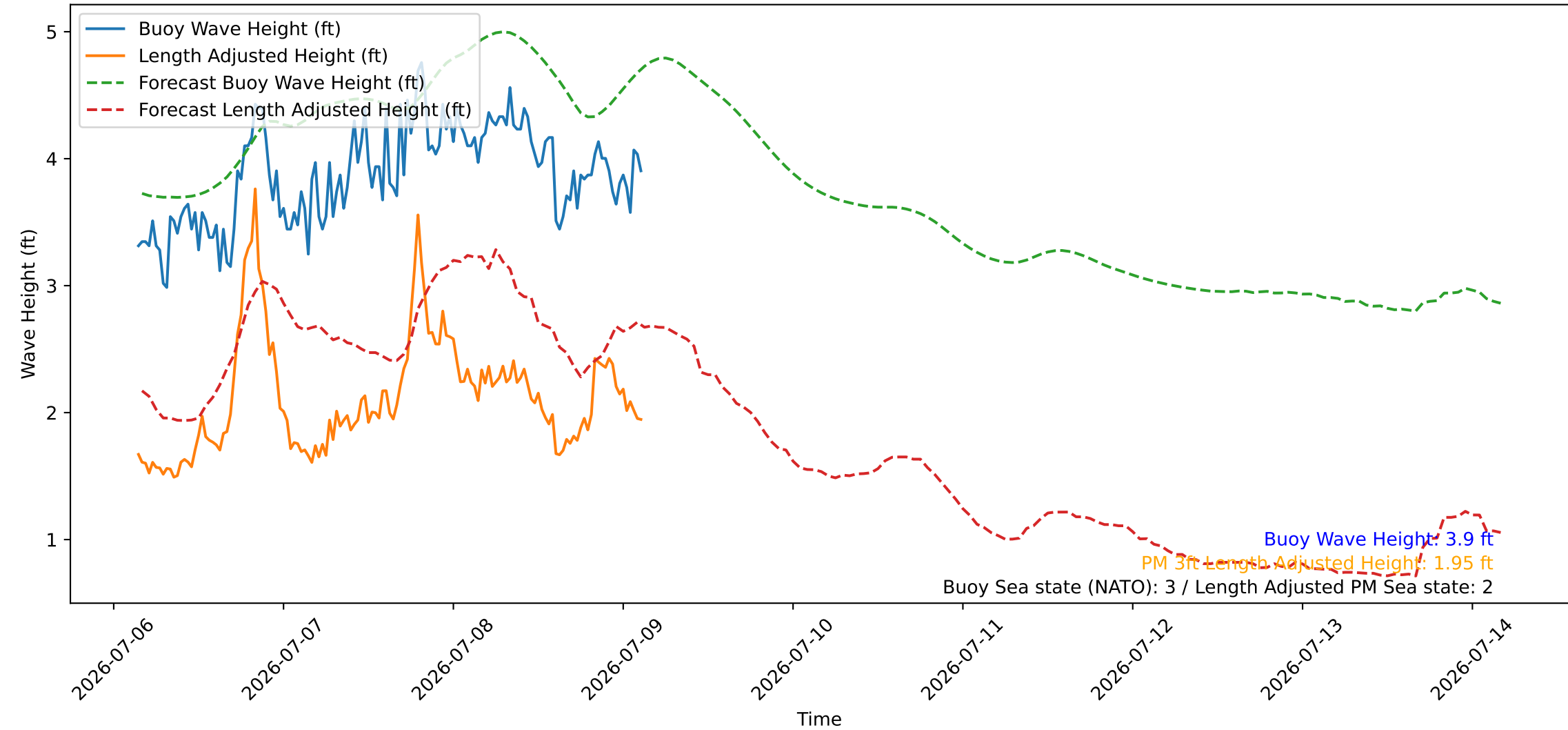
Wave Heights over Time for Green Beach at 2026-07-09 03:31:09
