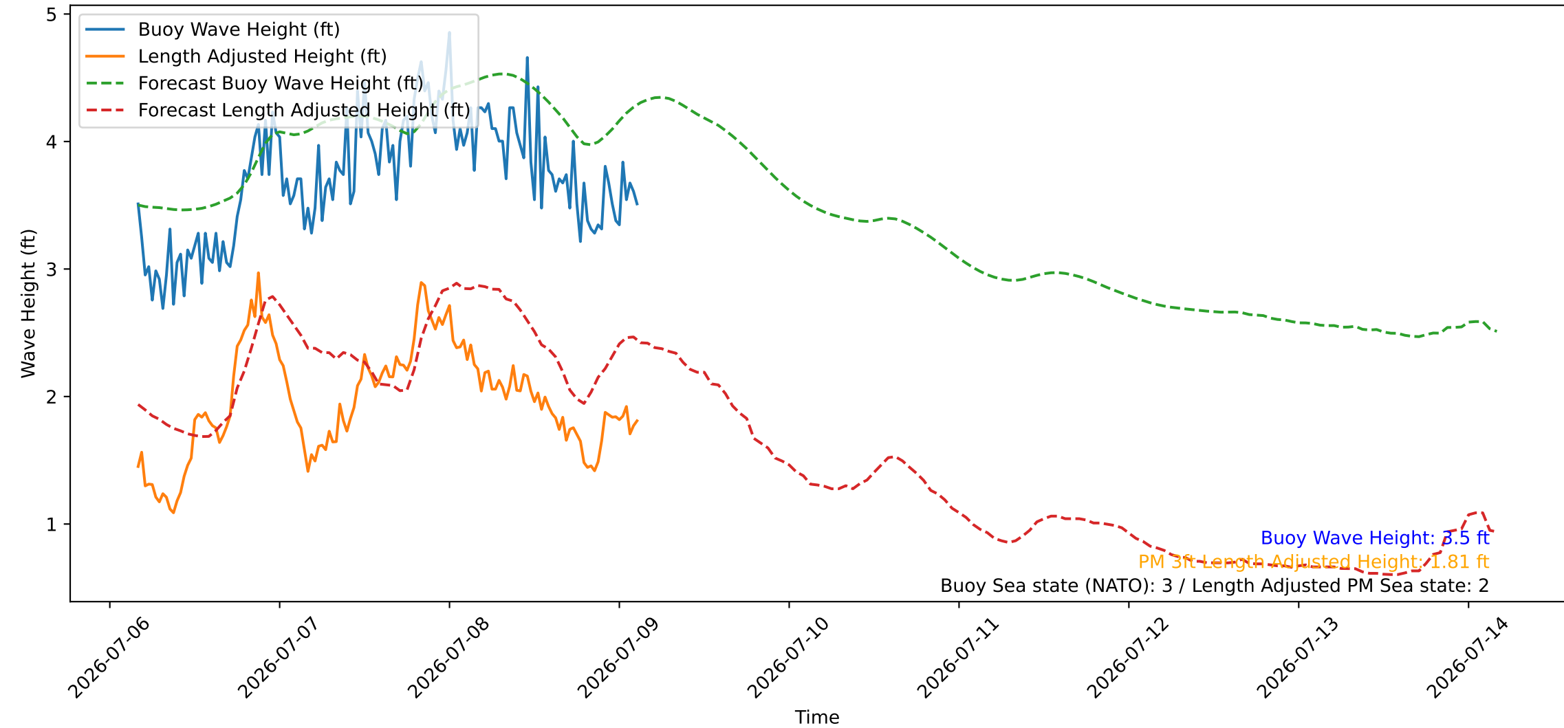
Wave Heights over Time for Red Beach at 2026-07-09 03:30:46
