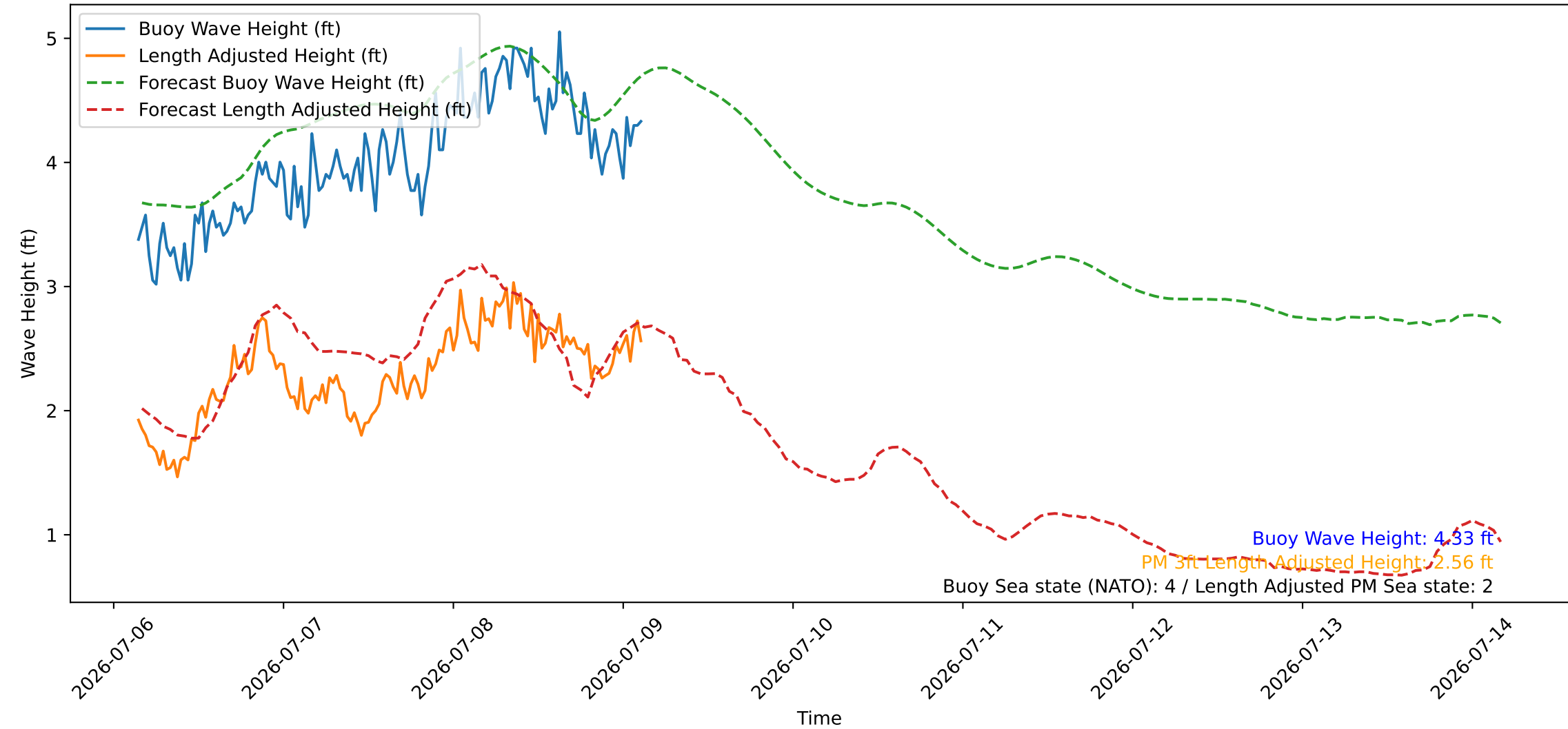
Wave Heights over Time for Oceanside Harbor at 2026-07-09 03:30:26
