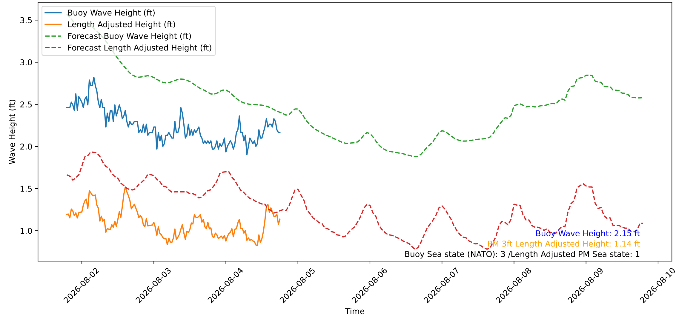
Wave Heights over Time for Red Beach at 2026-08-04 18:50:46
