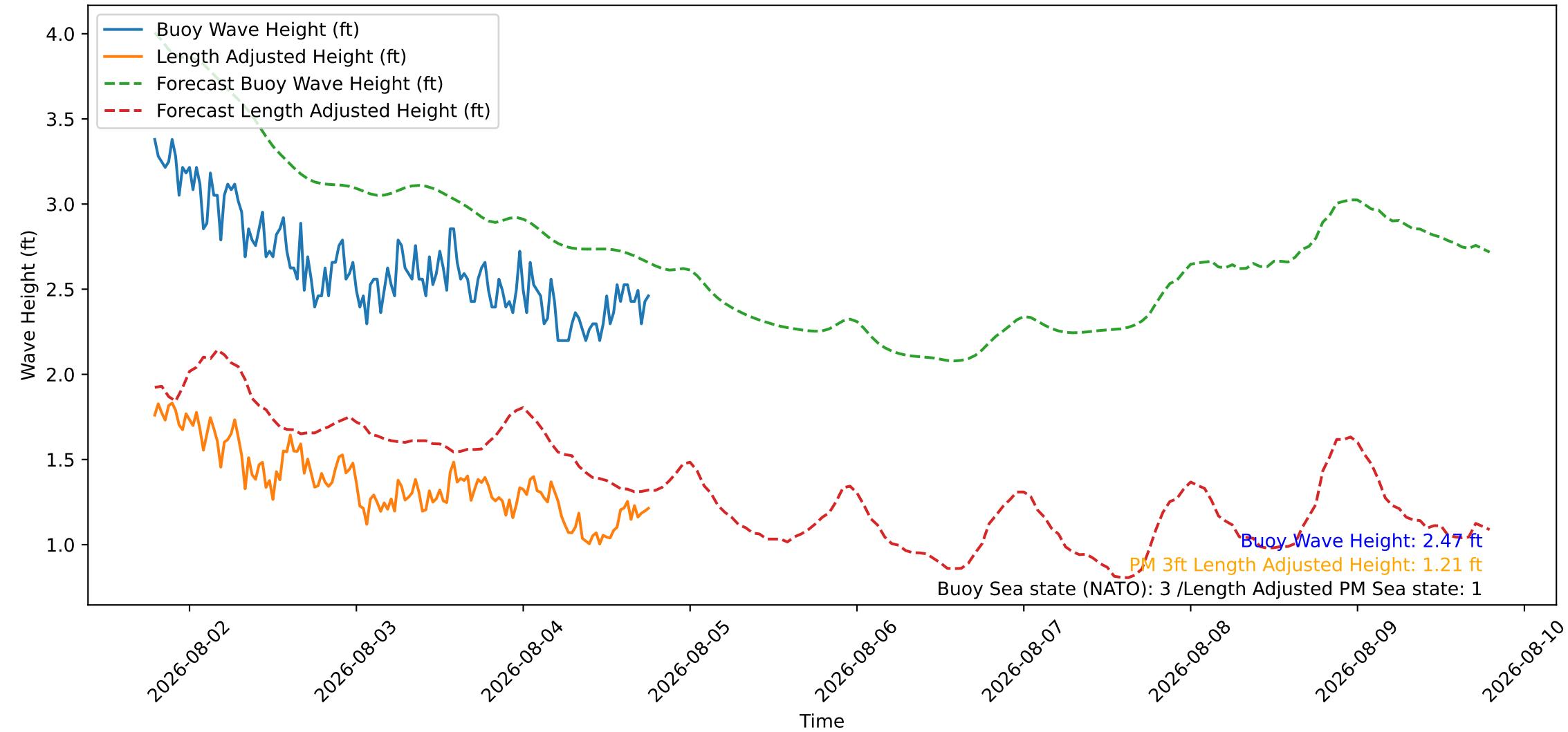
Wave Heights over Time for Oceanside Harbor at 2026-08-04 18:50:26
