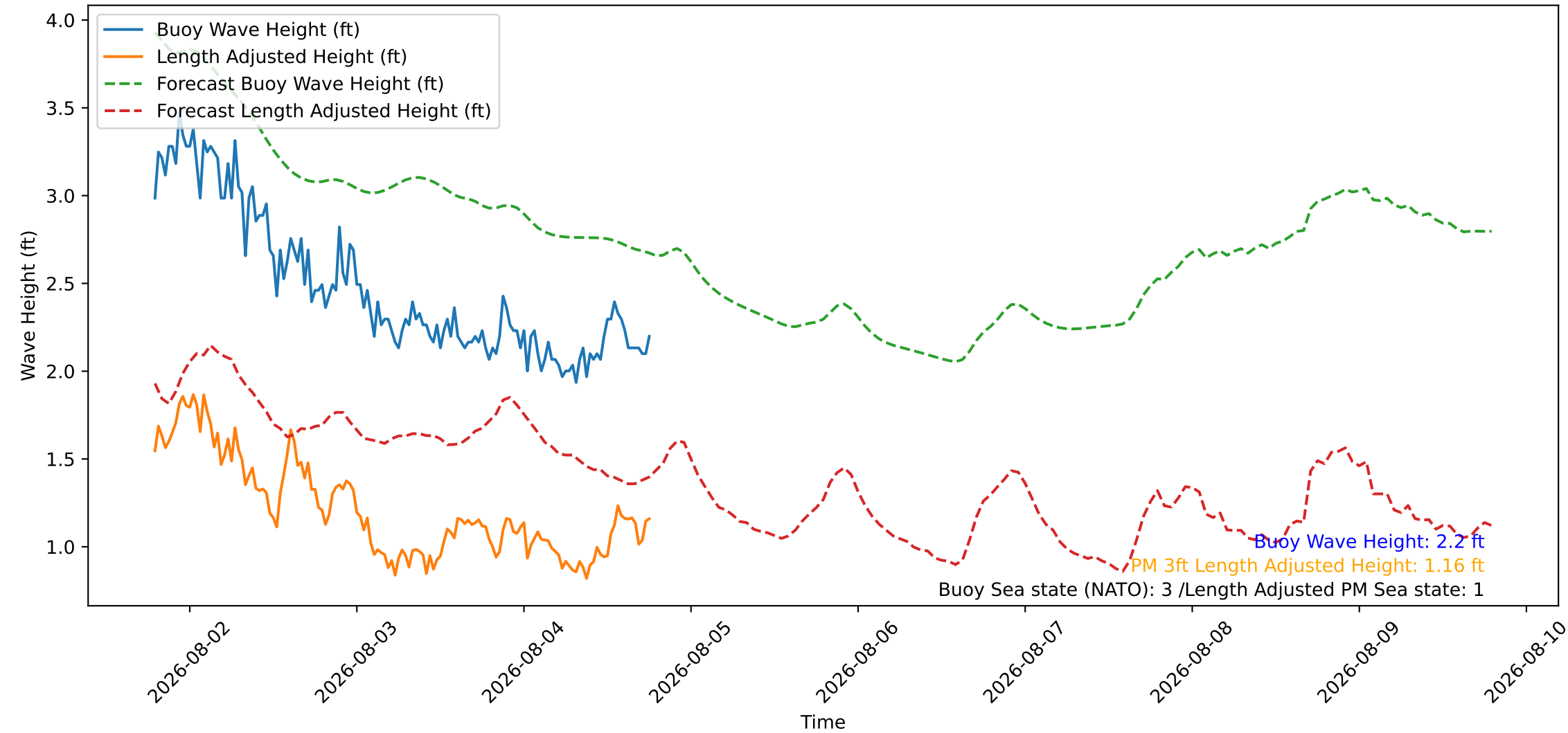
Wave Heights over Time for Green Beach at 2026-08-04 18:51:09
