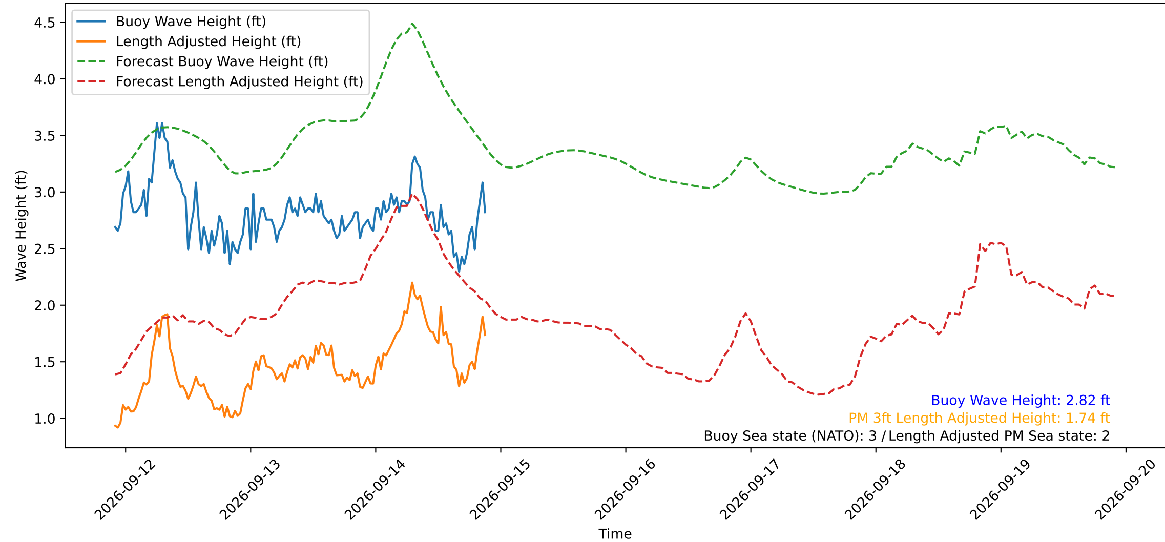
Wave Heights over Time for Green Beach at 2026-09-14 21:51:15
