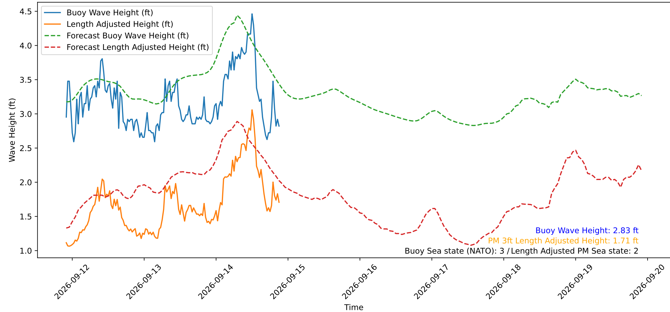
Wave Heights over Time for Oceanside Harbor at 2026-09-14 21:50:29
