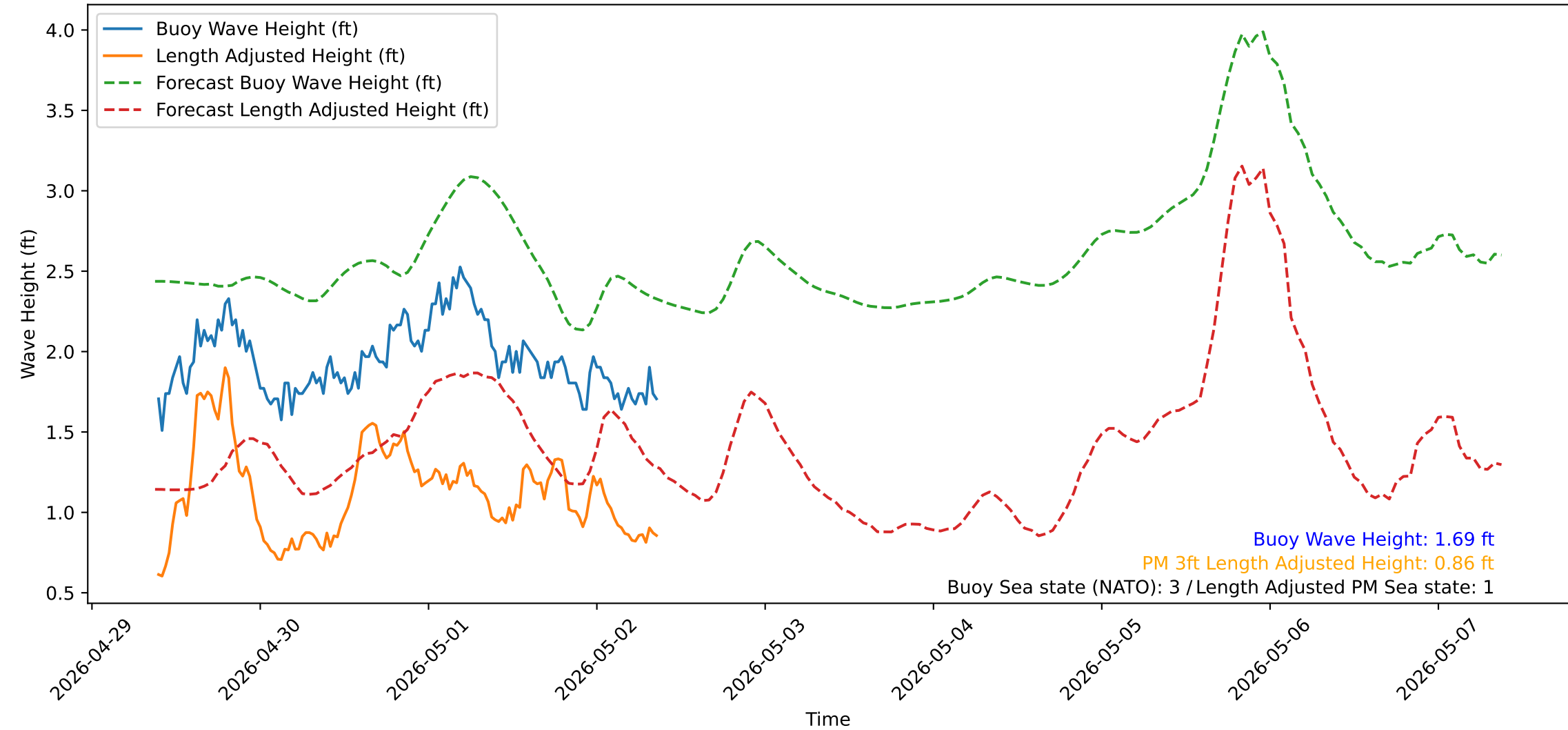
Wave Heights over Time for Red Beach at 2026-05-02 09:20:52
