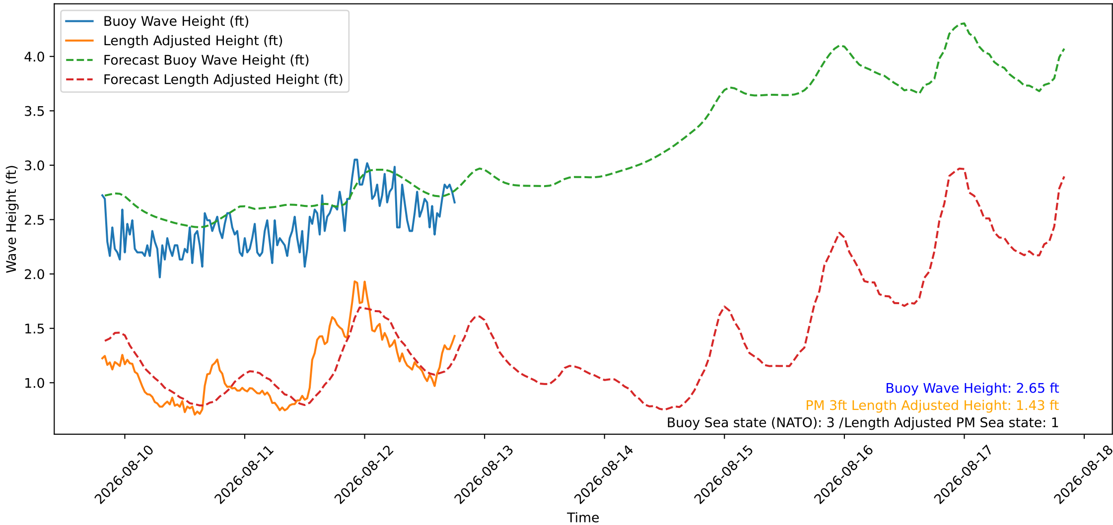
Wave Heights over Time for Oceanside Harbor at 2026-08-12 19:30:26
