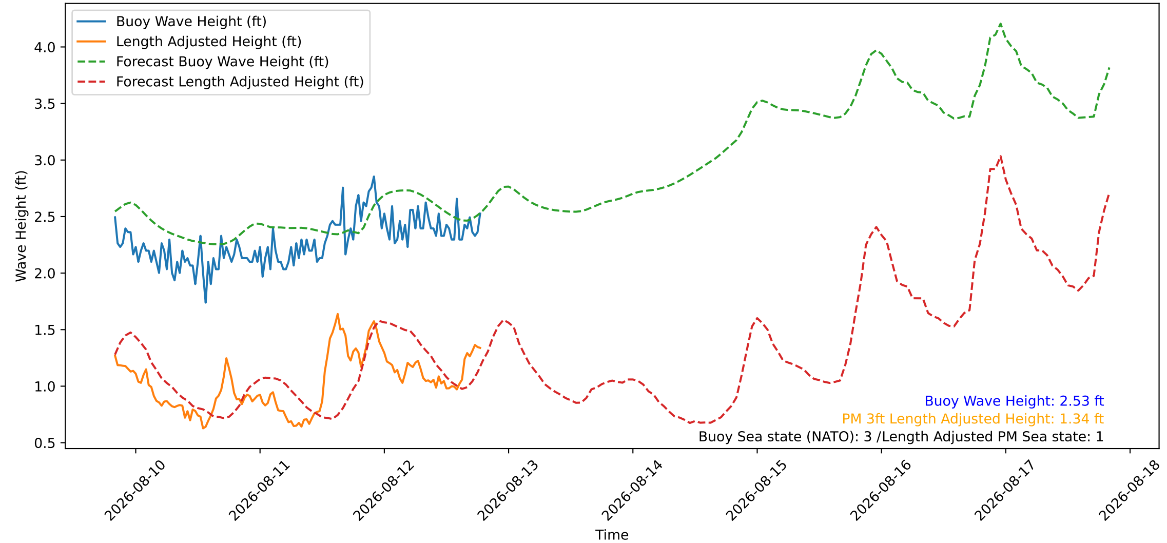
Wave Heights over Time for Red Beach at 2026-08-12 19:30:46
