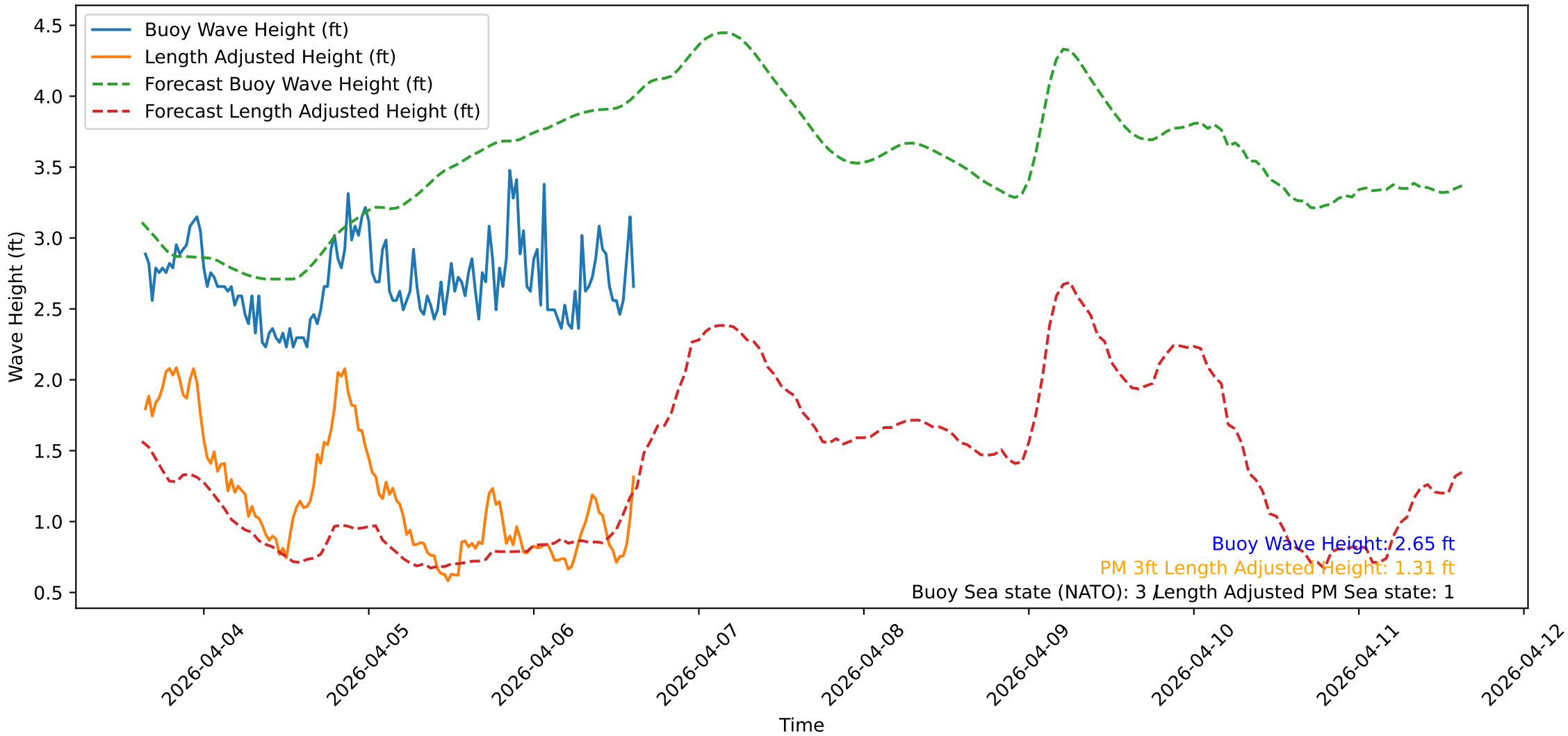
Wave Heights over Time for Green Beach at 2026-04-06 15:21:10
