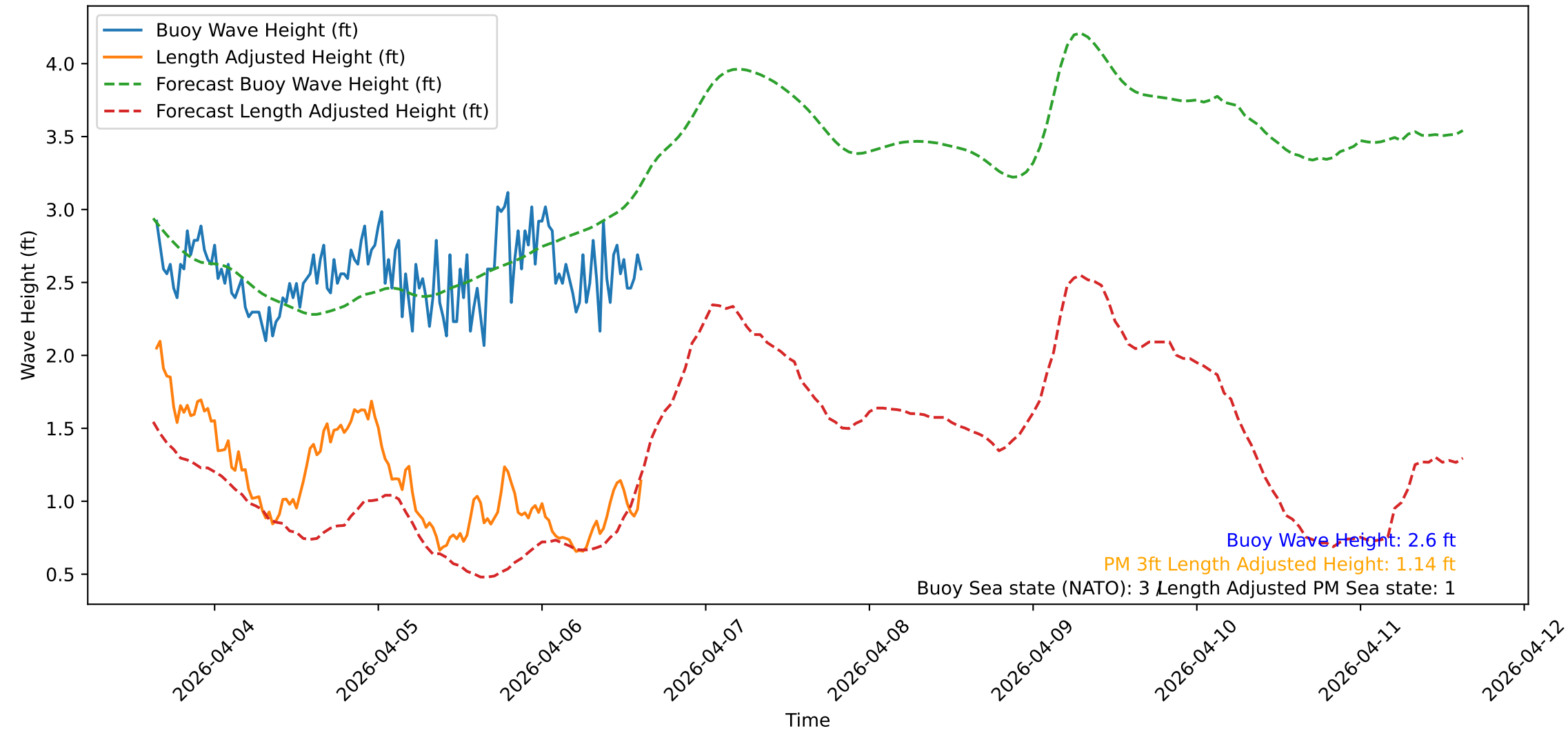
Wave Heights over Time for Oceanside Harbor at 2026-04-06 15:20:32
