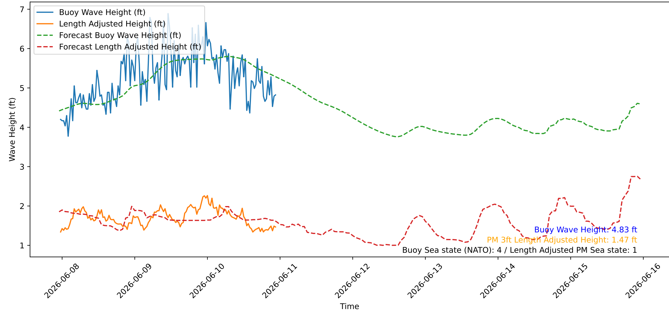
Wave Heights over Time for Green Beach at 2026-06-10 23:21:11
