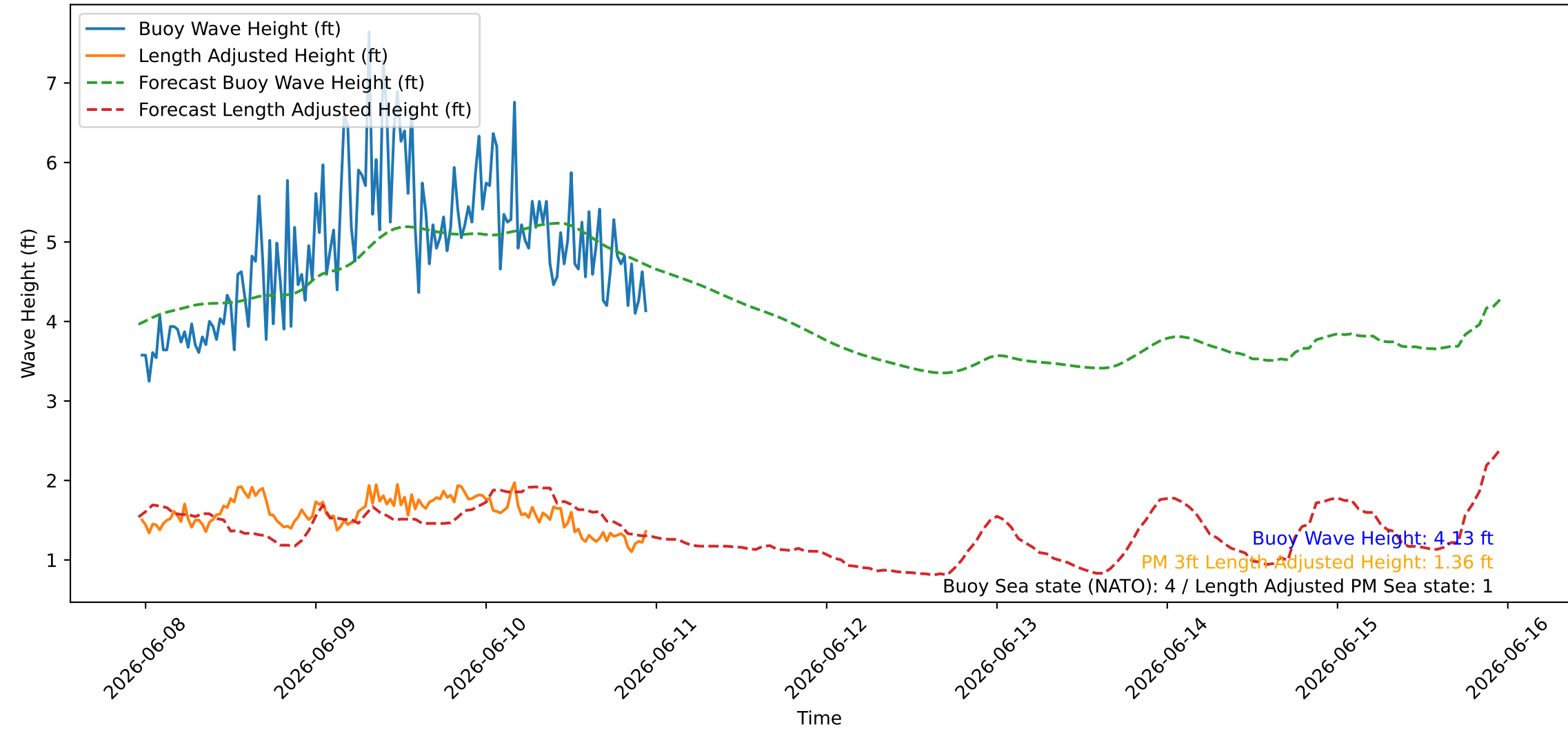
Wave Heights over Time for Red Beach at 2026-06-10 23:20:48
