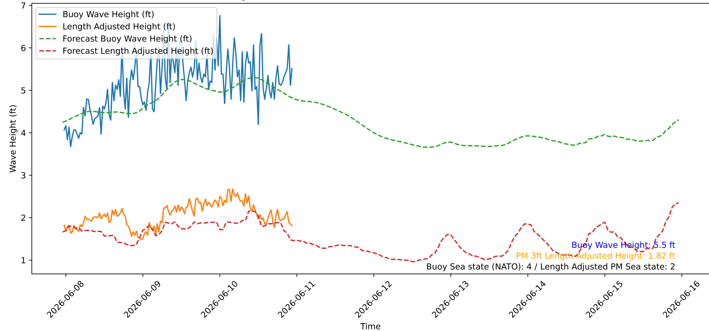
Wave Heights over Time for Oceanside Harbor at 2026-06-10 23:20:26
