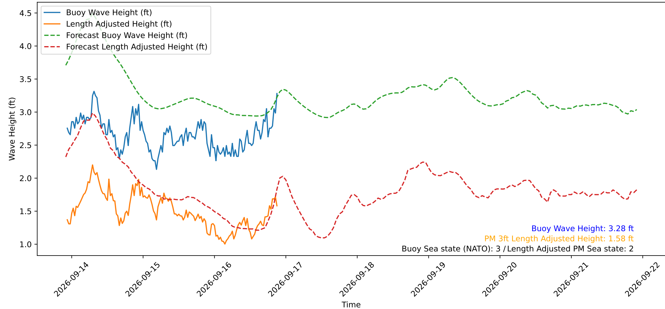
Wave Heights over Time for Green Beach at 2026-09-16 22:01:12
