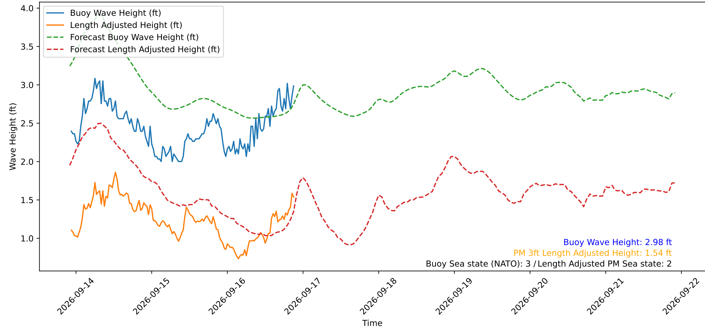
Wave Heights over Time for Red Beach at 2026-09-16 22:00:49
