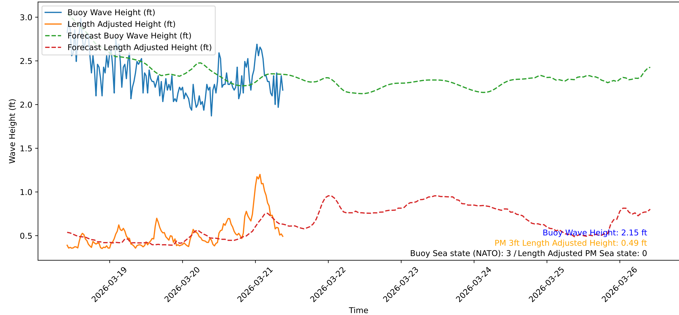
Wave Heights over Time for Red Beach at 2026-03-21 09:50:48
