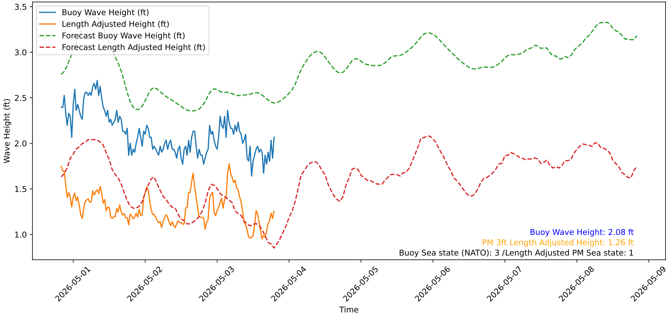
Wave Heights over Time for Oceanside Harbor at 2026-05-03 20:00:31
