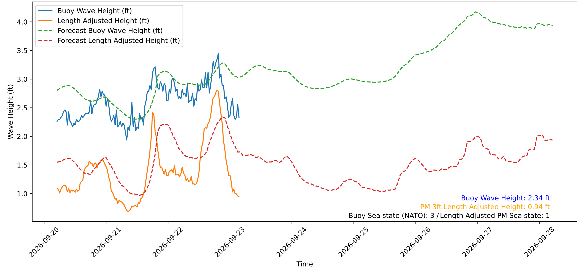
Wave Heights over Time for Green Beach at 2026-09-23 04:31:11
