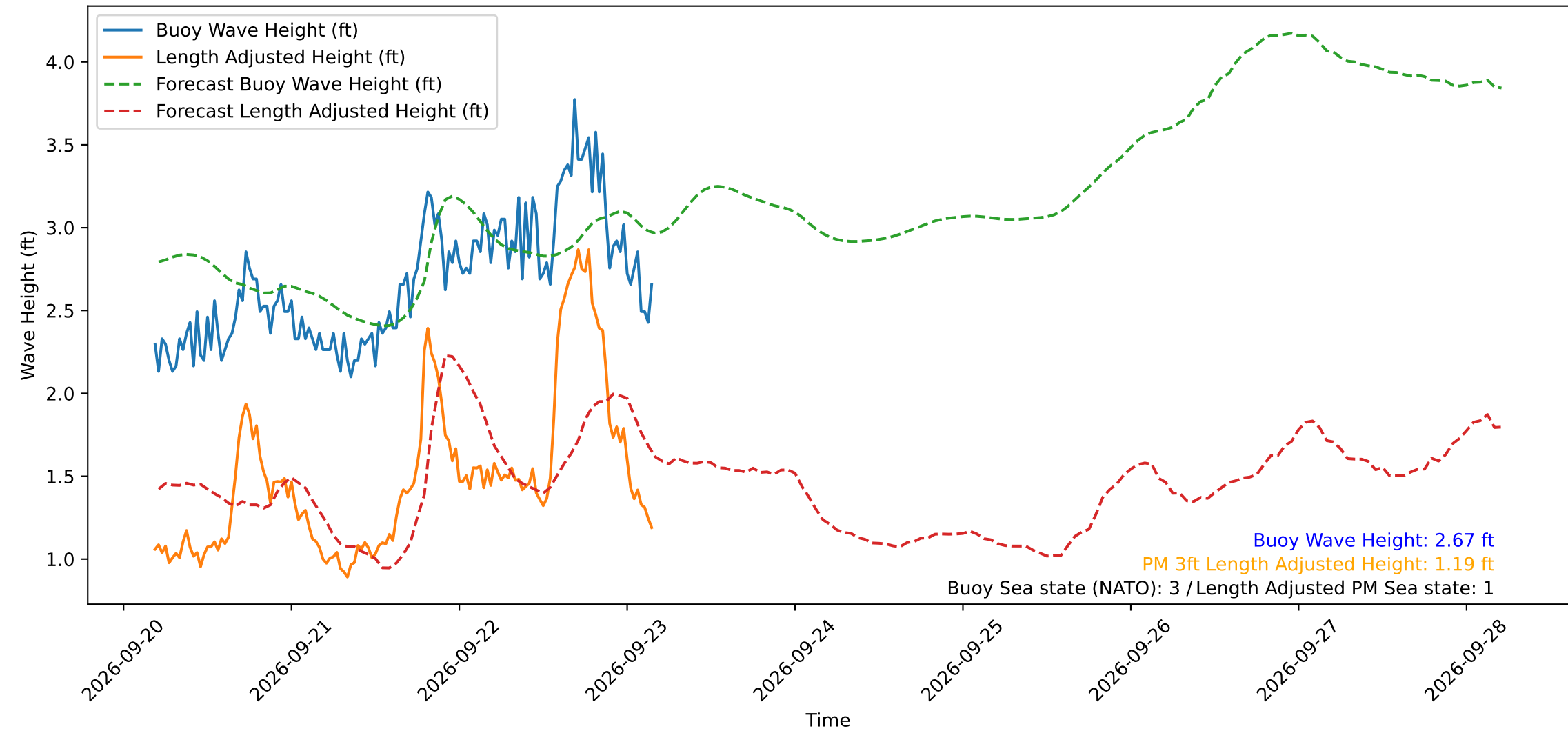
Wave Heights over Time for Oceanside Harbor at 2026-09-23 04:30:29
