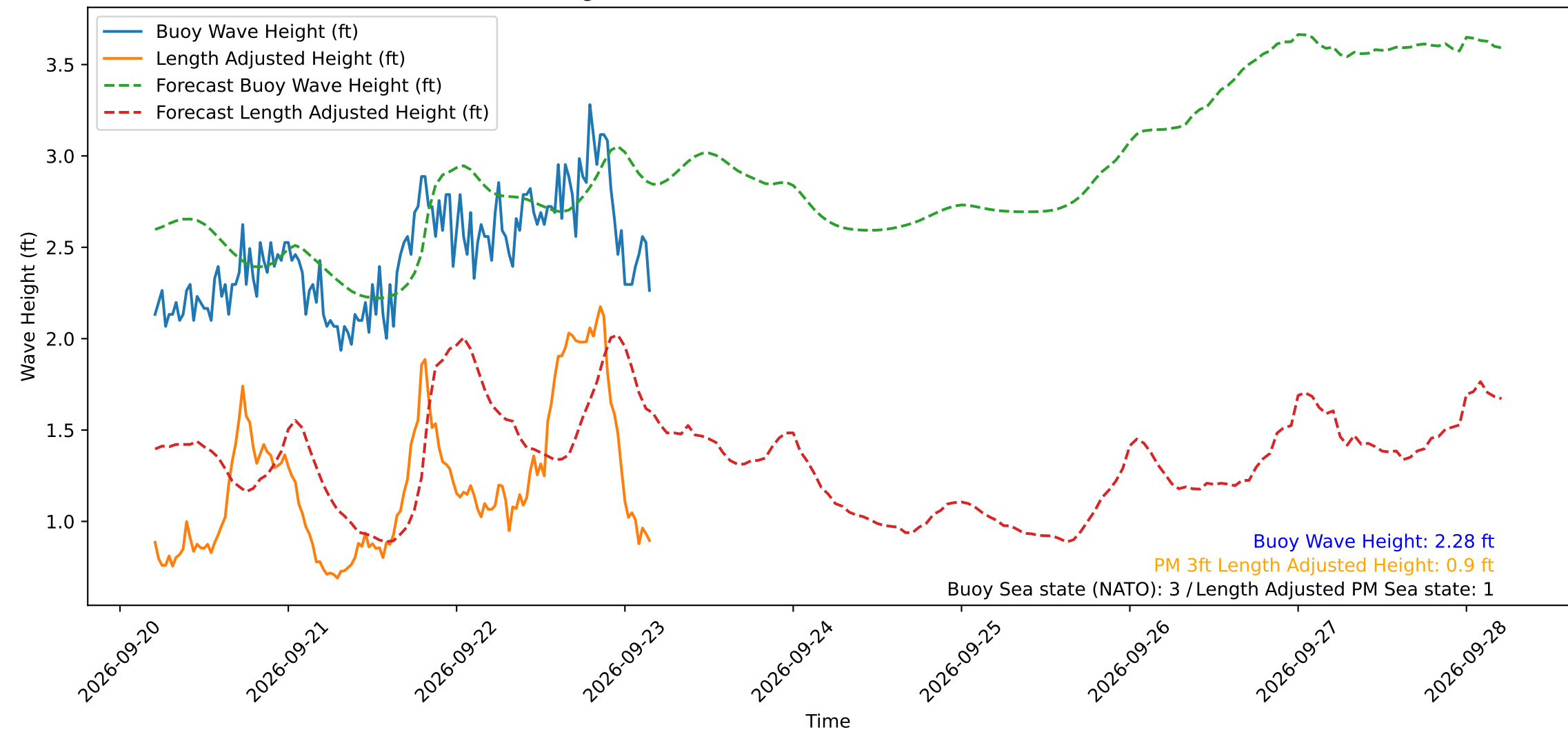
Wave Heights over Time for Red Beach at 2026-09-23 04:30:49
