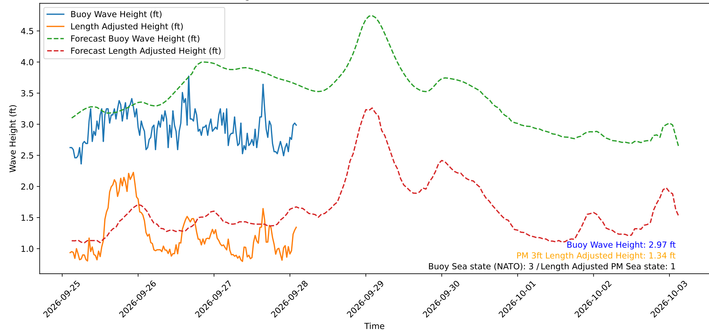
Wave Heights over Time for Oceanside Harbor at 2026-09-28 02:40:30
