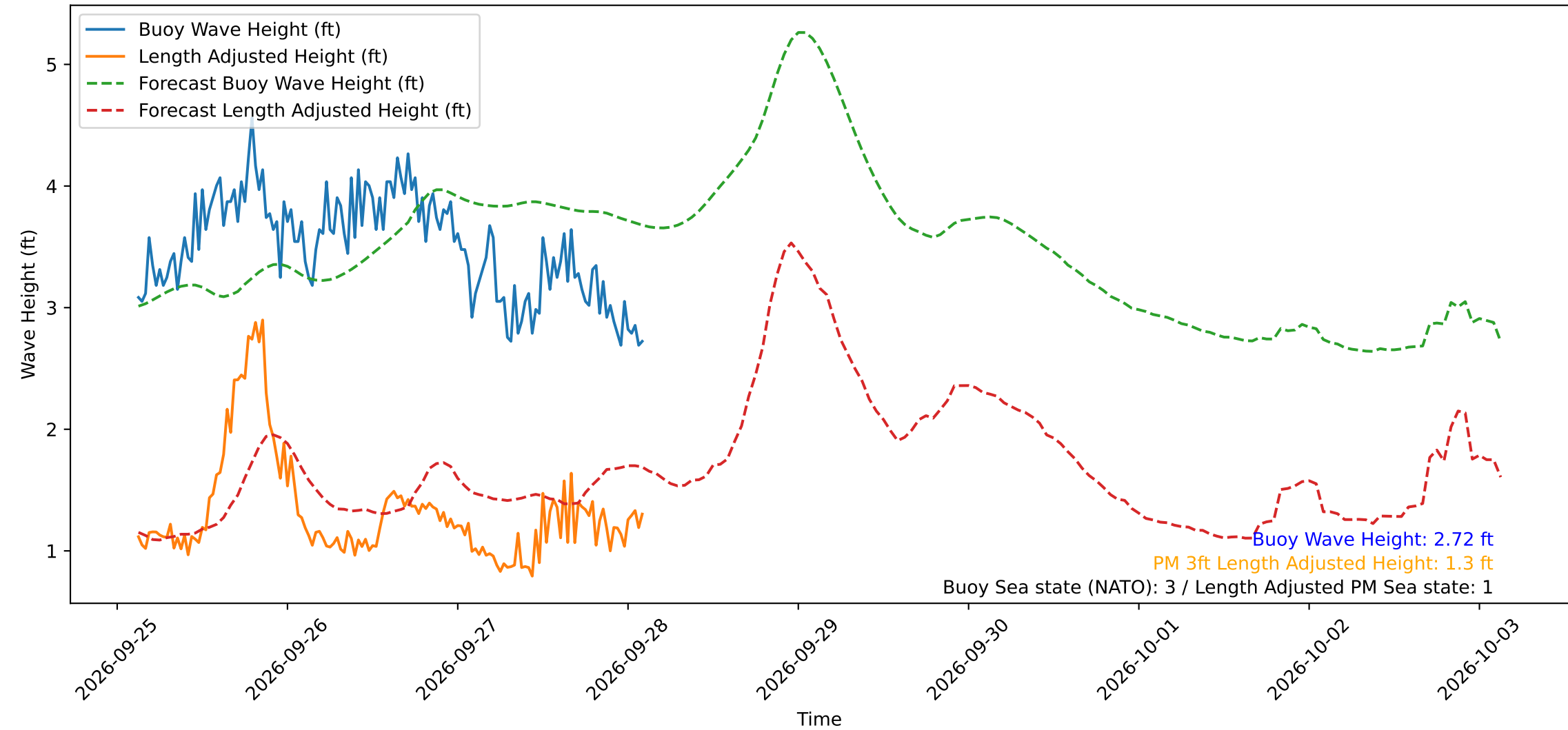
Wave Heights over Time for Green Beach at 2026-09-28 02:41:12
