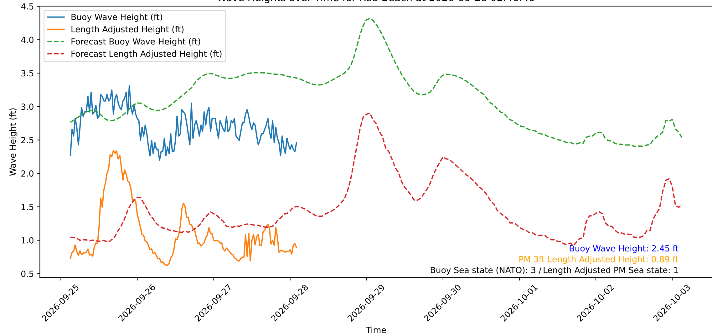
Wave Heights over Time for Red Beach at 2026-09-28 02:40:49
