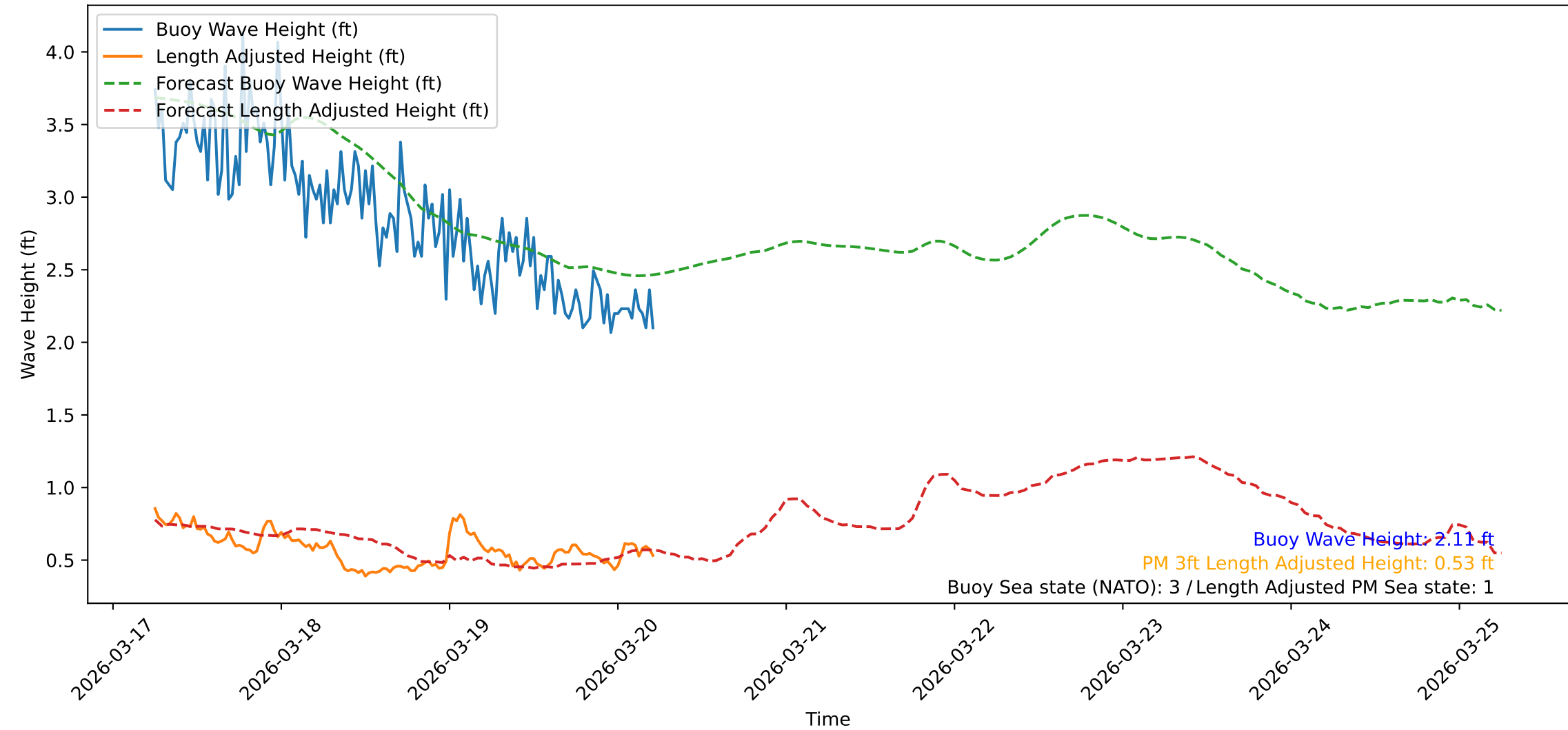
Wave Heights over Time for Green Beach at 2026-03-20 05:51:10
