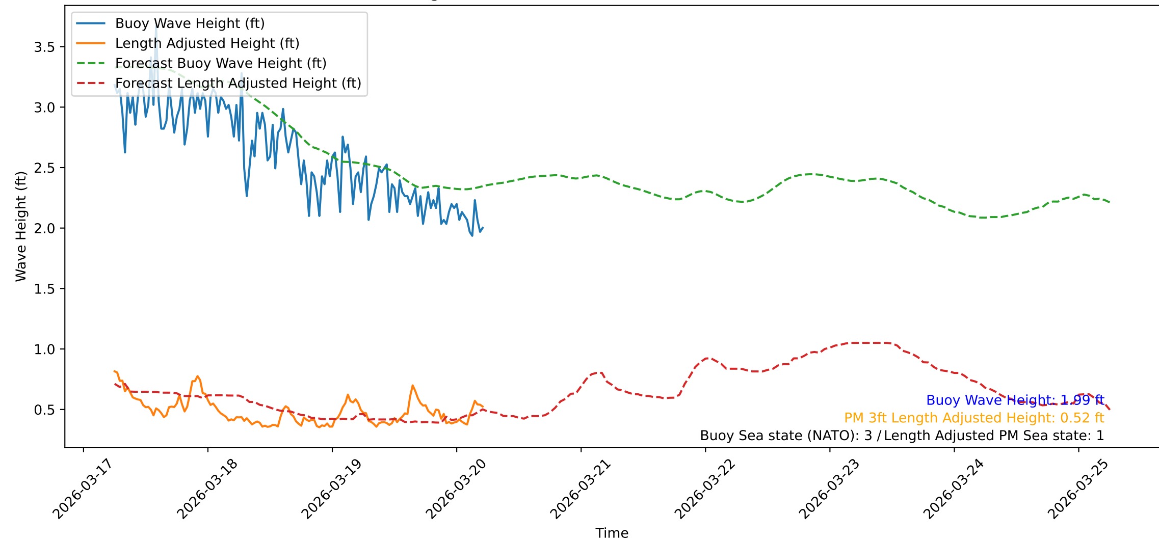
Wave Heights over Time for Red Beach at 2026-03-20 05:50:47
