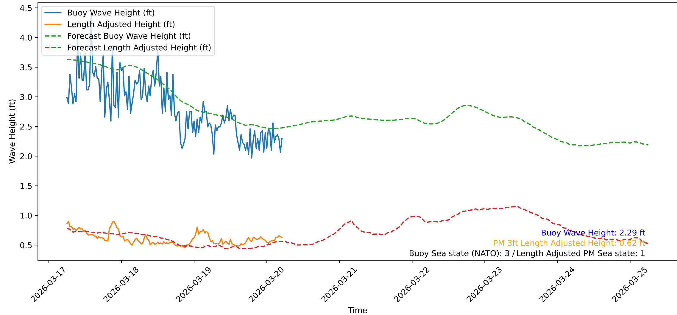
Wave Heights over Time for Oceanside Harbor at 2026-03-20 05:50:31
