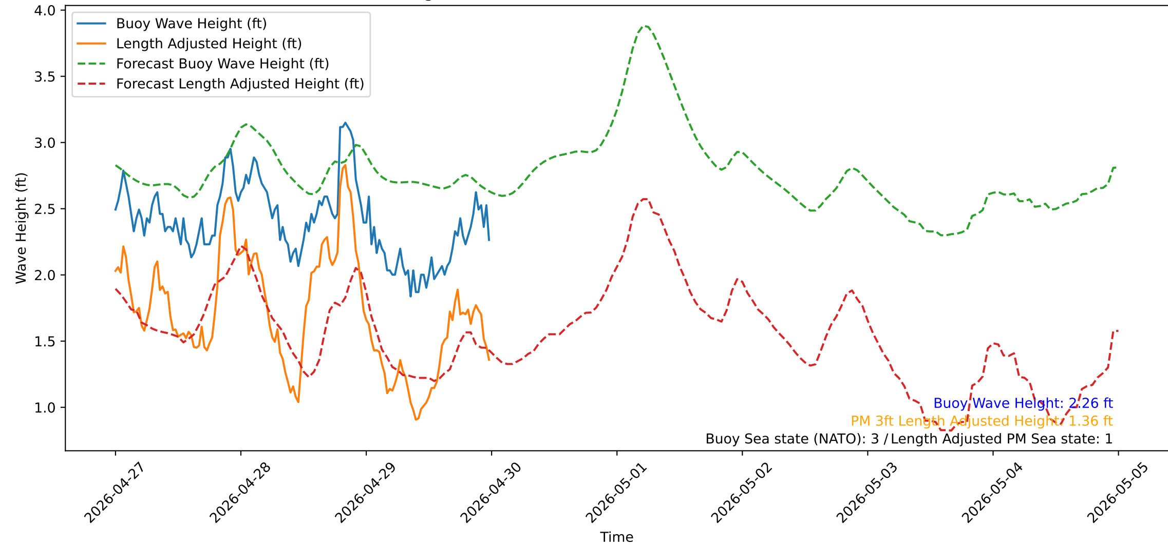
Wave Heights over Time for Green Beach at 2026-04-30 00:11:12
