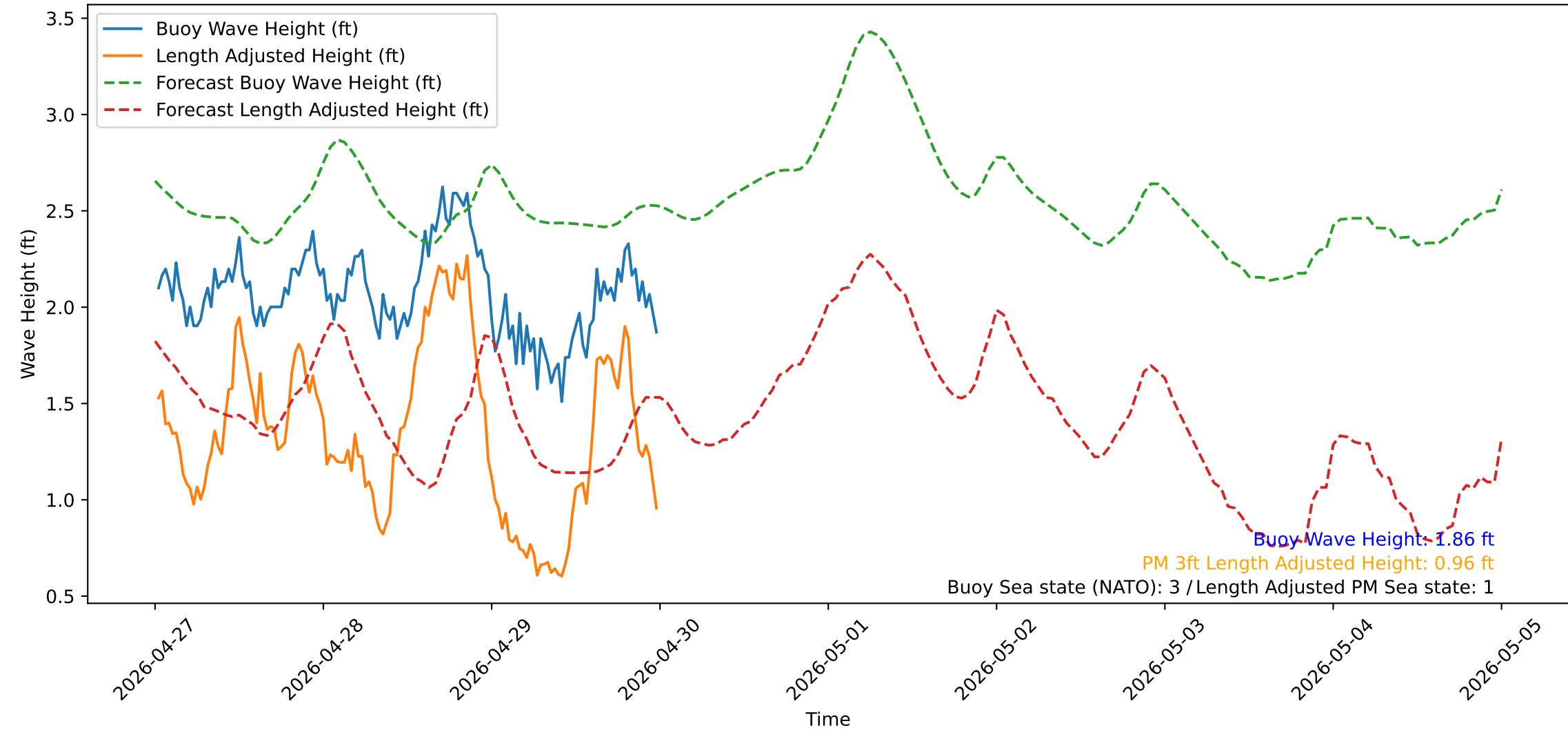
Wave Heights over Time for Red Beach at 2026-04-30 00:10:50
