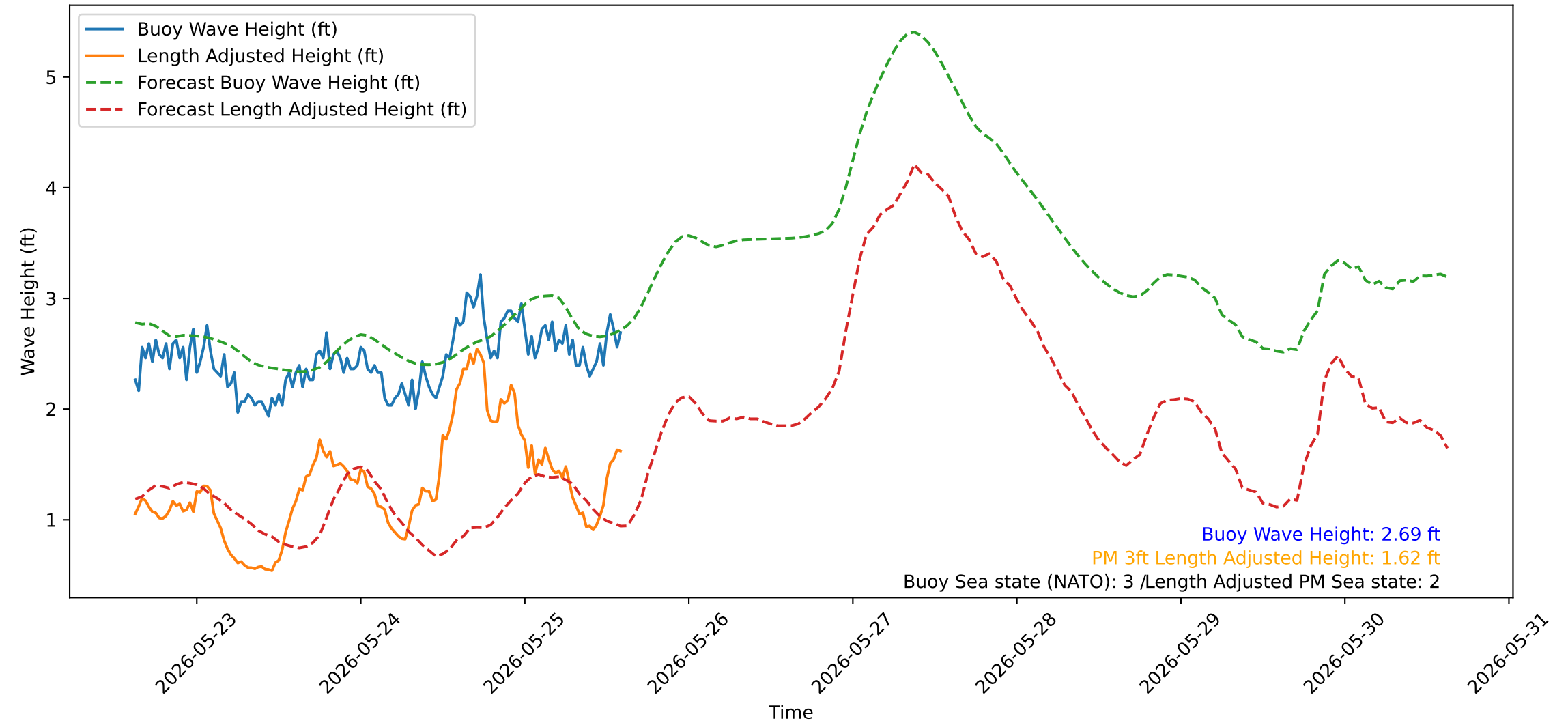
Wave Heights over Time for Red Beach at 2026-05-25 14:50:51
