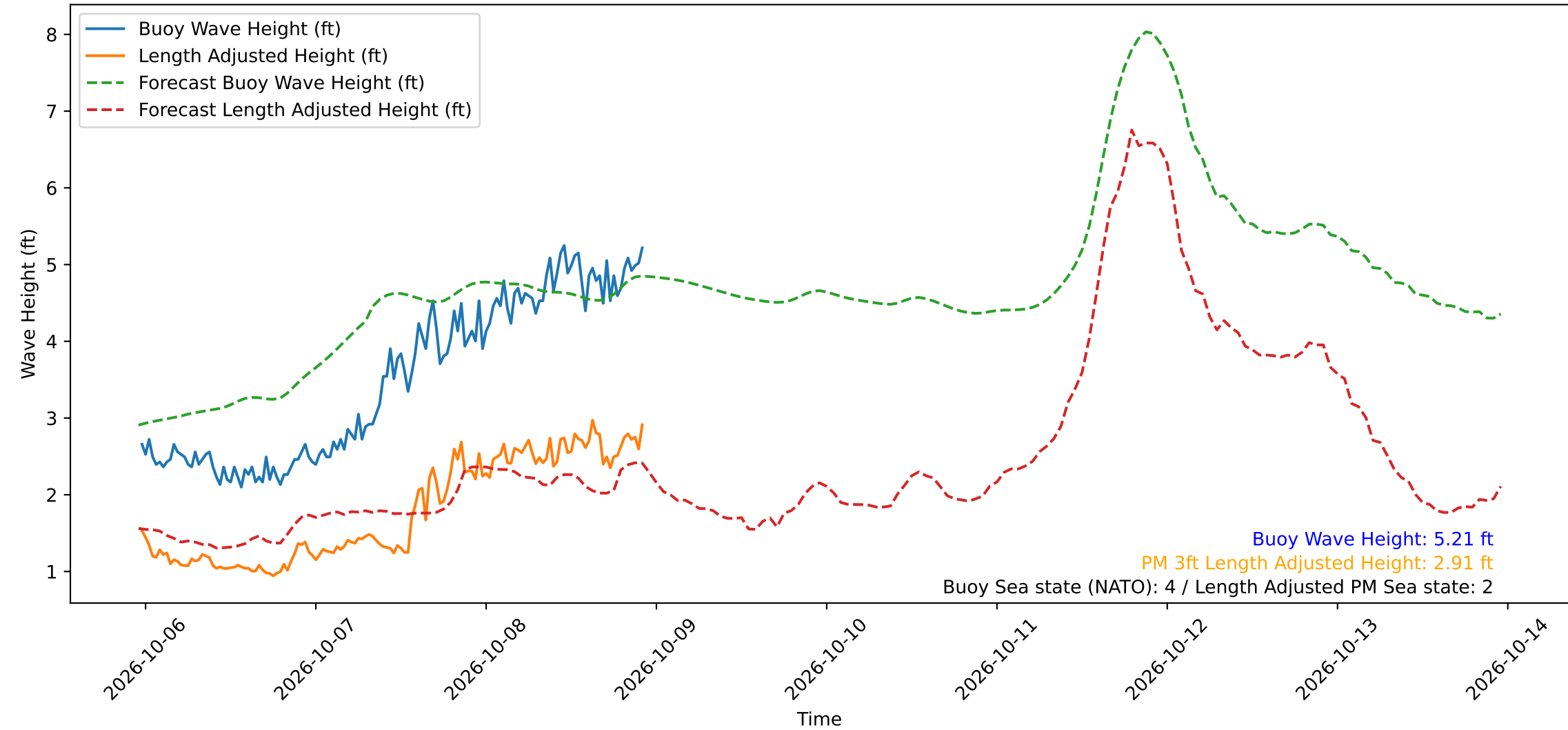
Wave Heights over Time for Green Beach at 2026-10-08 23:01:11
