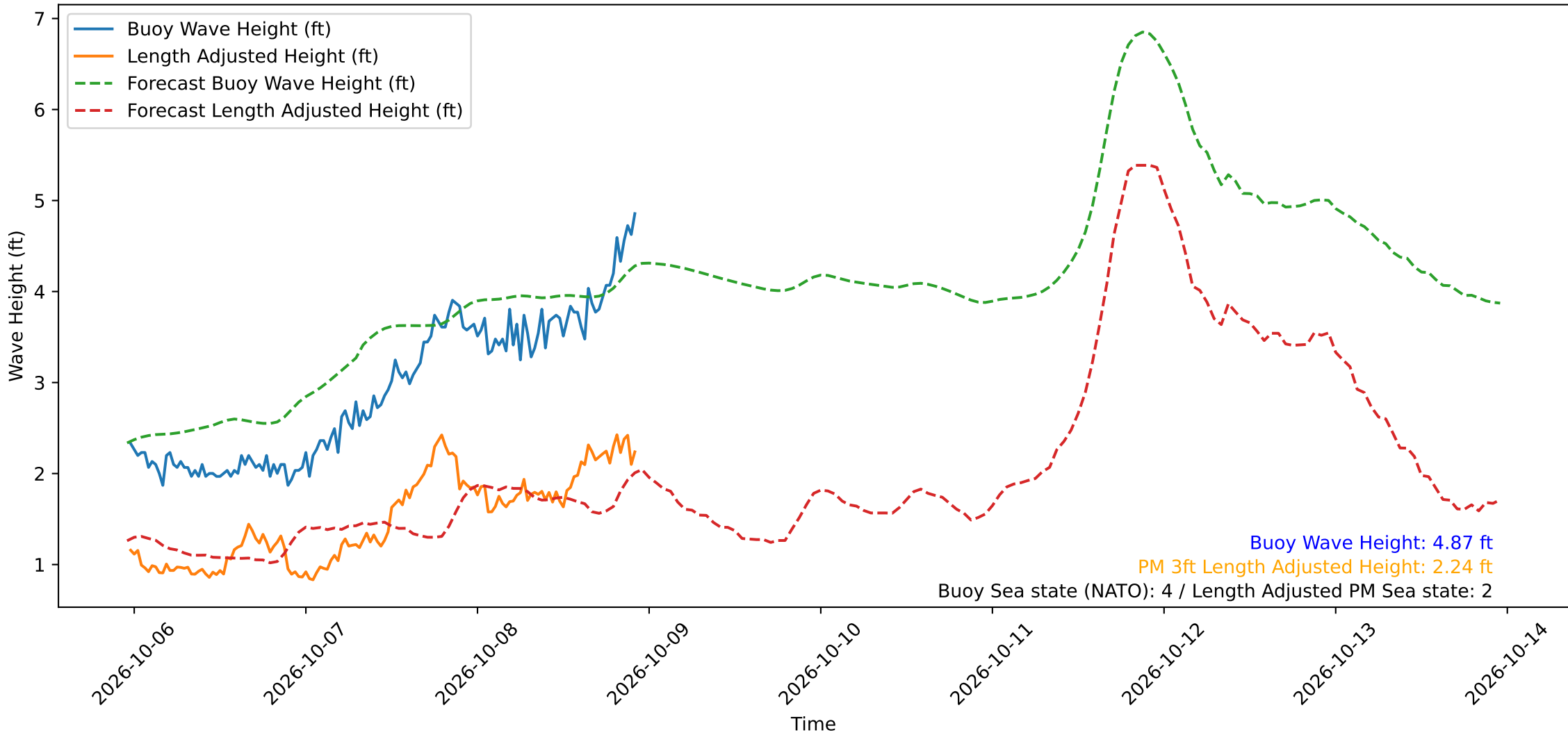
Wave Heights over Time for Red Beach at 2026-10-08 23:00:49
