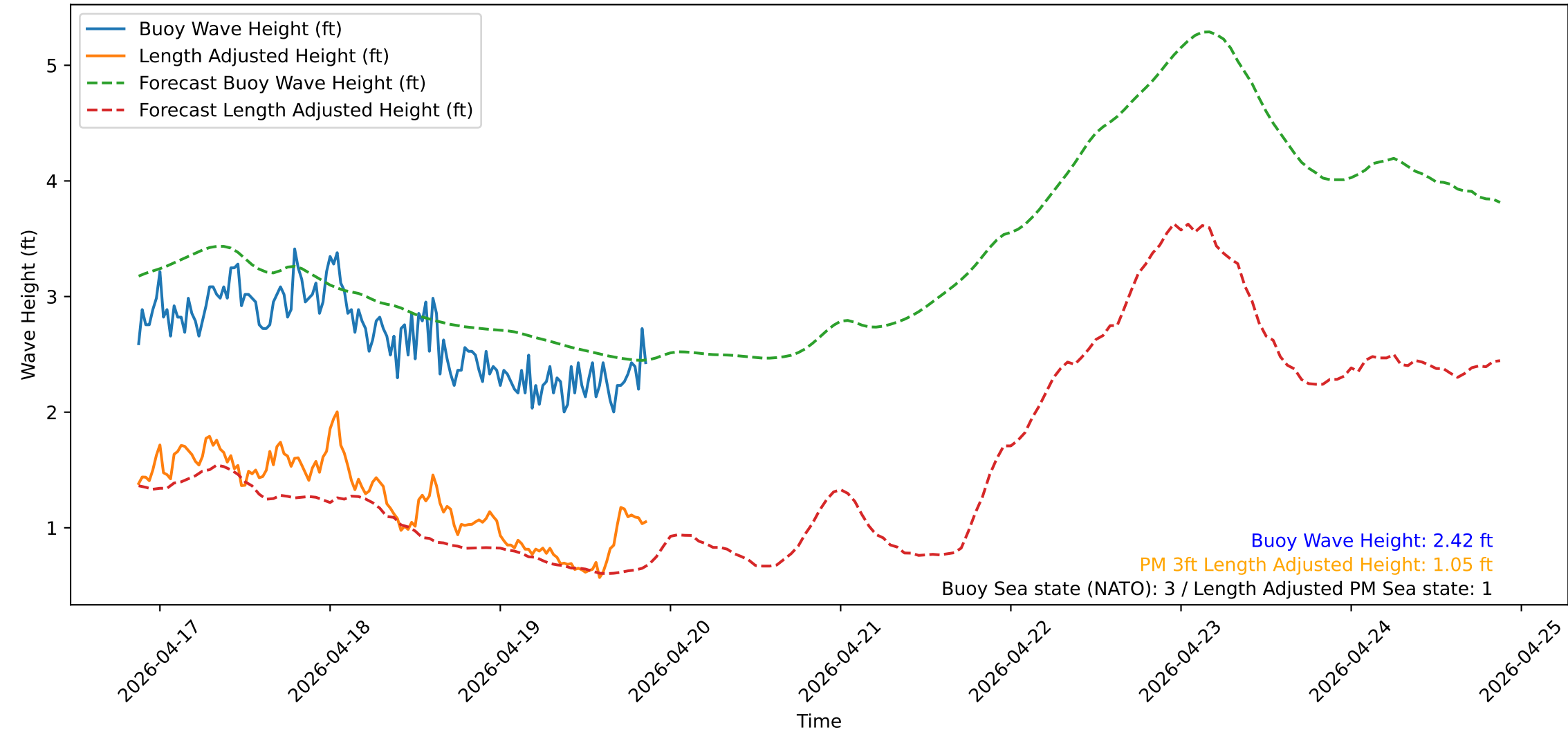
Wave Heights over Time for Oceanside Harbor at 2026-04-19 21:00:31
