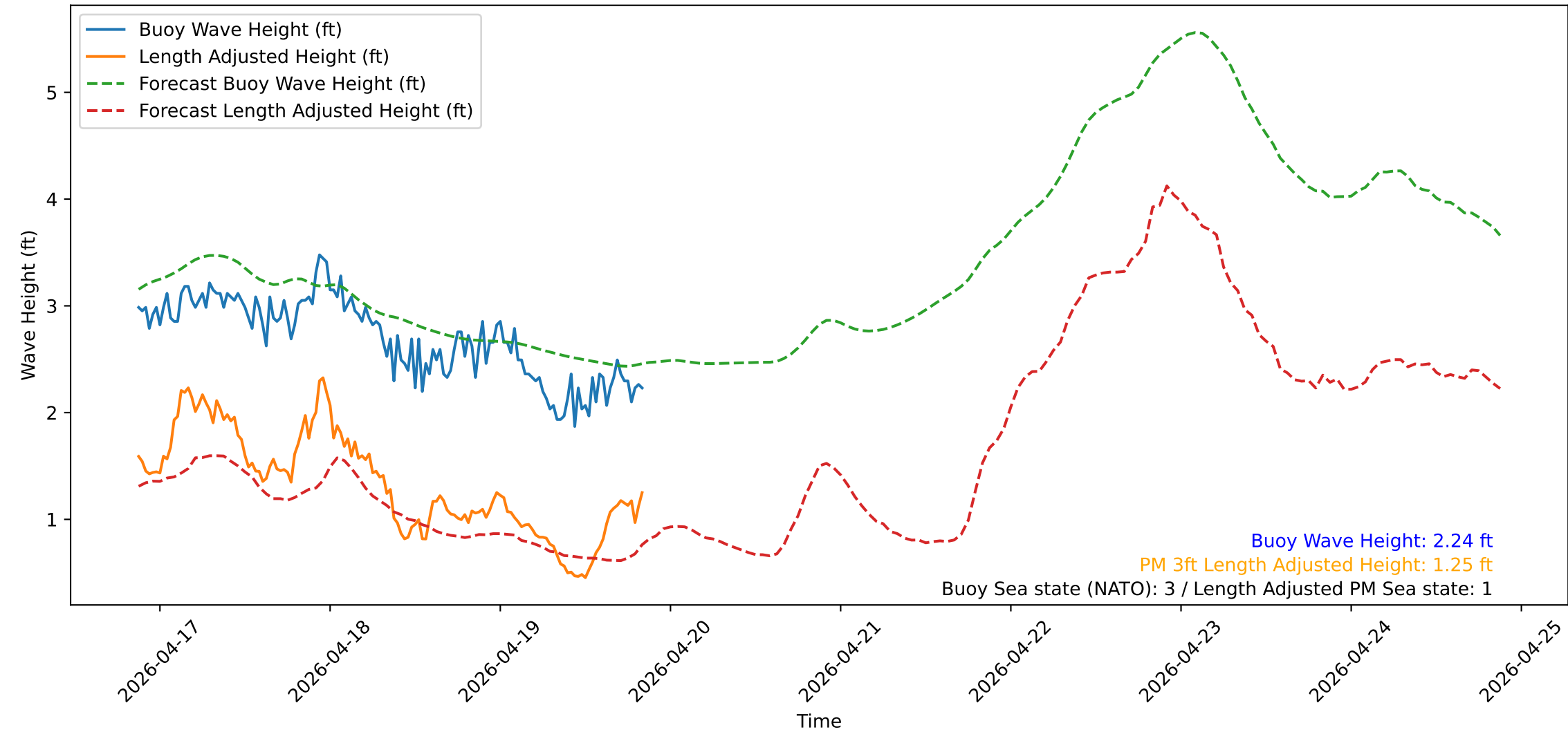
Wave Heights over Time for Green Beach at 2026-04-19 21:01:11
