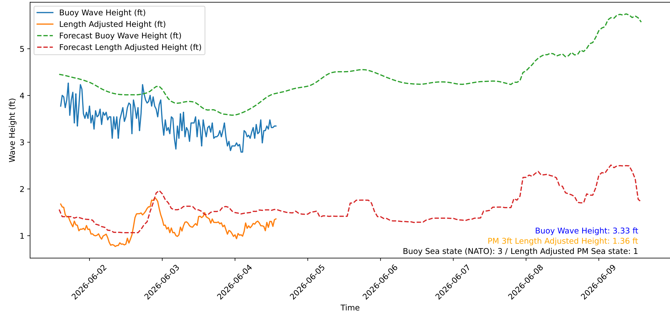
Wave Heights over Time for Green Beach at 2026-06-04 14:21:09
