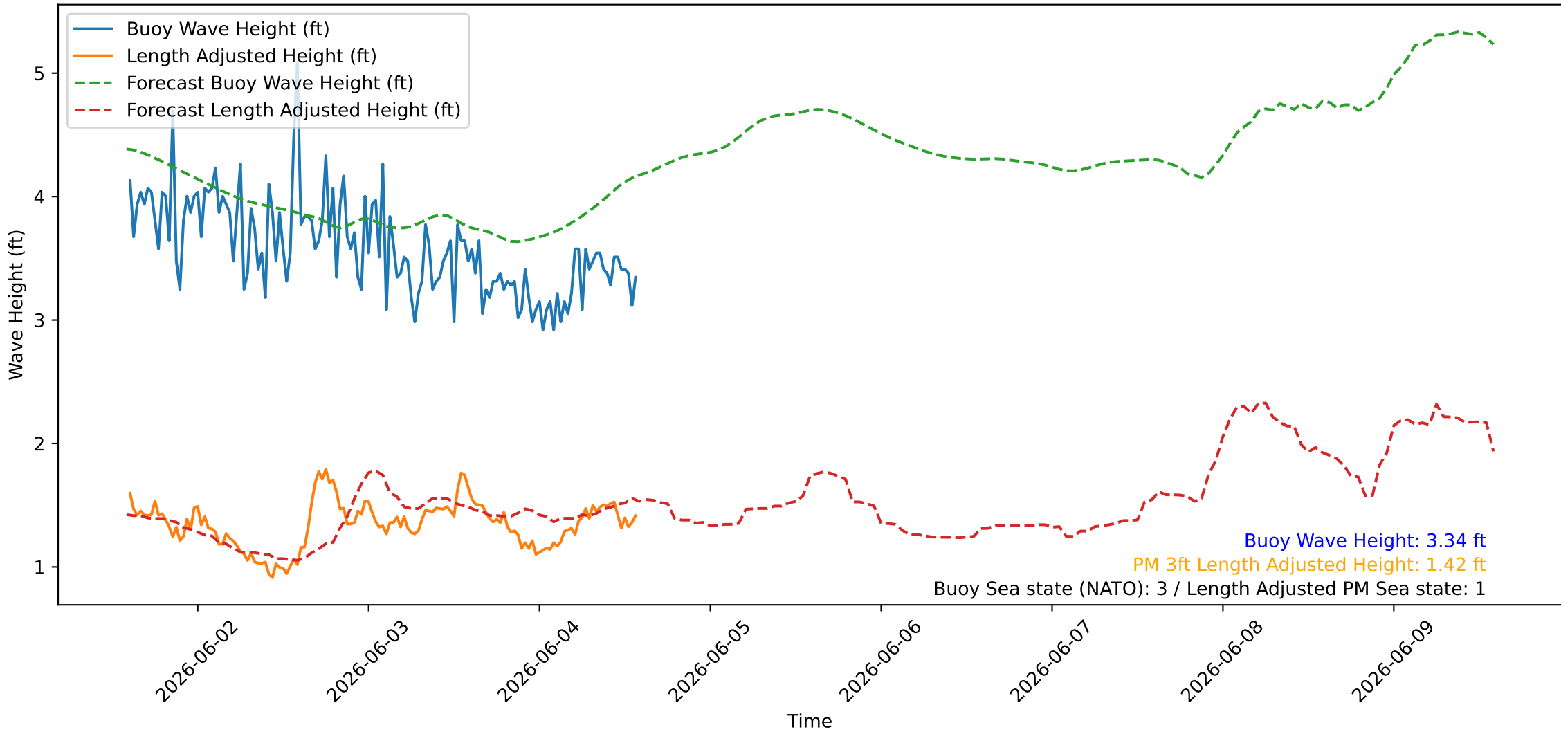
Wave Heights over Time for Oceanside Harbor at 2026-06-04 14:20:26
