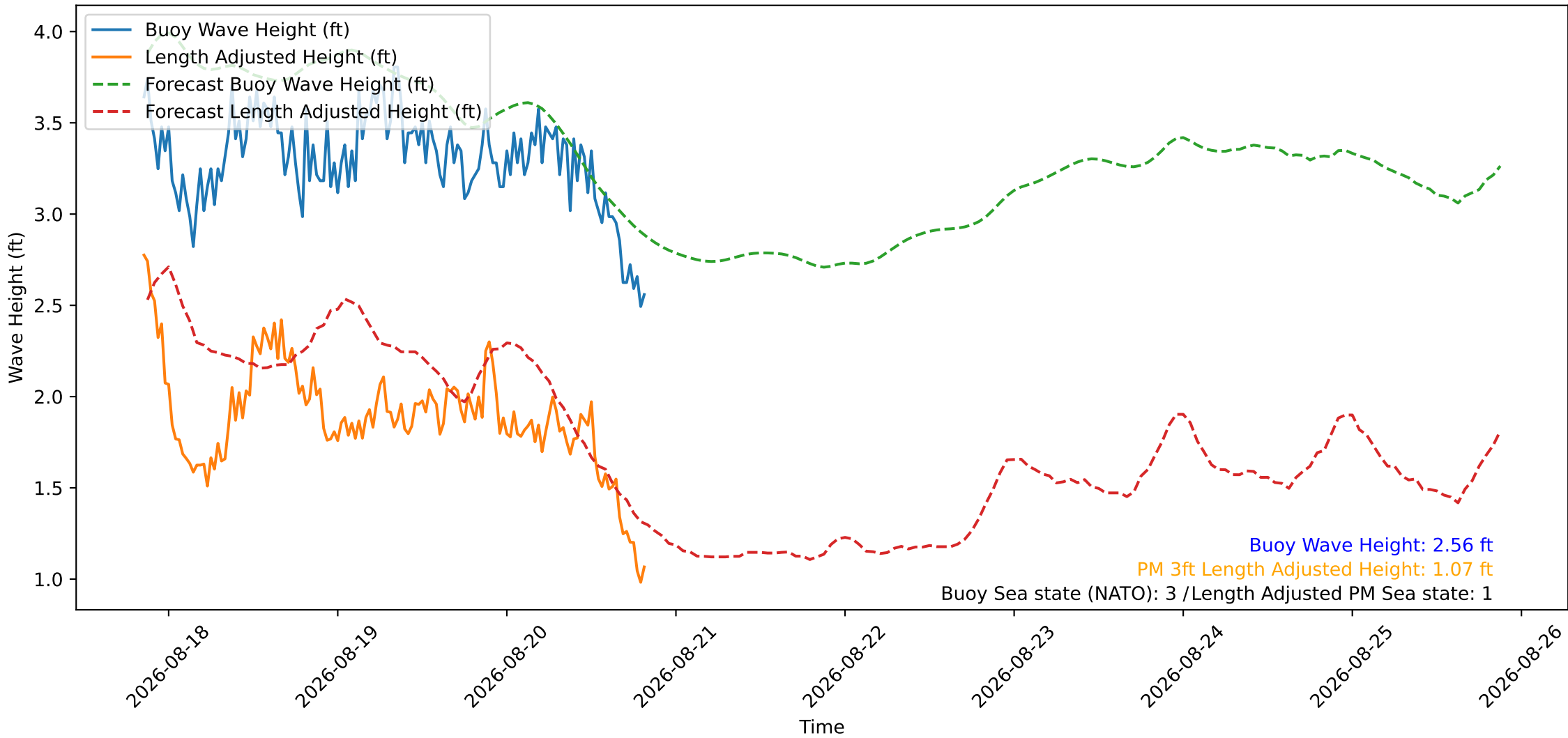
Wave Heights over Time for Oceanside Harbor at 2026-08-20 20:30:26
