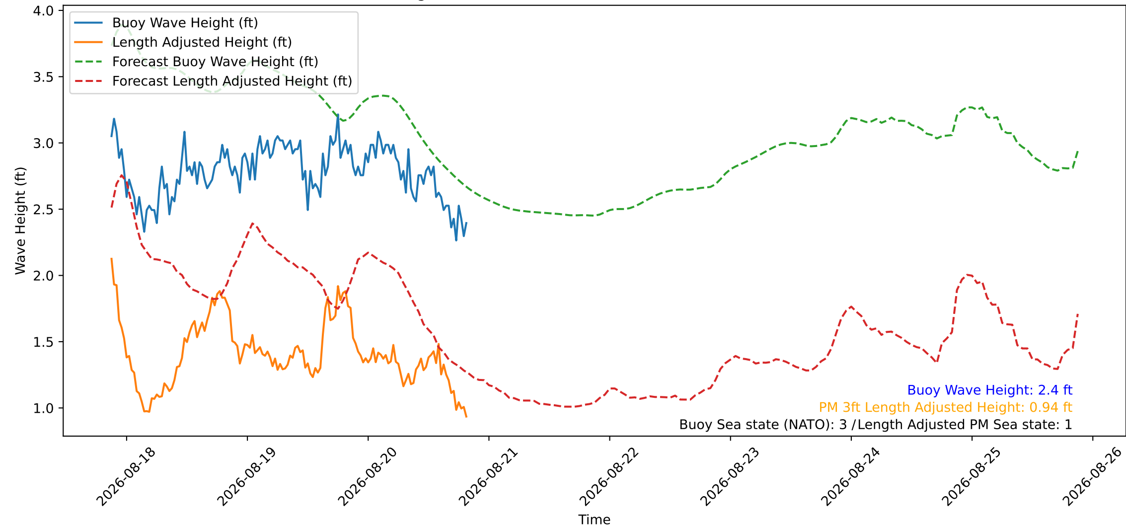
Wave Heights over Time for Red Beach at 2026-08-20 20:30:46
