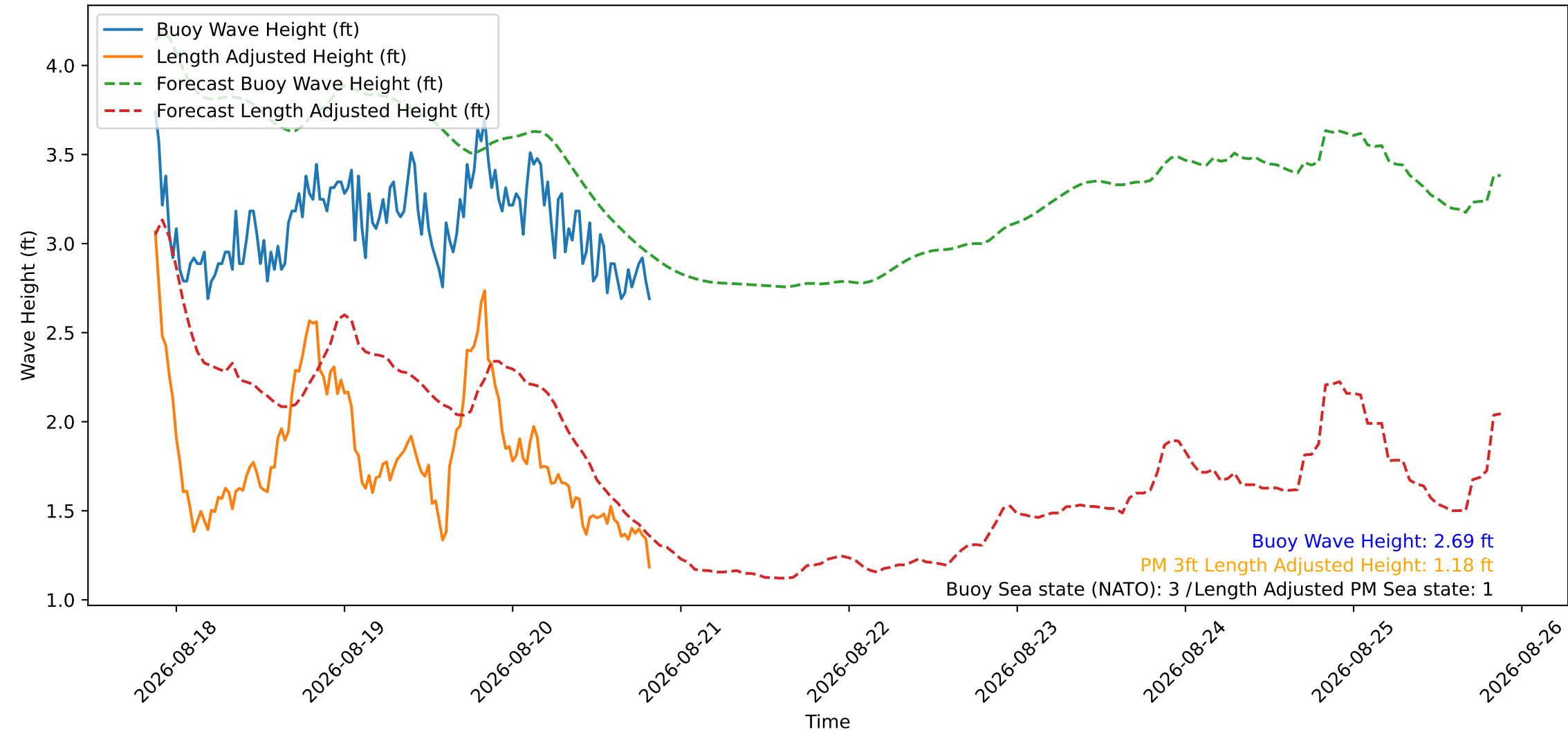
Wave Heights over Time for Green Beach at 2026-08-20 20:31:08
