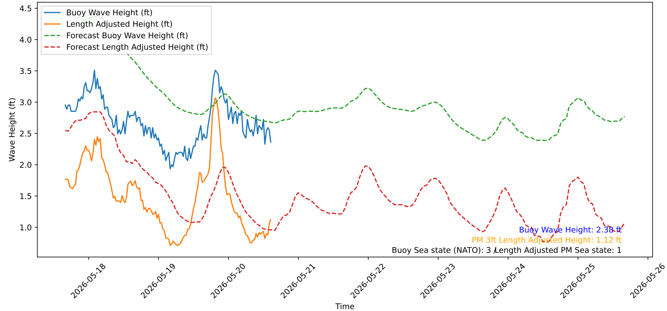
Wave Heights over Time for Red Beach at 2026-05-20 15:30:51
