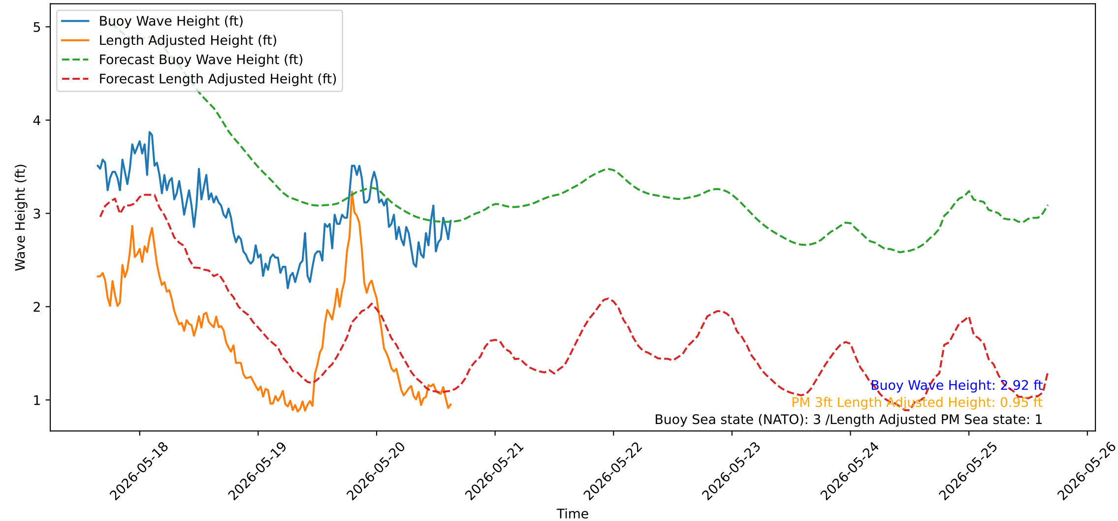
Wave Heights over Time for Oceanside Harbor at 2026-05-20 15:30:31
