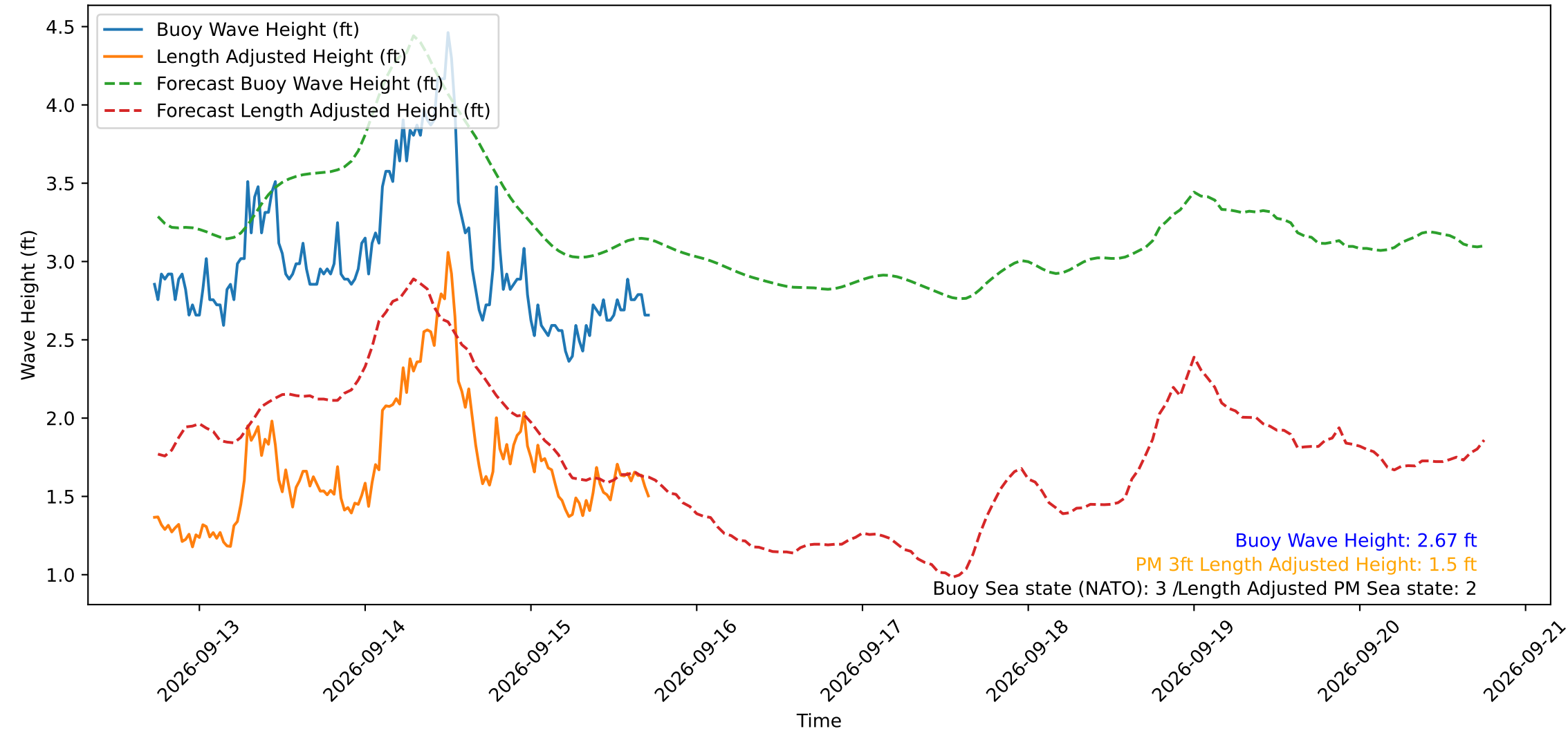
Wave Heights over Time for Oceanside Harbor at 2026-09-15 17:30:30
