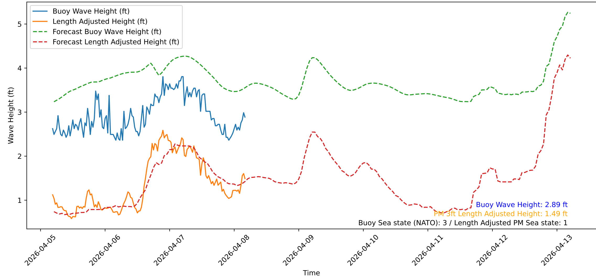
Wave Heights over Time for Green Beach at 2026-04-08 04:41:10
