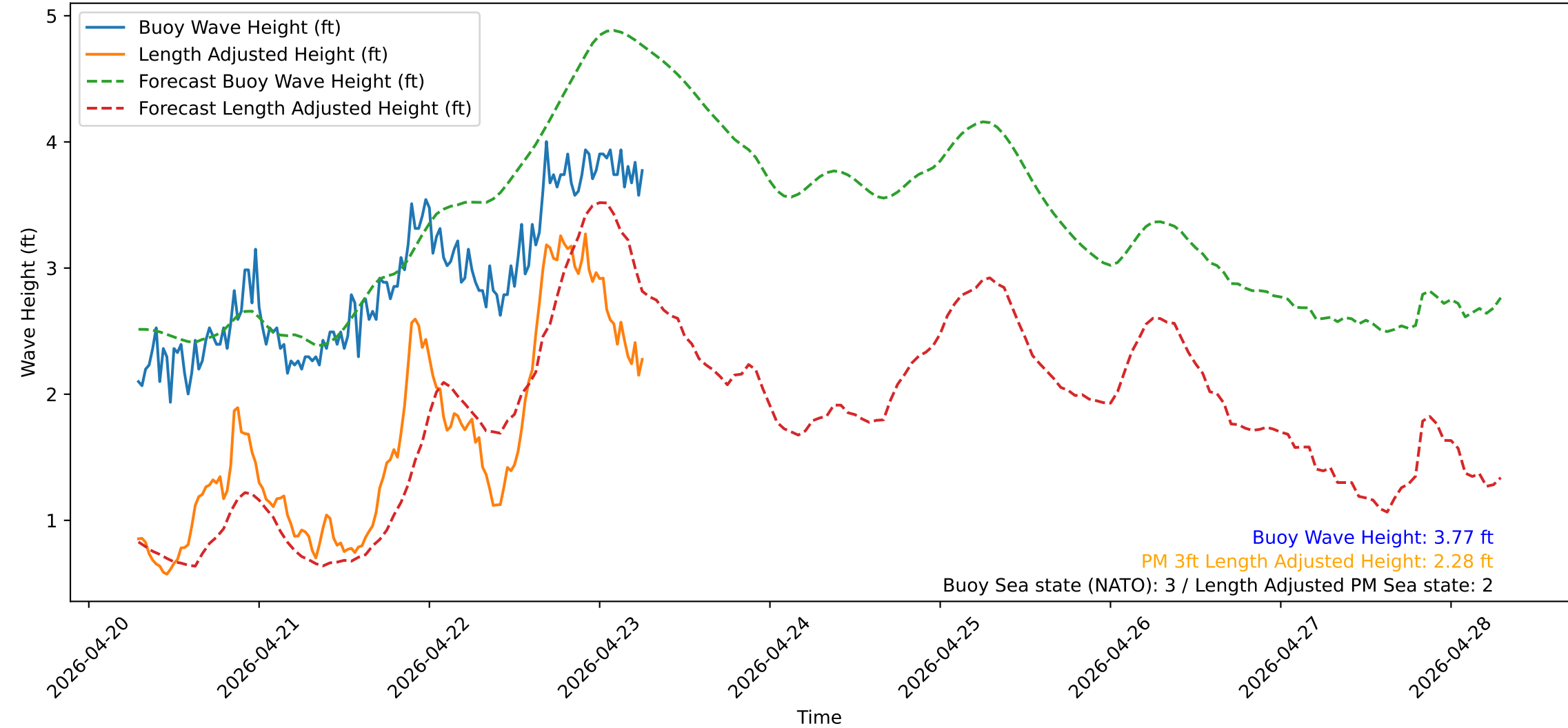
Wave Heights over Time for Green Beach at 2026-04-23 06:51:13
