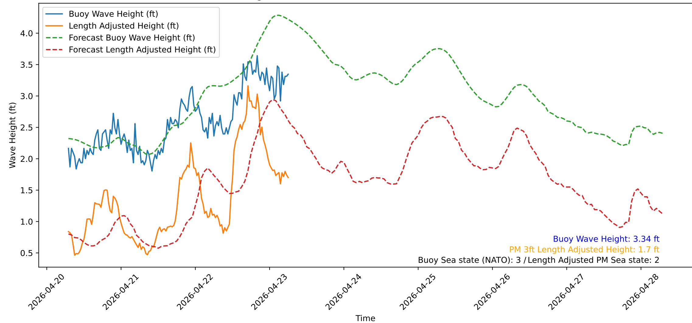
Wave Heights over Time for Red Beach at 2026-04-23 06:50:51
