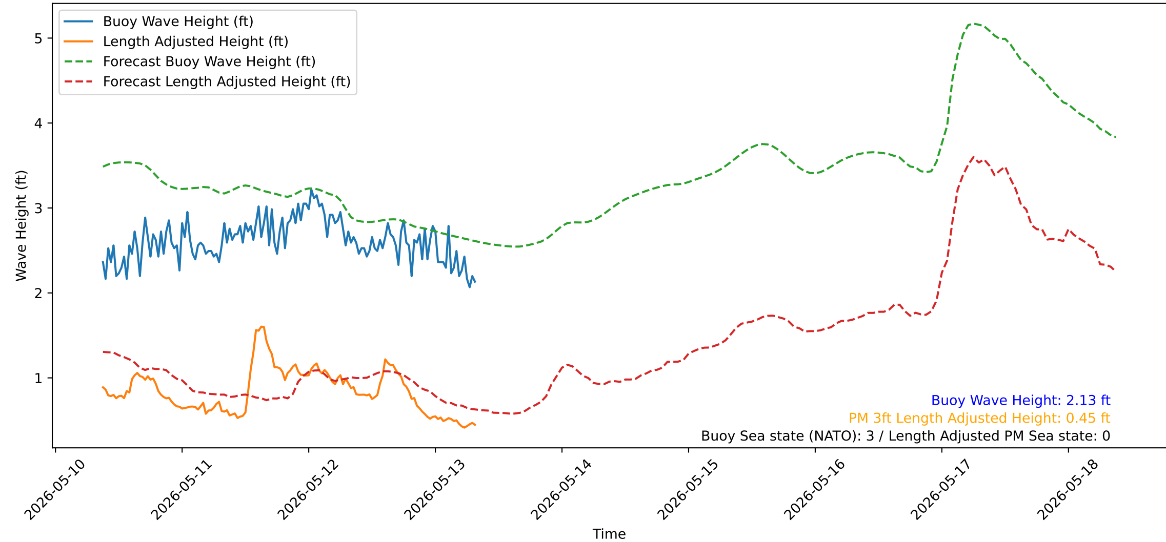
Wave Heights over Time for Red Beach at 2026-05-13 08:30:52
