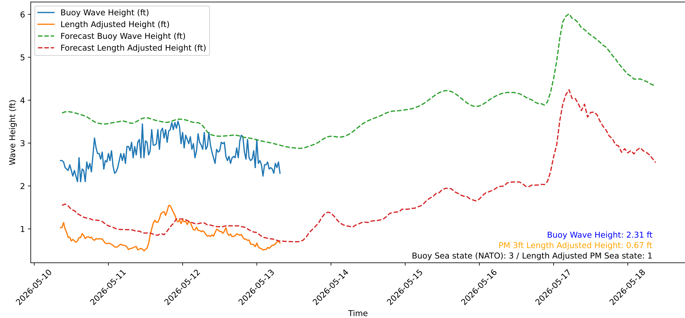
Wave Heights over Time for Green Beach at 2026-05-13 08:31:14
