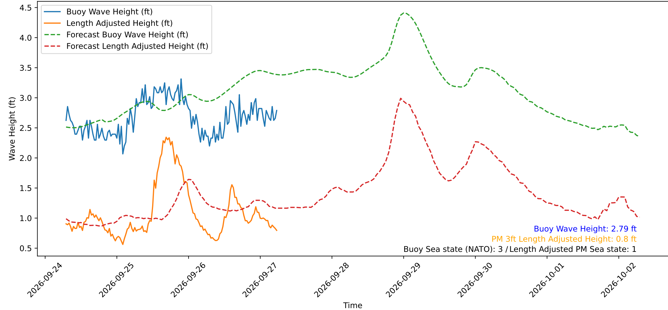
Wave Heights over Time for Red Beach at 2026-09-27 06:30:49
