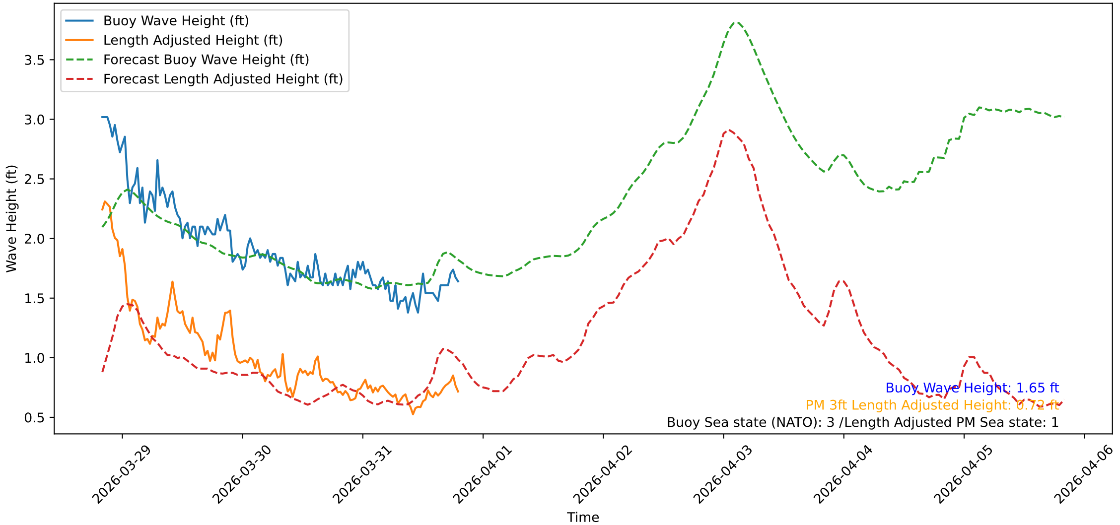
Wave Heights over Time for Red Beach at 2026-03-31 19:40:47
