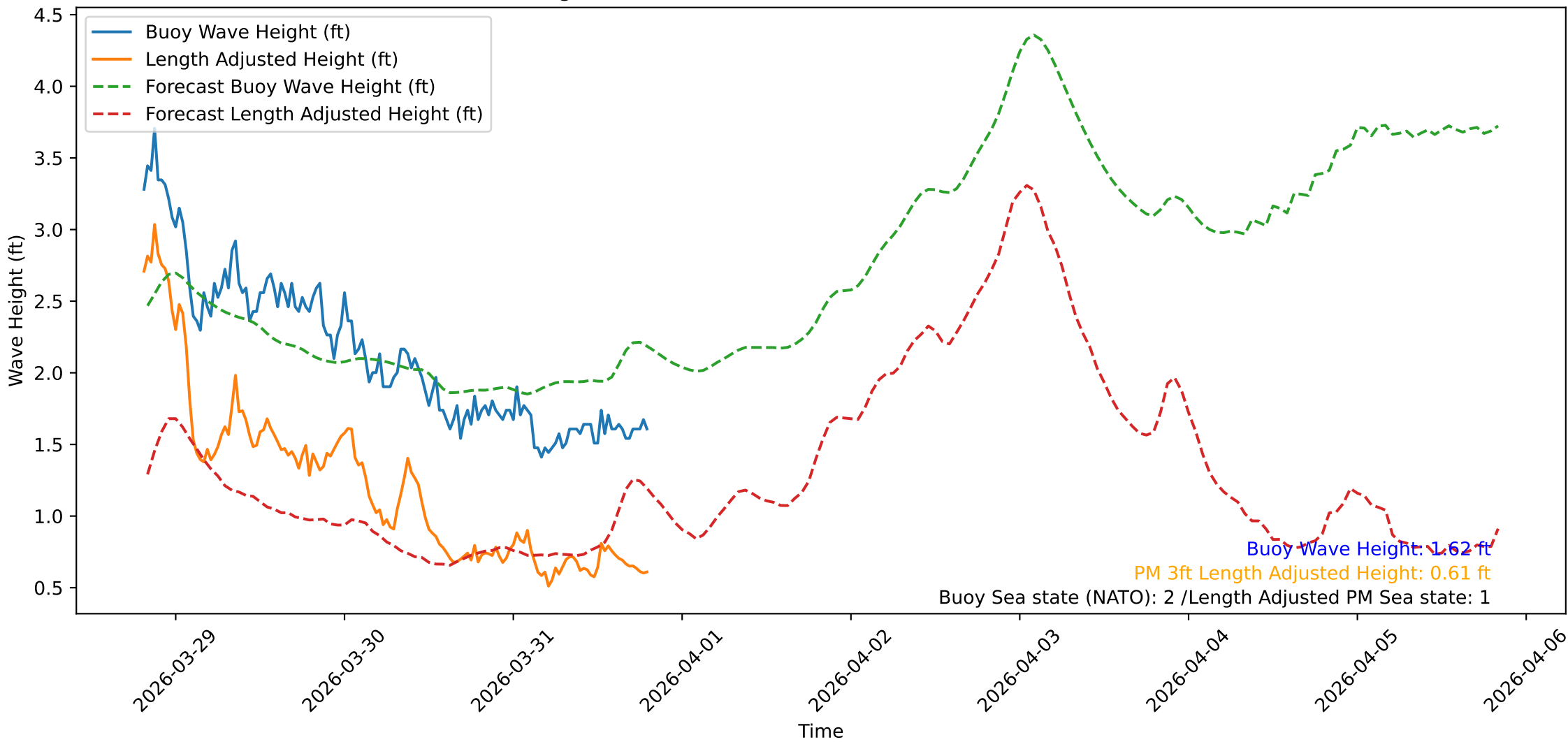
Wave Heights over Time for Green Beach at 2026-03-31 19:41:10
