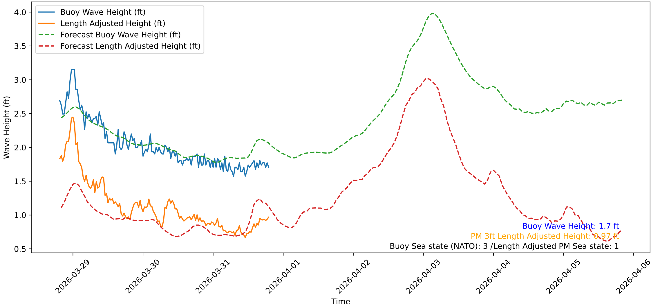
Wave Heights over Time for Oceanside Harbor at 2026-03-31 19:40:31
