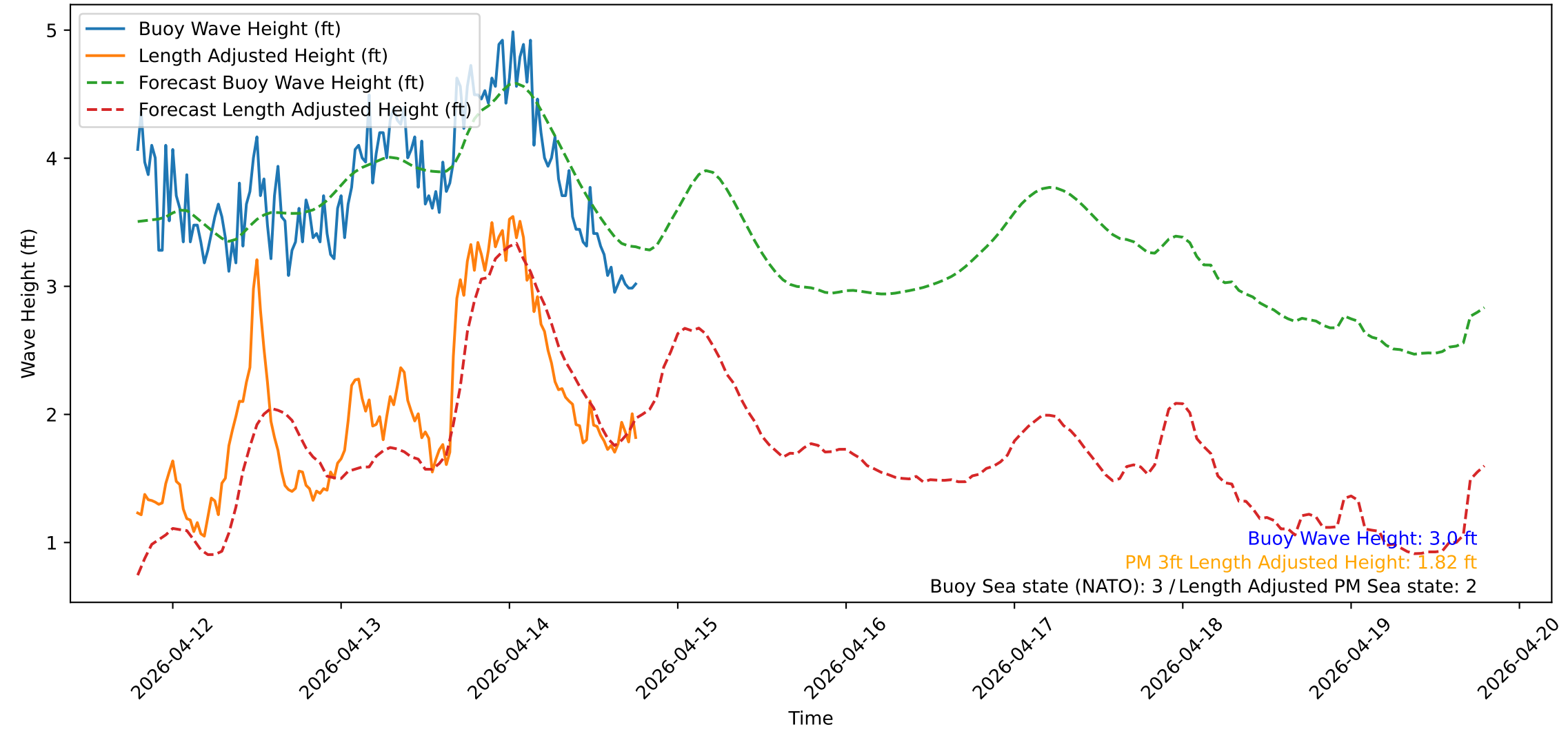
Wave Heights over Time for Green Beach at 2026-04-14 19:01:13
