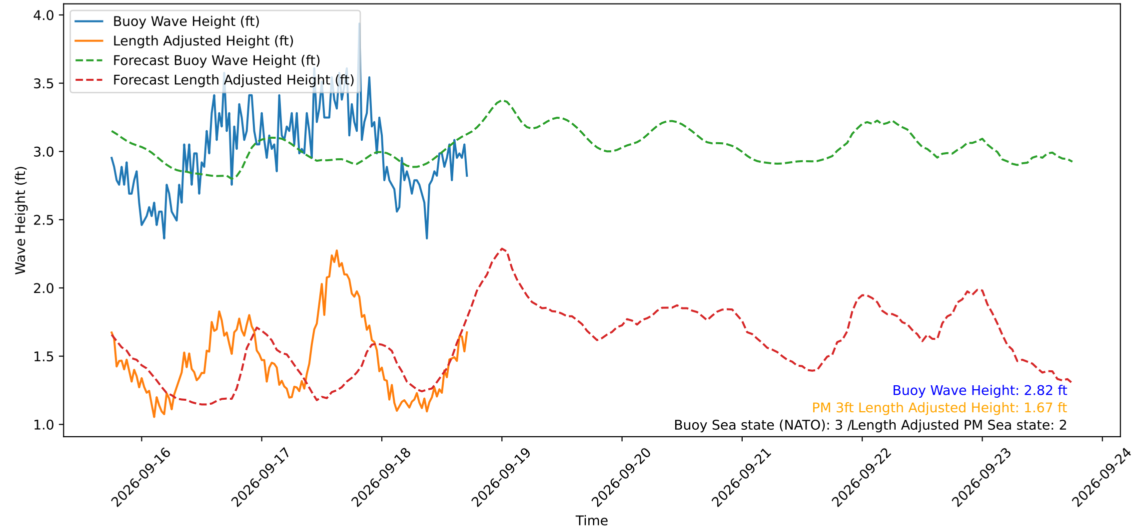
Wave Heights over Time for Oceanside Harbor at 2026-09-18 18:00:30
