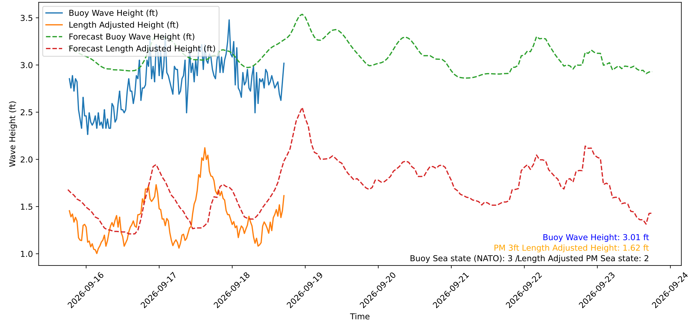
Wave Heights over Time for Green Beach at 2026-09-18 18:01:12
