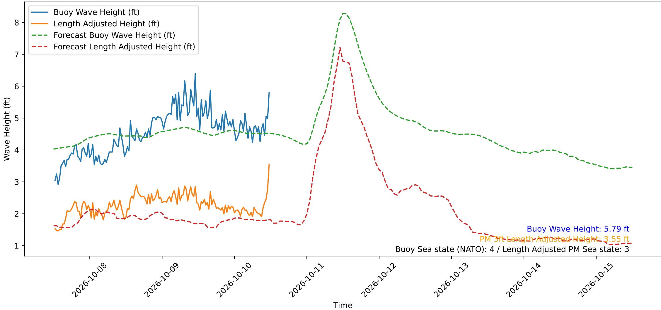
Wave Heights over Time for Oceanside Harbor at 2026-10-10 12:20:29
