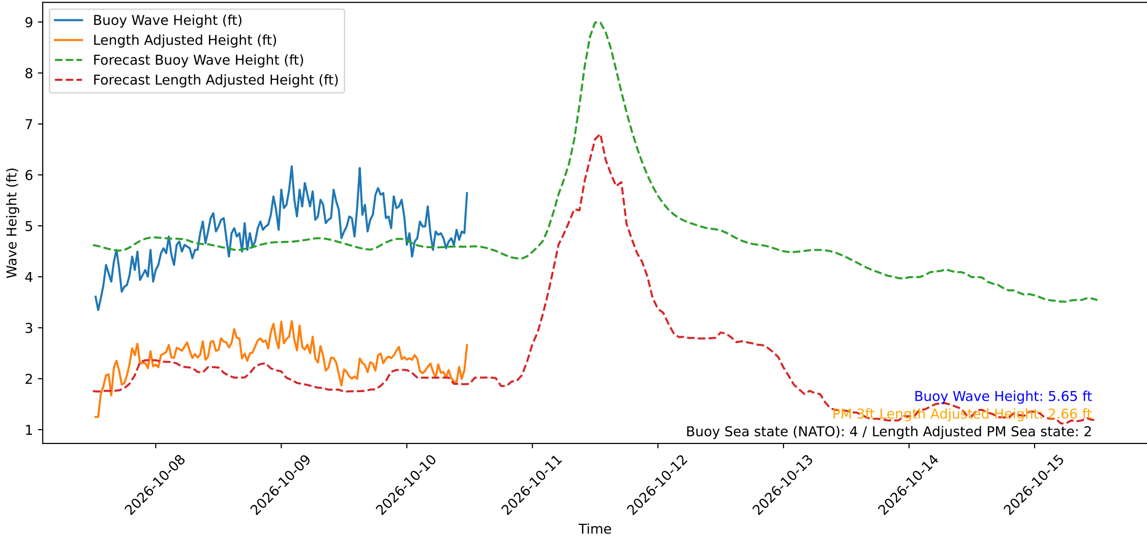
Wave Heights over Time for Green Beach at 2026-10-10 12:21:14
