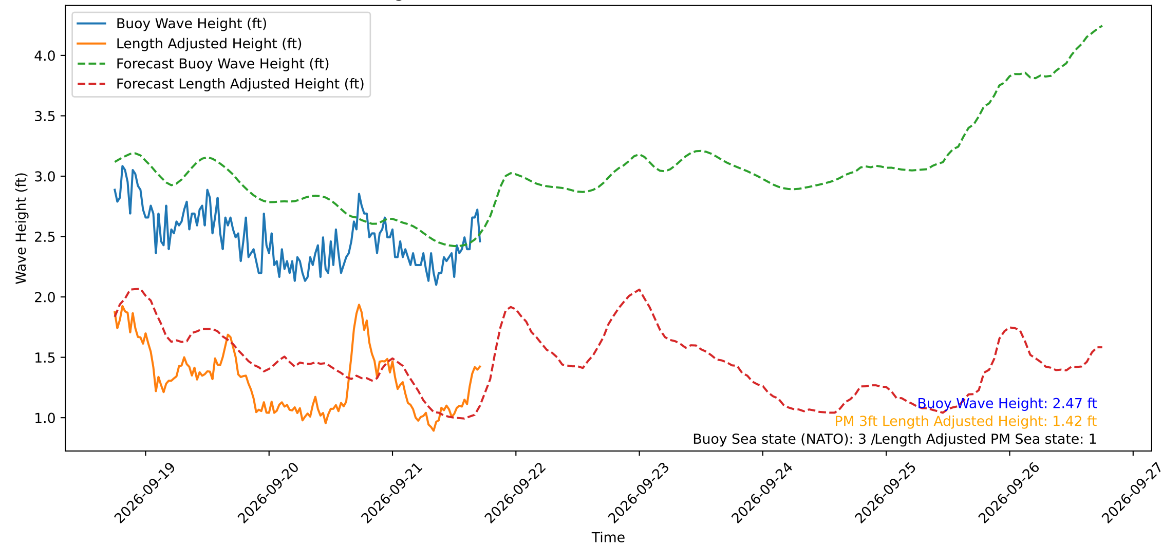
Wave Heights over Time for Oceanside Harbor at 2026-09-21 18:00:30
