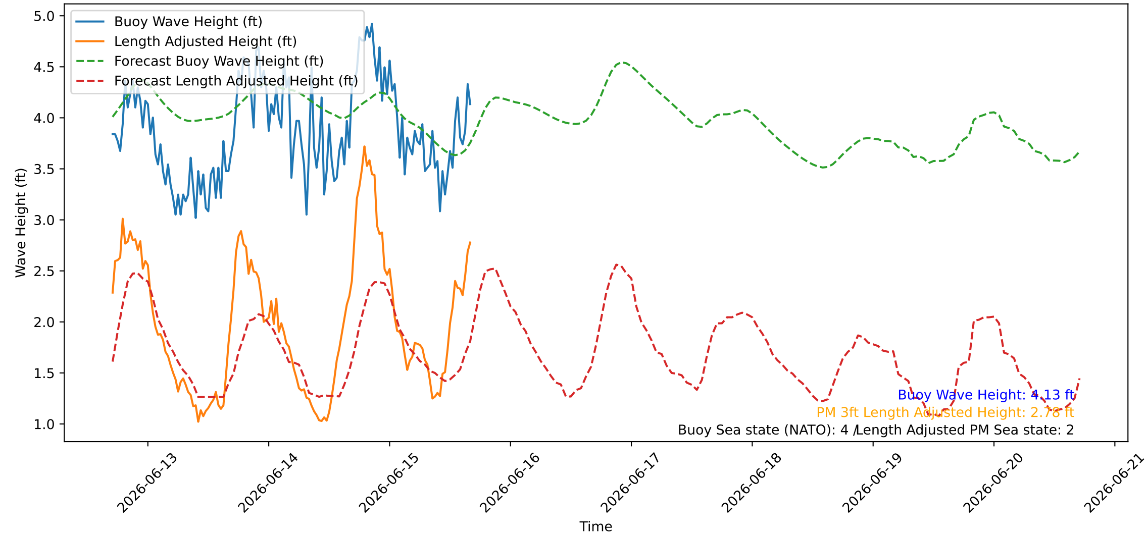
Wave Heights over Time for Green Beach at 2026-06-15 17:01:07
