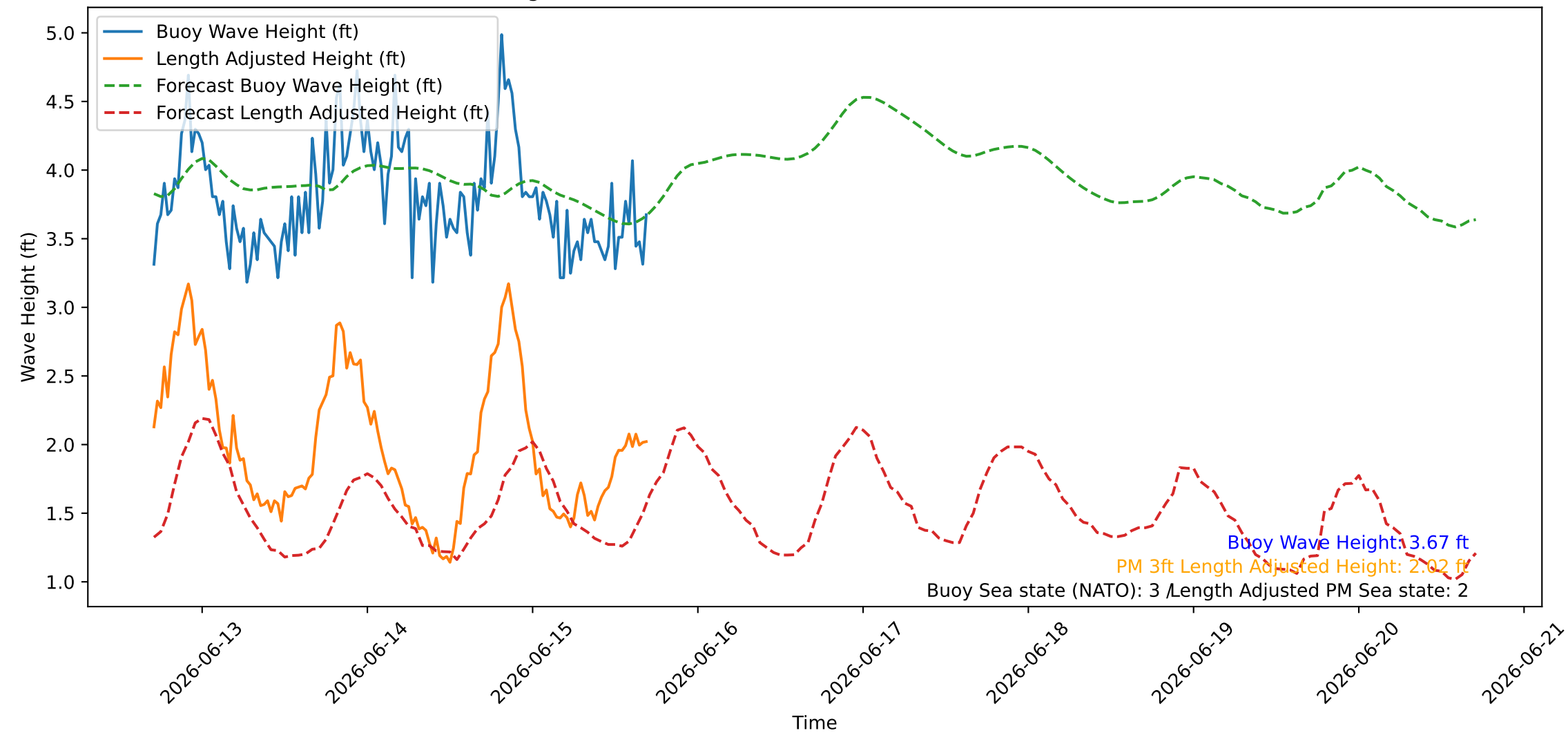
Wave Heights over Time for Oceanside Harbor at 2026-06-15 17:00:26
