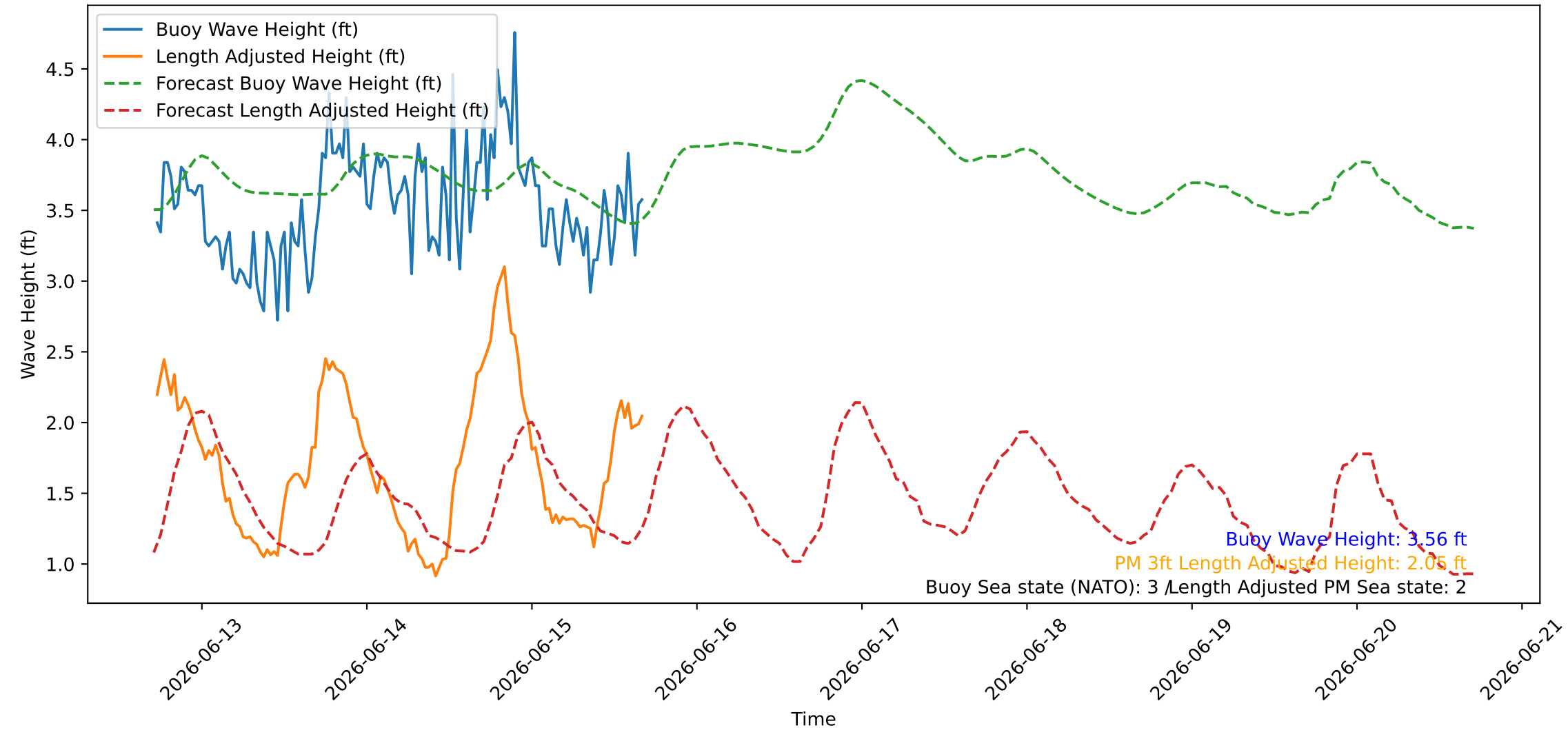
Wave Heights over Time for Red Beach at 2026-06-15 17:00:45
