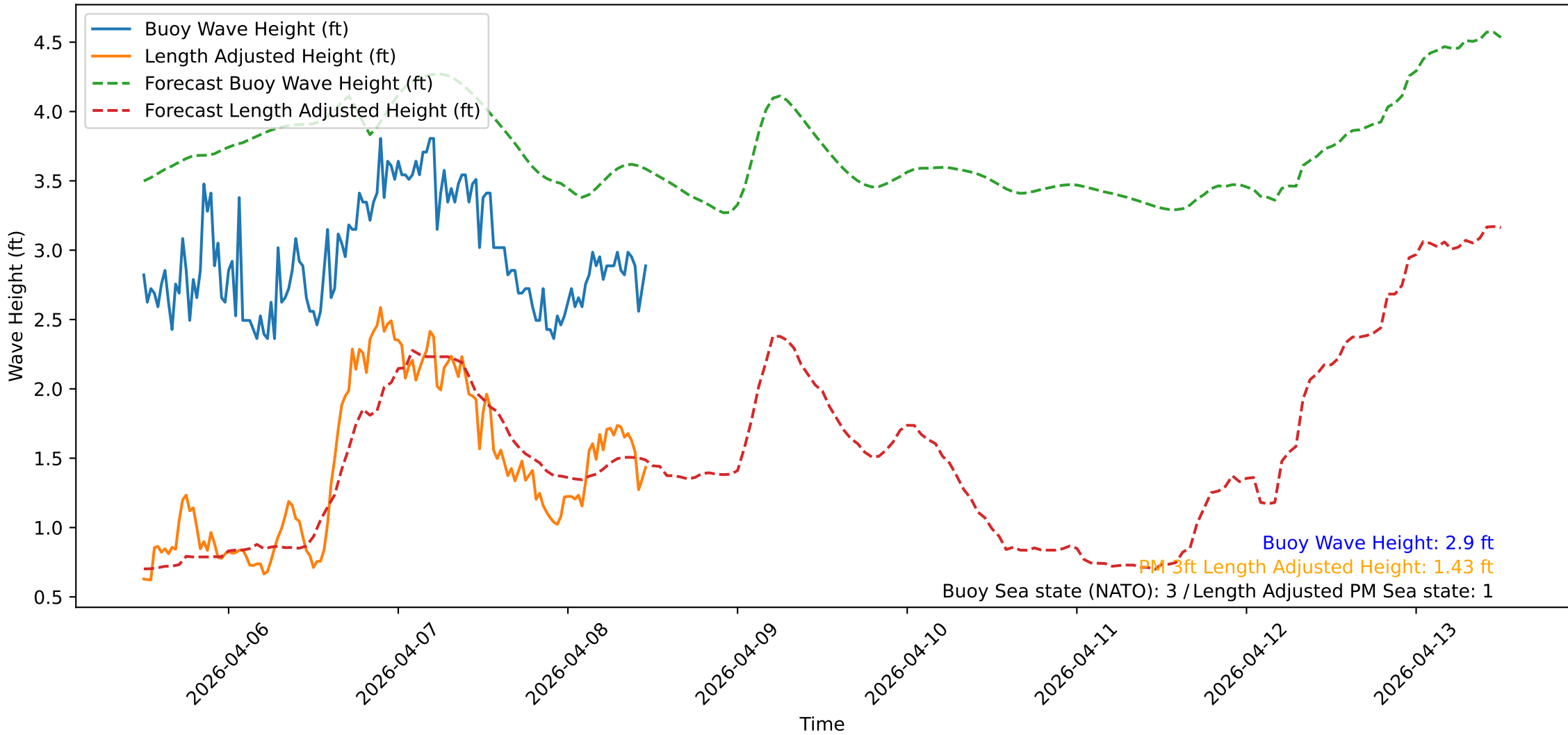
Wave Heights over Time for Green Beach at 2026-04-08 11:51:10
