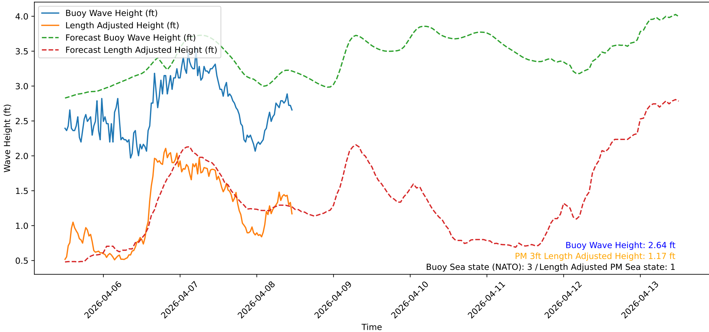
Wave Heights over Time for Red Beach at 2026-04-08 11:50:48
