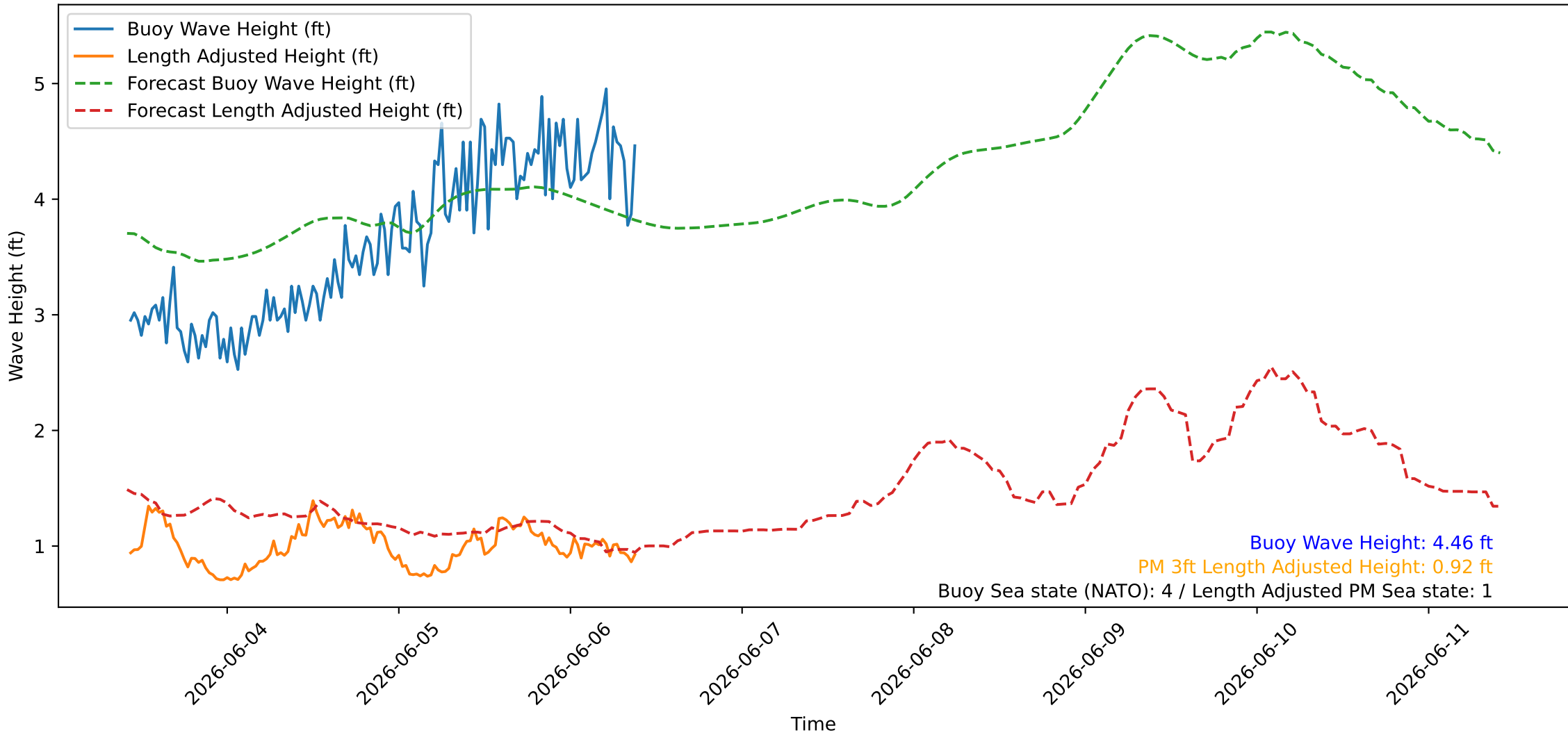
Wave Heights over Time for Red Beach at 2026-06-06 10:00:45
