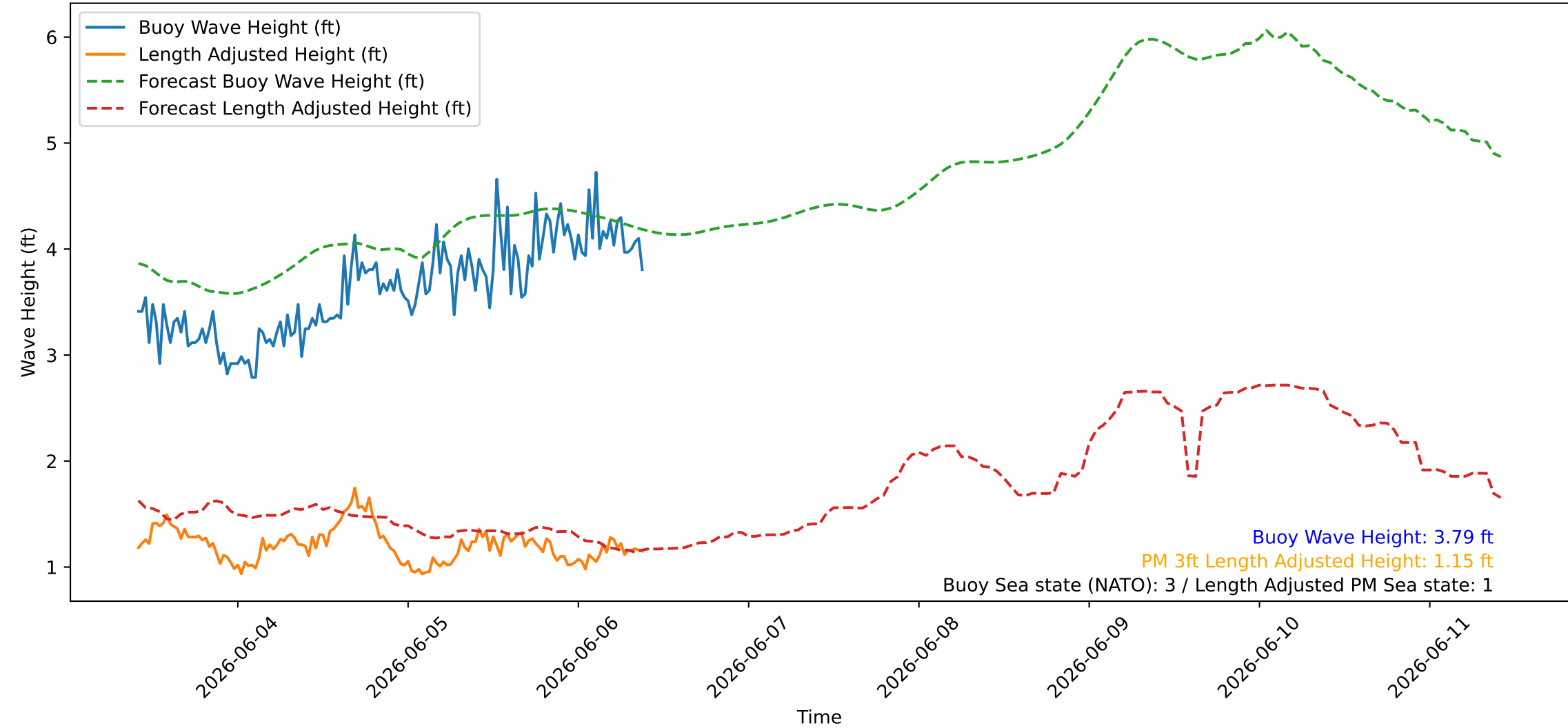
Wave Heights over Time for Green Beach at 2026-06-06 10:01:07
