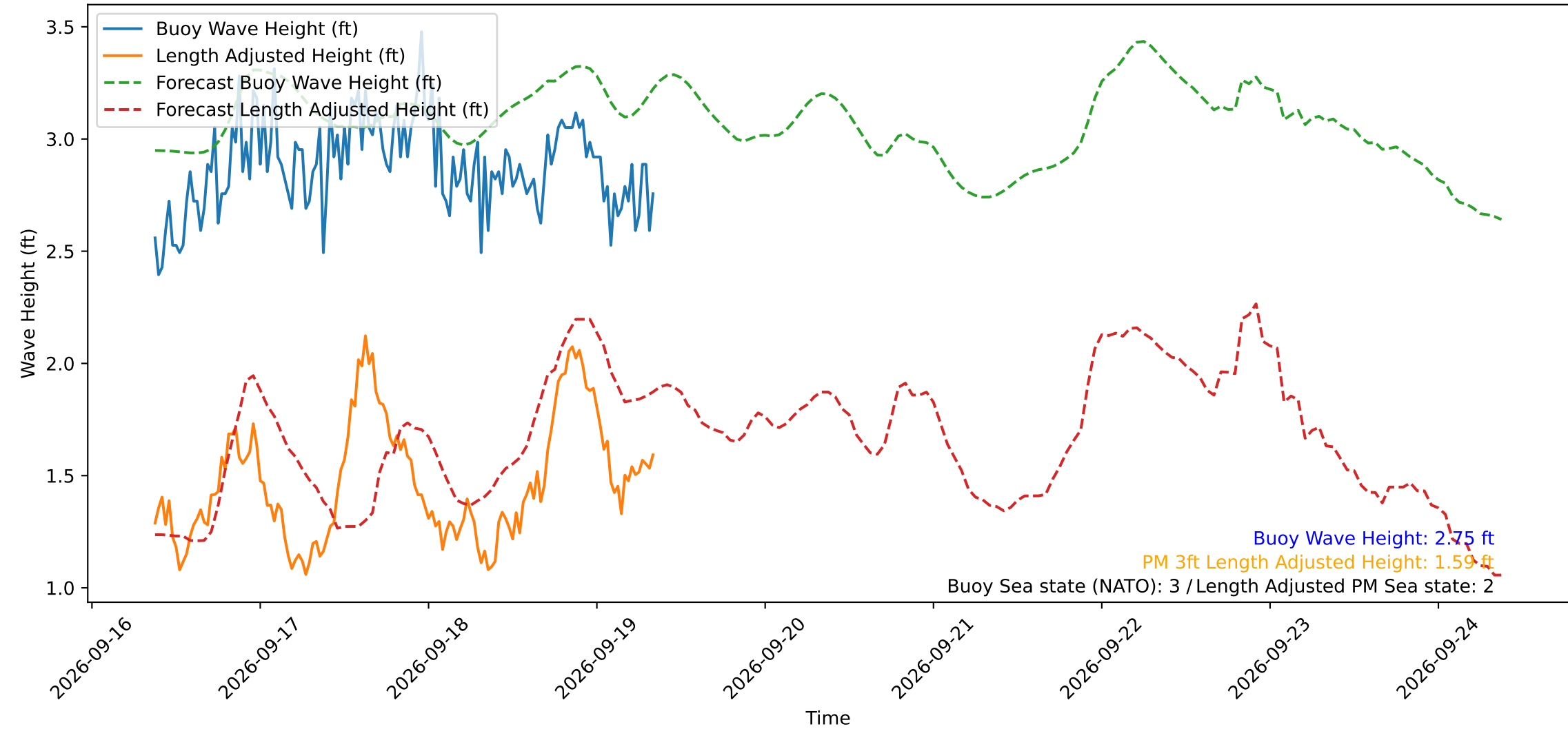
Wave Heights over Time for Green Beach at 2026-09-19 08:41:10
