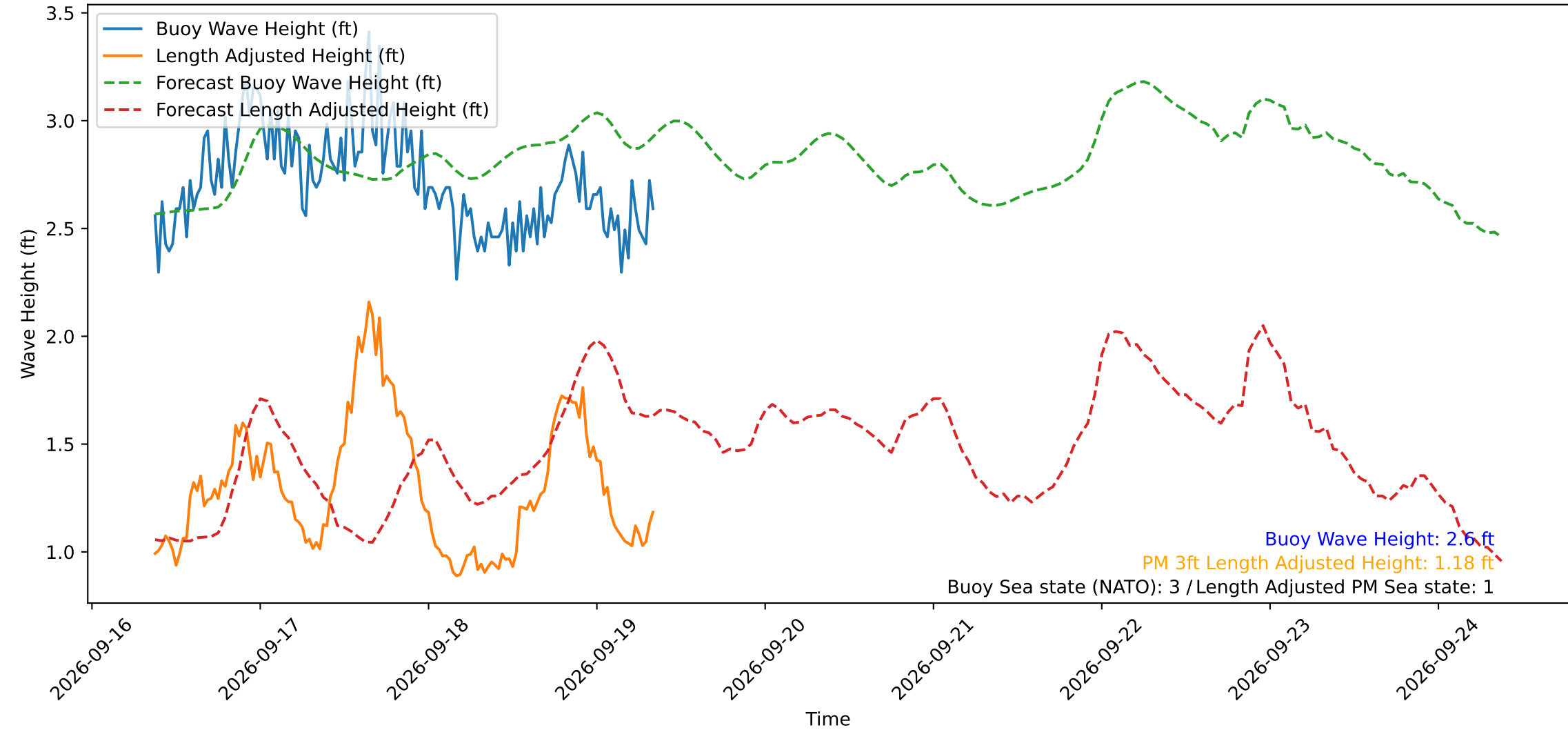
Wave Heights over Time for Red Beach at 2026-09-19 08:40:48
