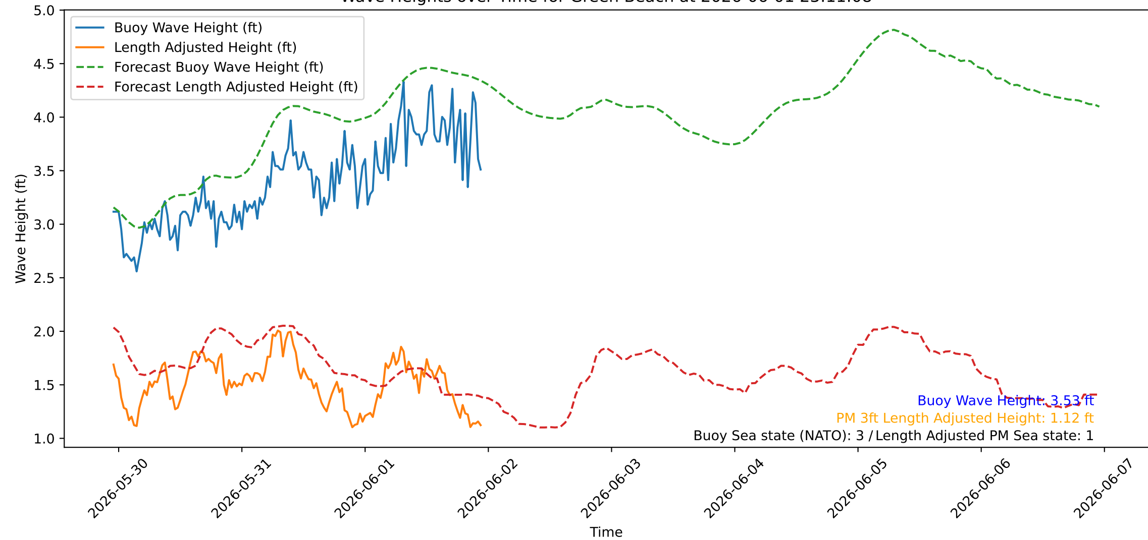
Wave Heights over Time for Green Beach at 2026-06-01 23:11:08
