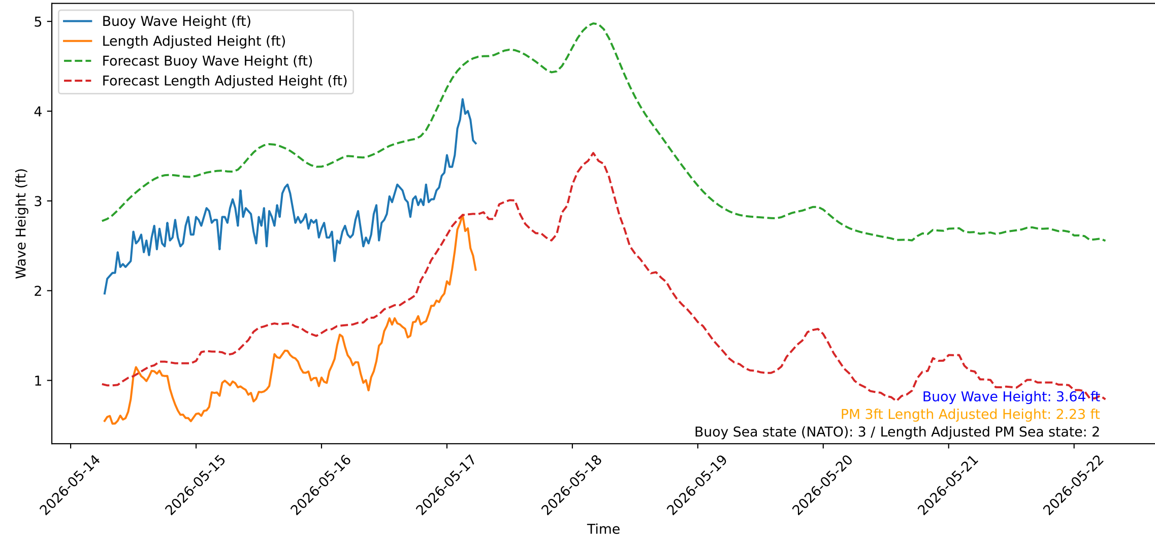
Wave Heights over Time for Red Beach at 2026-05-17 06:20:52
