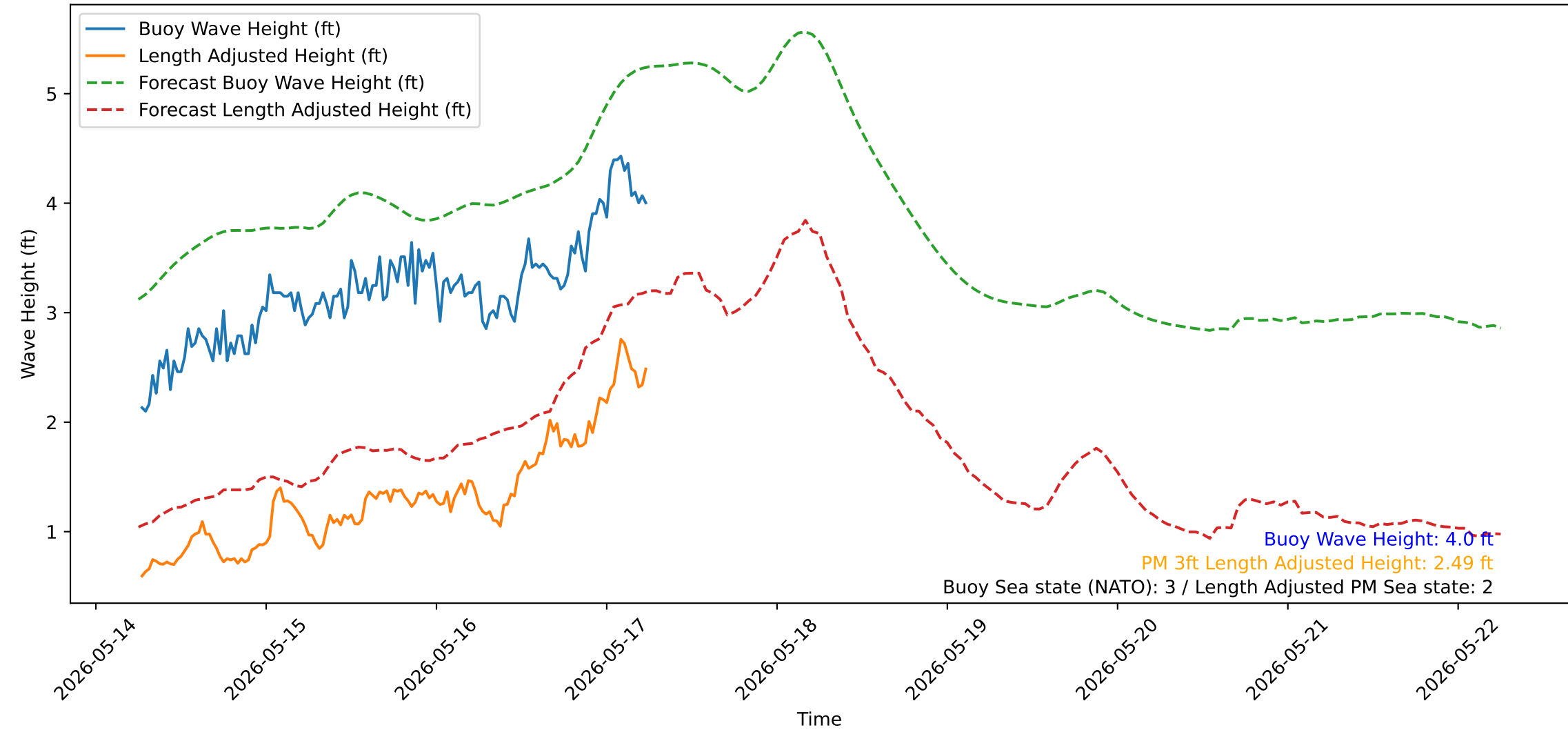
Wave Heights over Time for Green Beach at 2026-05-17 06:21:15
