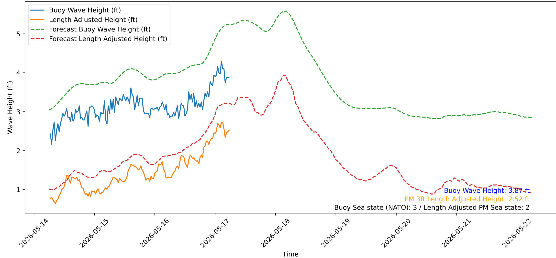
Wave Heights over Time for Oceanside Harbor at 2026-05-17 06:20:32
