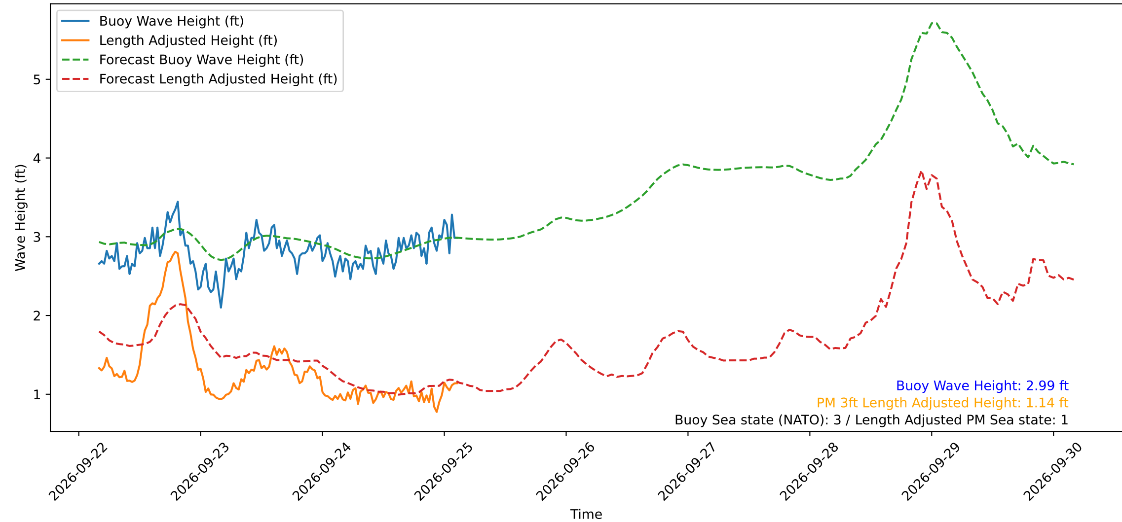
Wave Heights over Time for Green Beach at 2026-09-25 03:31:11
