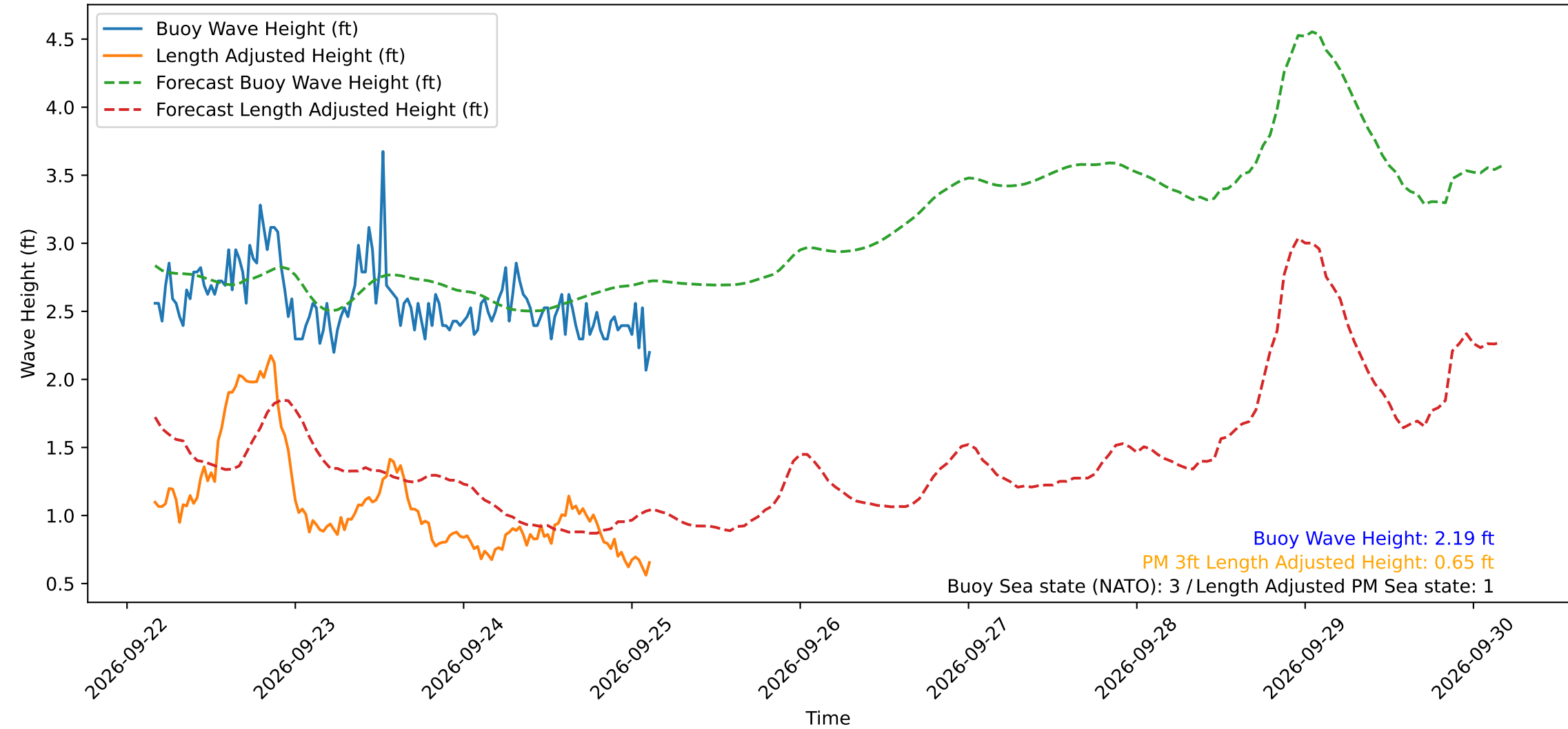
Wave Heights over Time for Red Beach at 2026-09-25 03:30:49
