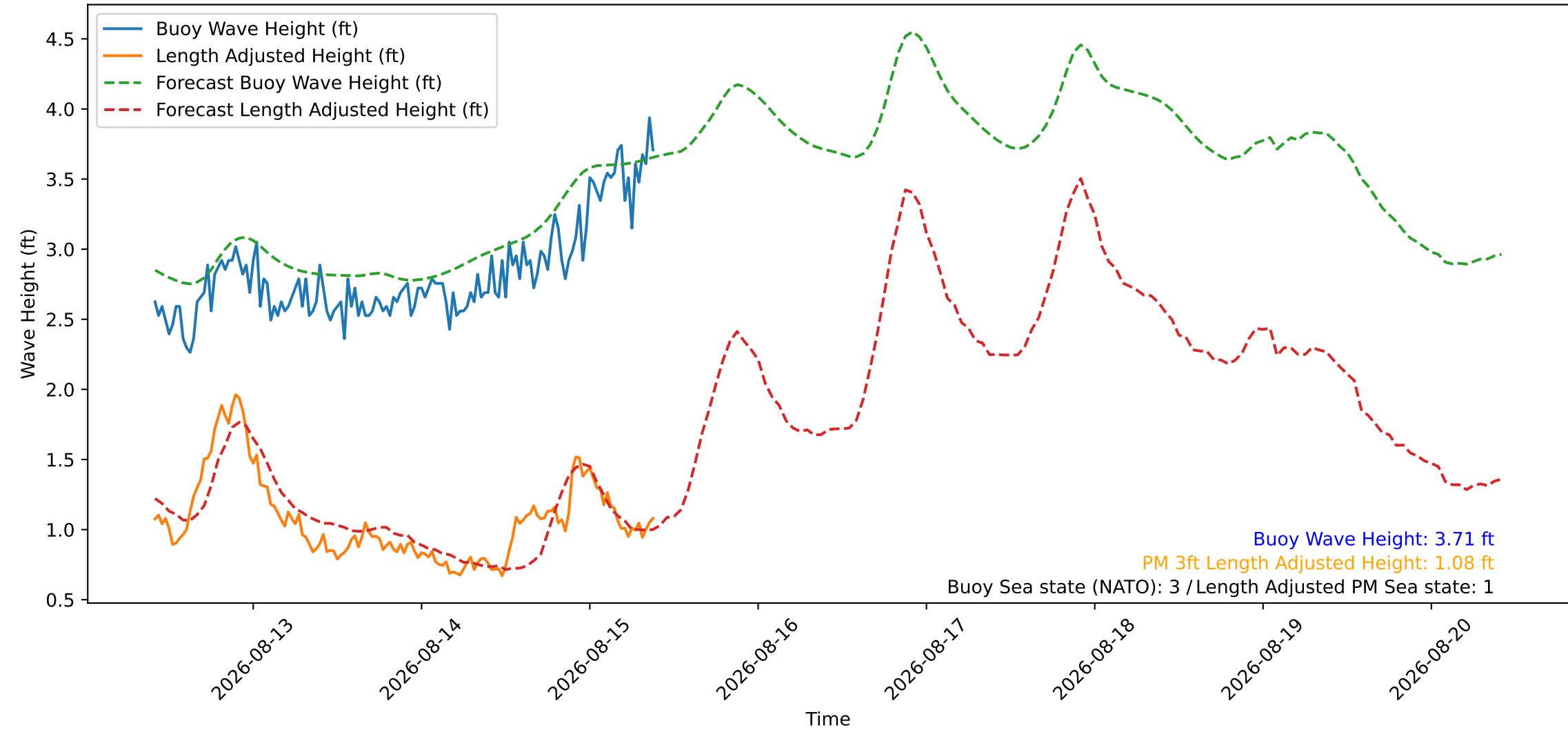
Wave Heights over Time for Green Beach at 2026-08-15 10:11:08
