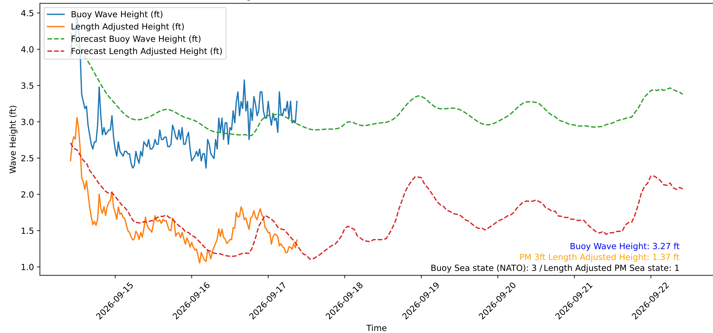
Wave Heights over Time for Oceanside Harbor at 2026-09-17 10:00:30
