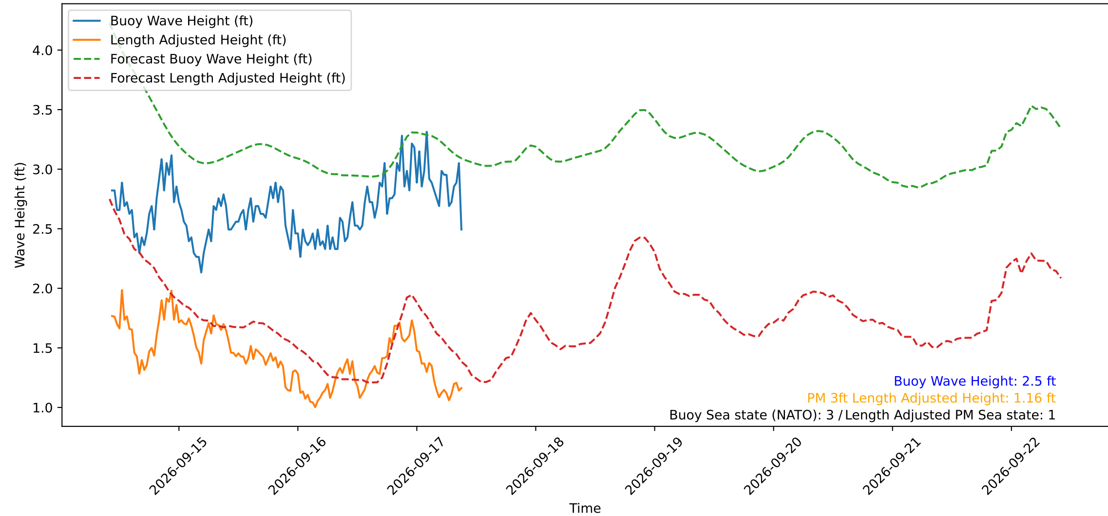
Wave Heights over Time for Green Beach at 2026-09-17 10:01:12
