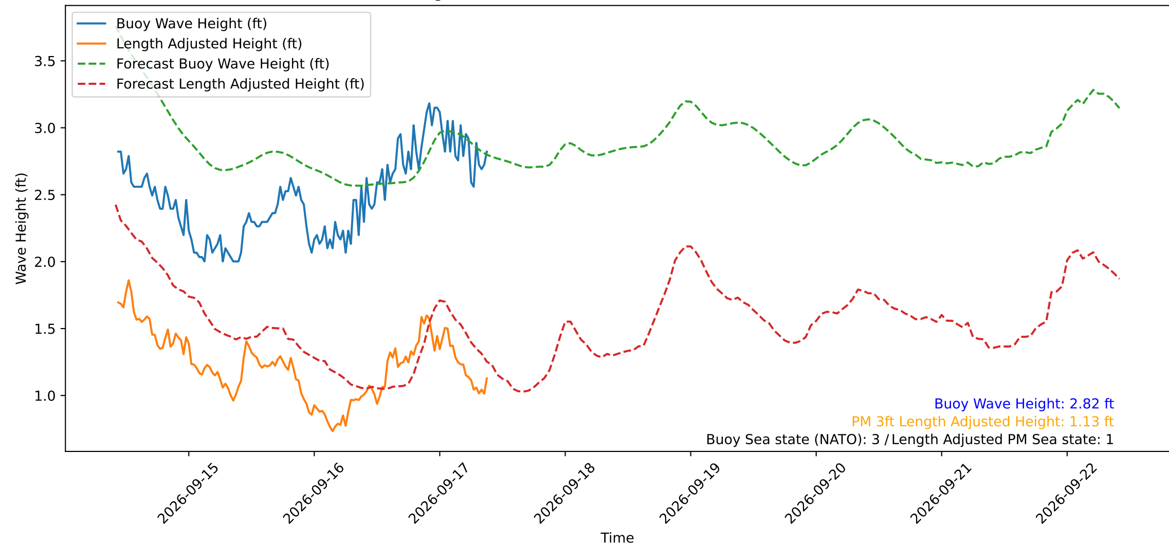
Wave Heights over Time for Red Beach at 2026-09-17 10:00:50
