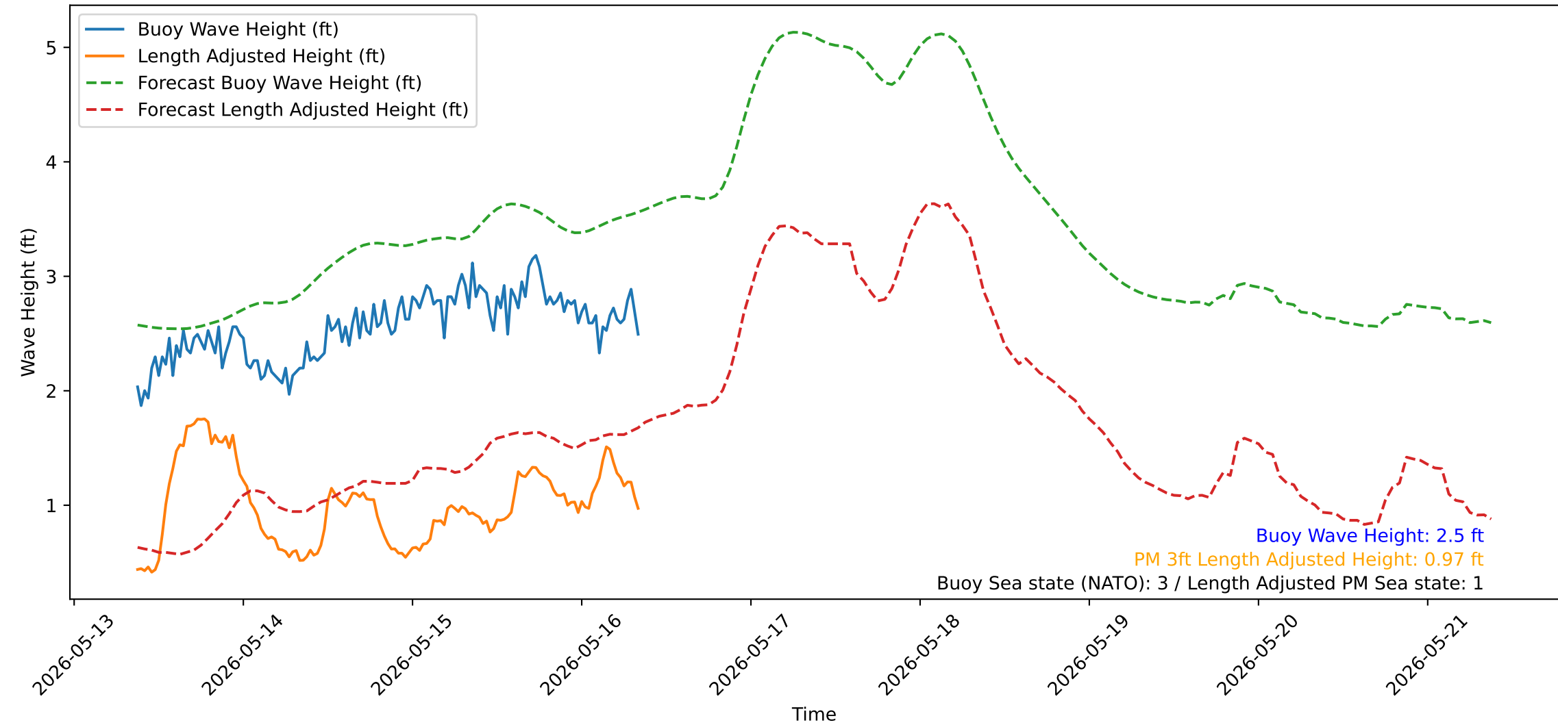
Wave Heights over Time for Red Beach at 2026-05-16 08:50:52
