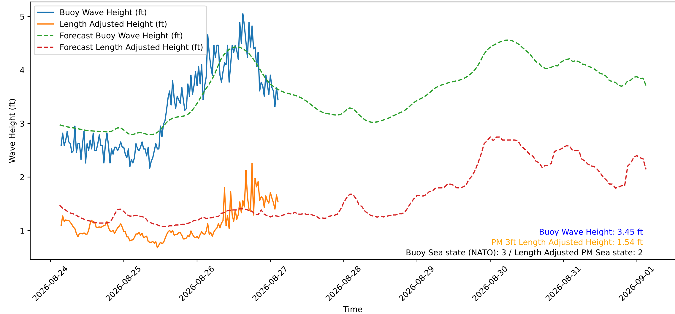
Wave Heights over Time for Red Beach at 2026-08-27 03:20:51
