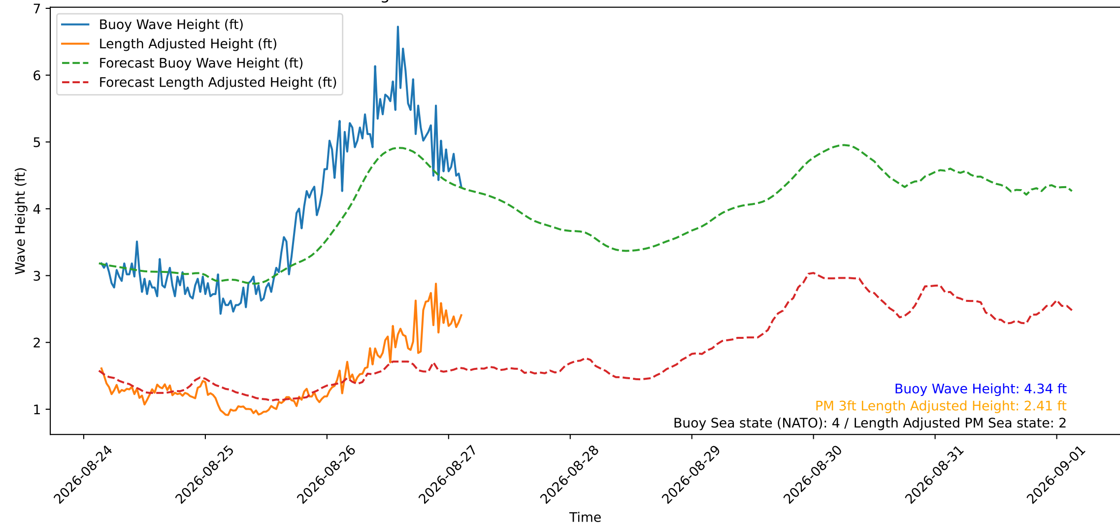
Wave Heights over Time for Oceanside Harbor at 2026-08-27 03:20:29
