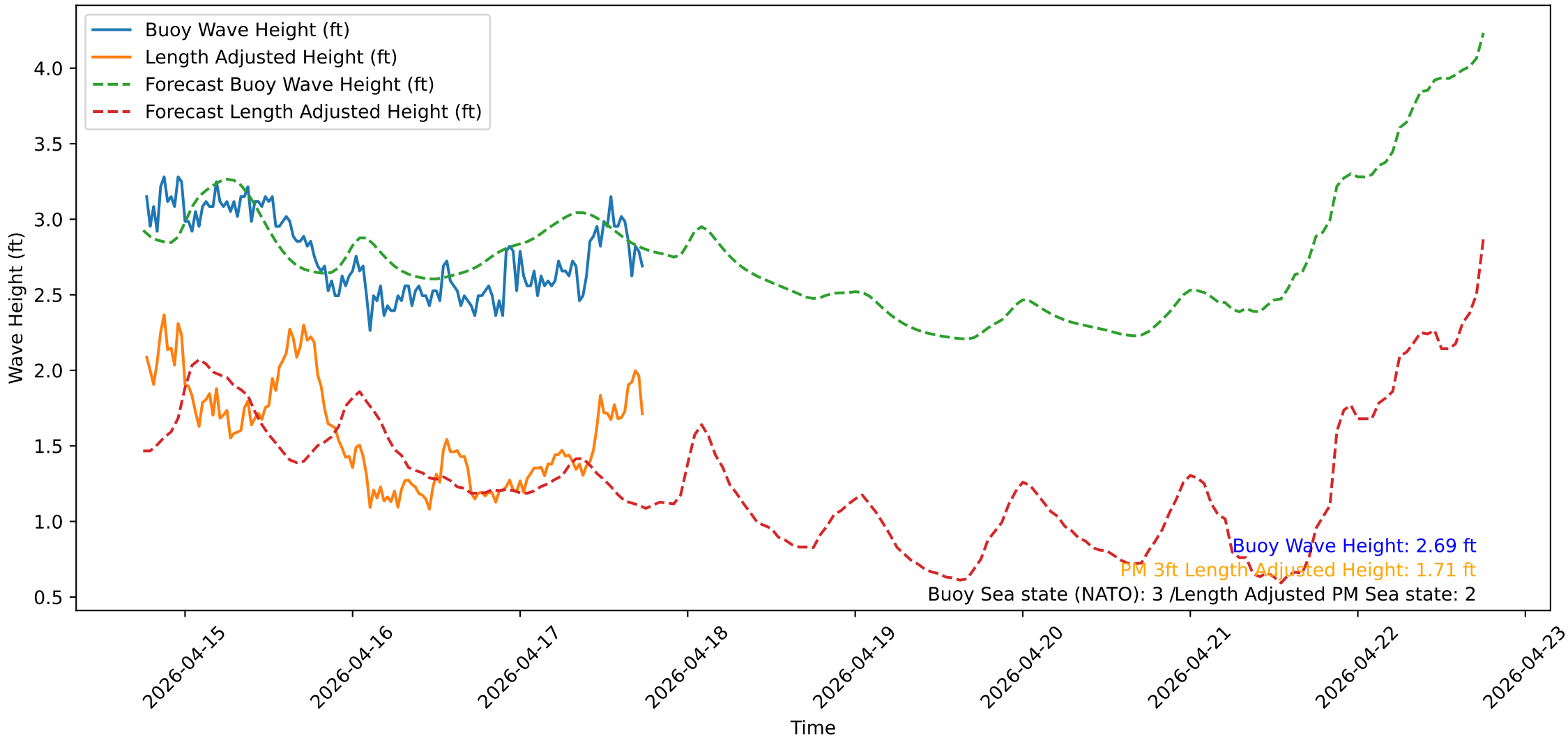
Wave Heights over Time for Red Beach at 2026-04-17 18:20:54
