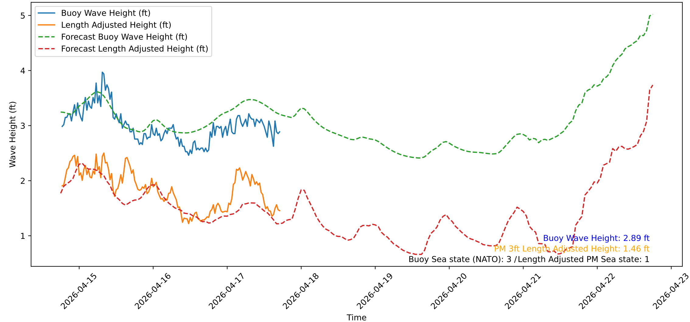
Wave Heights over Time for Green Beach at 2026-04-17 18:21:18
