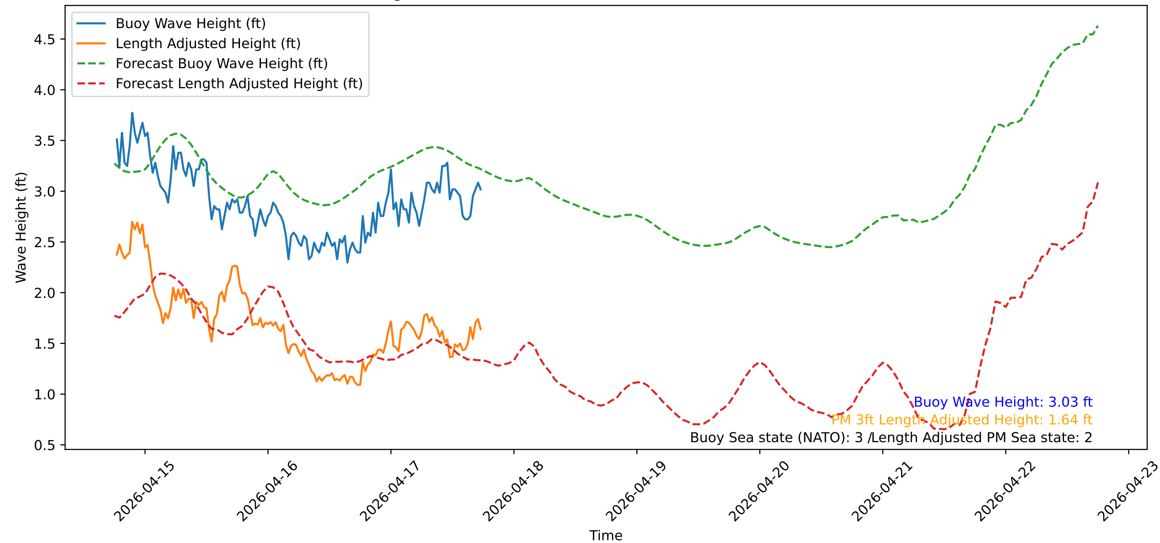
Wave Heights over Time for Oceanside Harbor at 2026-04-17 18:20:32
