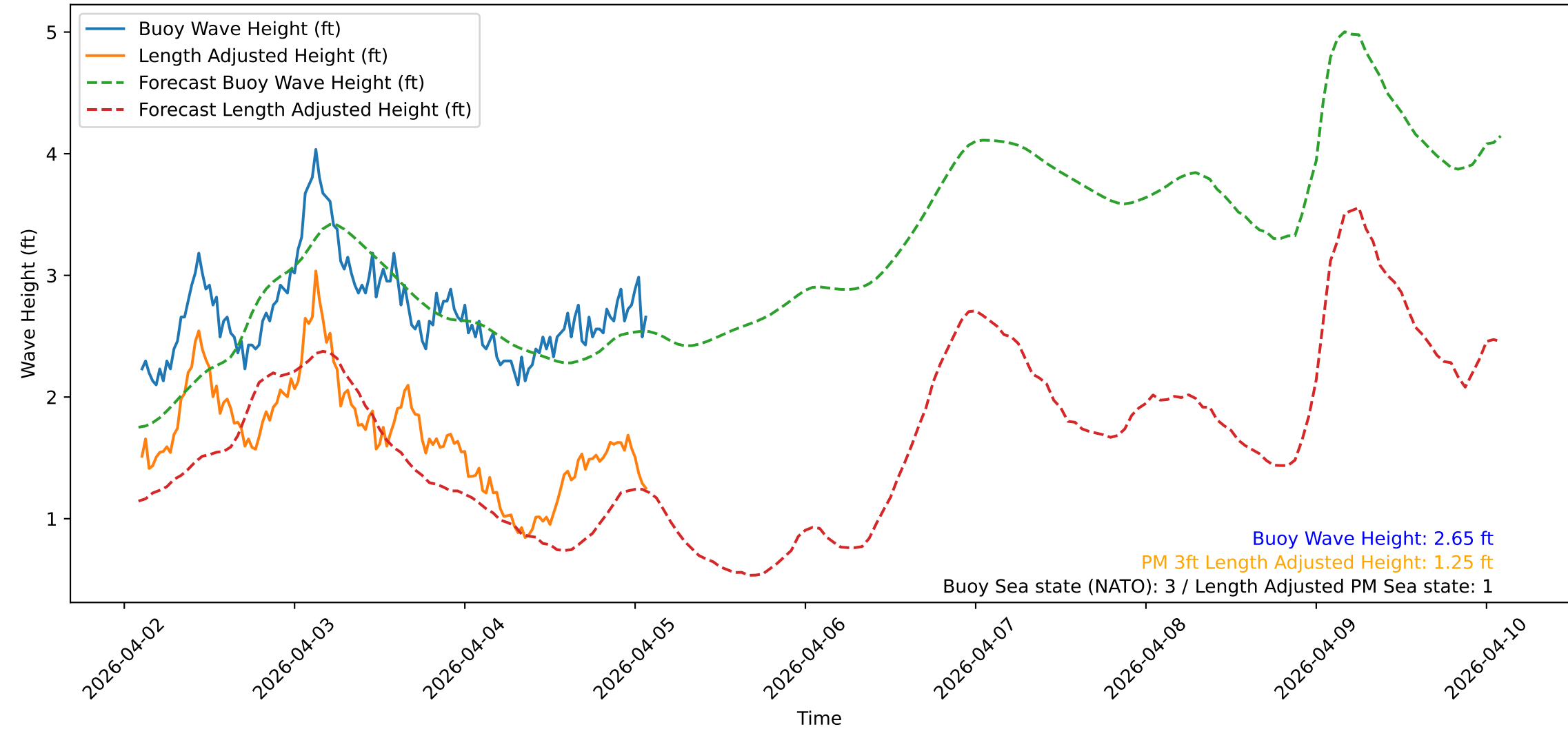
Wave Heights over Time for Oceanside Harbor at 2026-04-05 02:20:31
