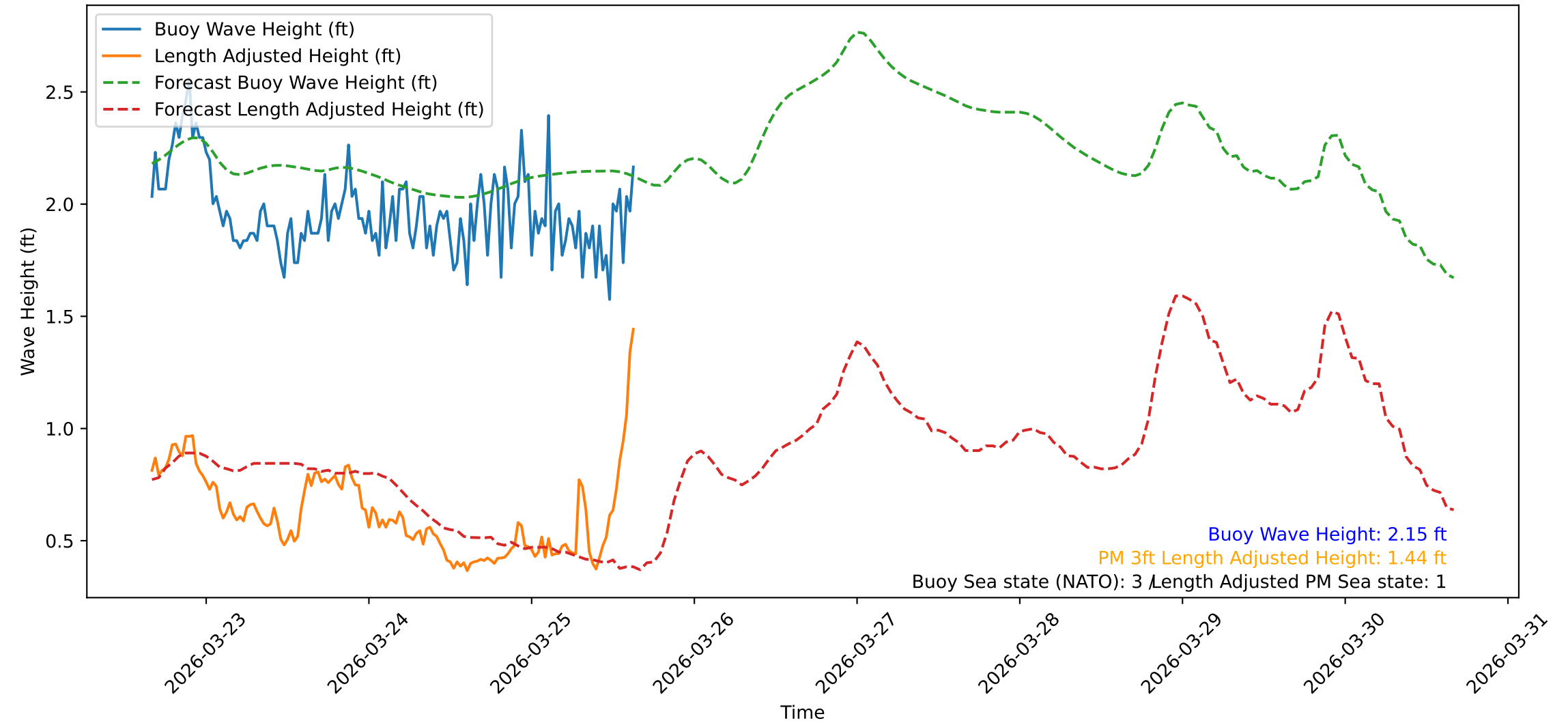
Wave Heights over Time for Red Beach at 2026-03-25 15:50:48
