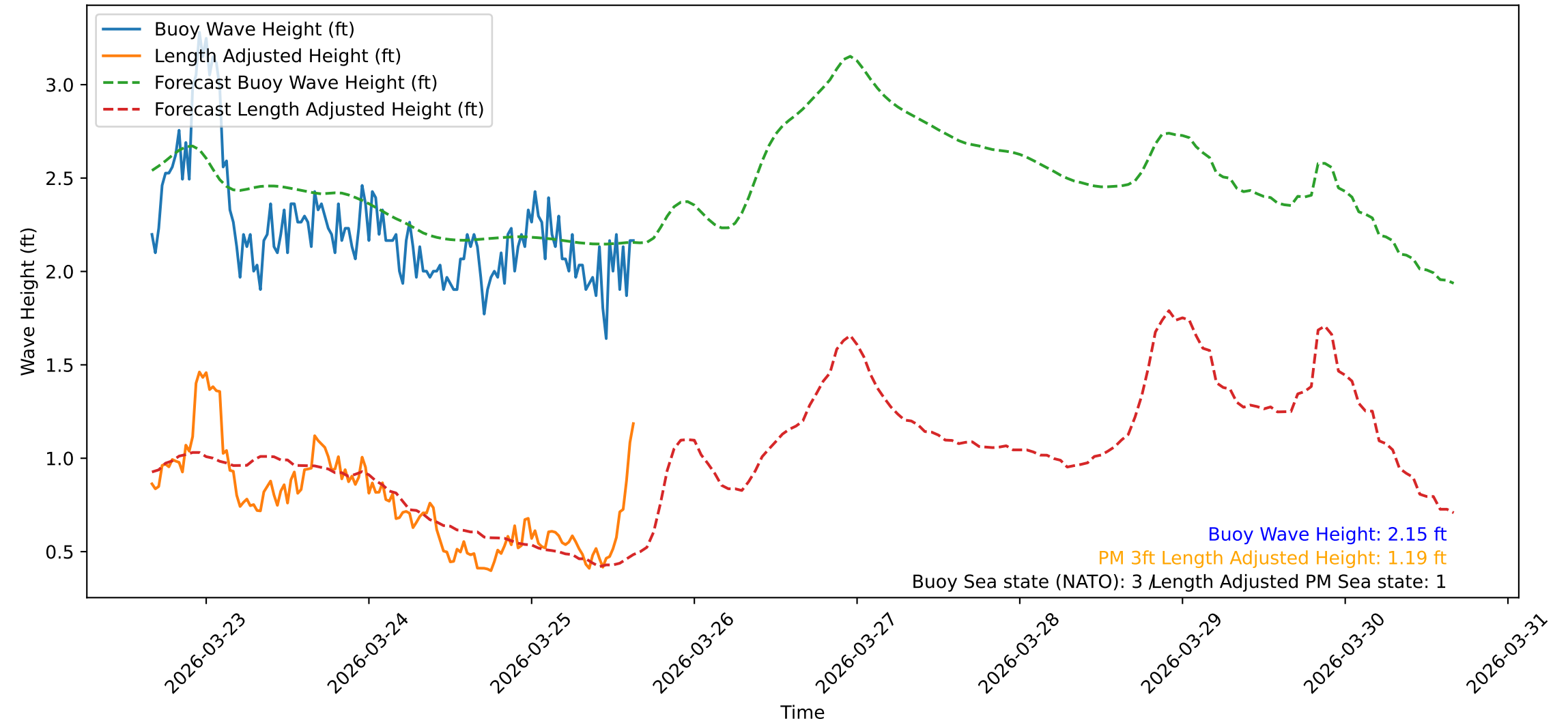
Wave Heights over Time for Green Beach at 2026-03-25 15:51:10
