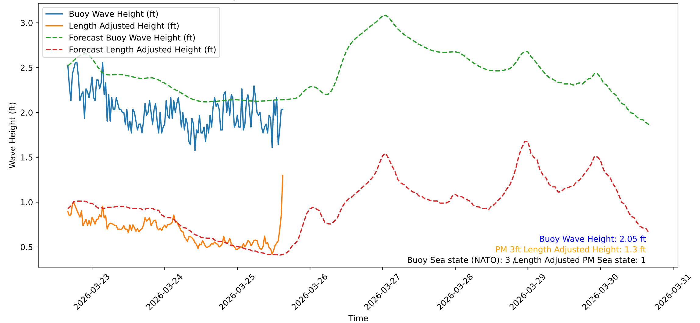
Wave Heights over Time for Oceanside Harbor at 2026-03-25 15:50:32
